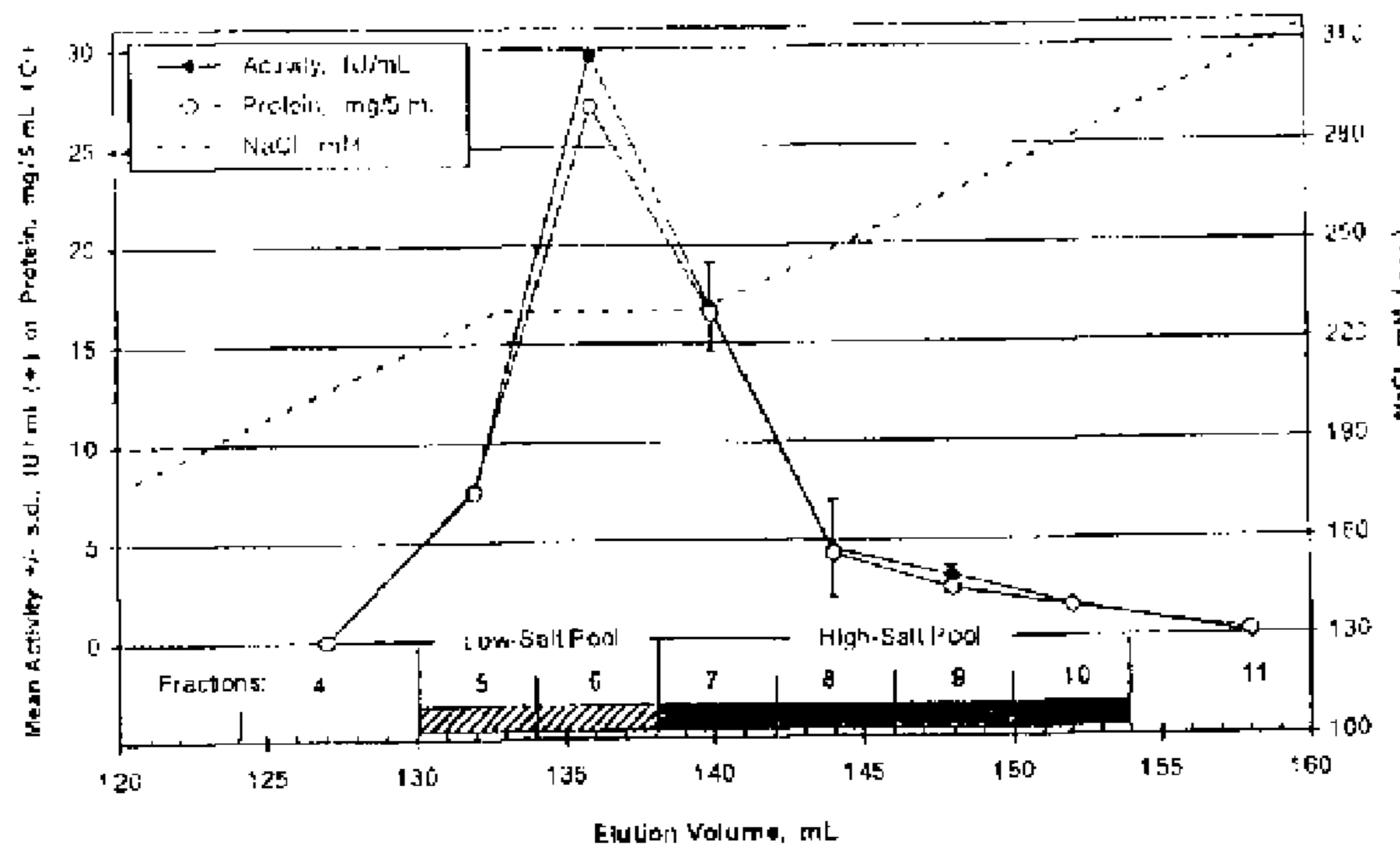
UV Assay of Uricolytic Activity in Fractions from Mono Q Chromatography of PK5 Uricase (Protein Based on Size Exclusion HPLC)
