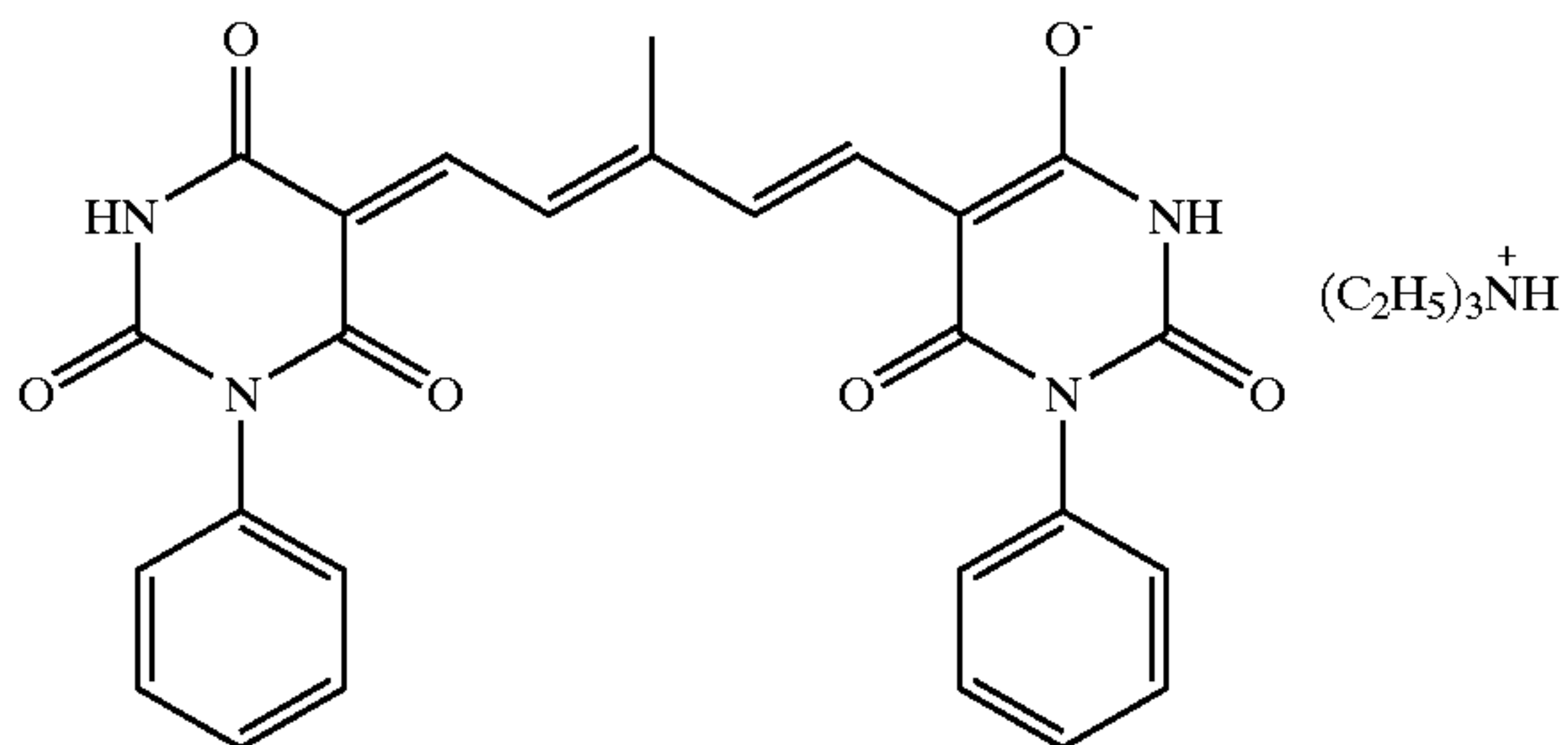
Dye "A"
