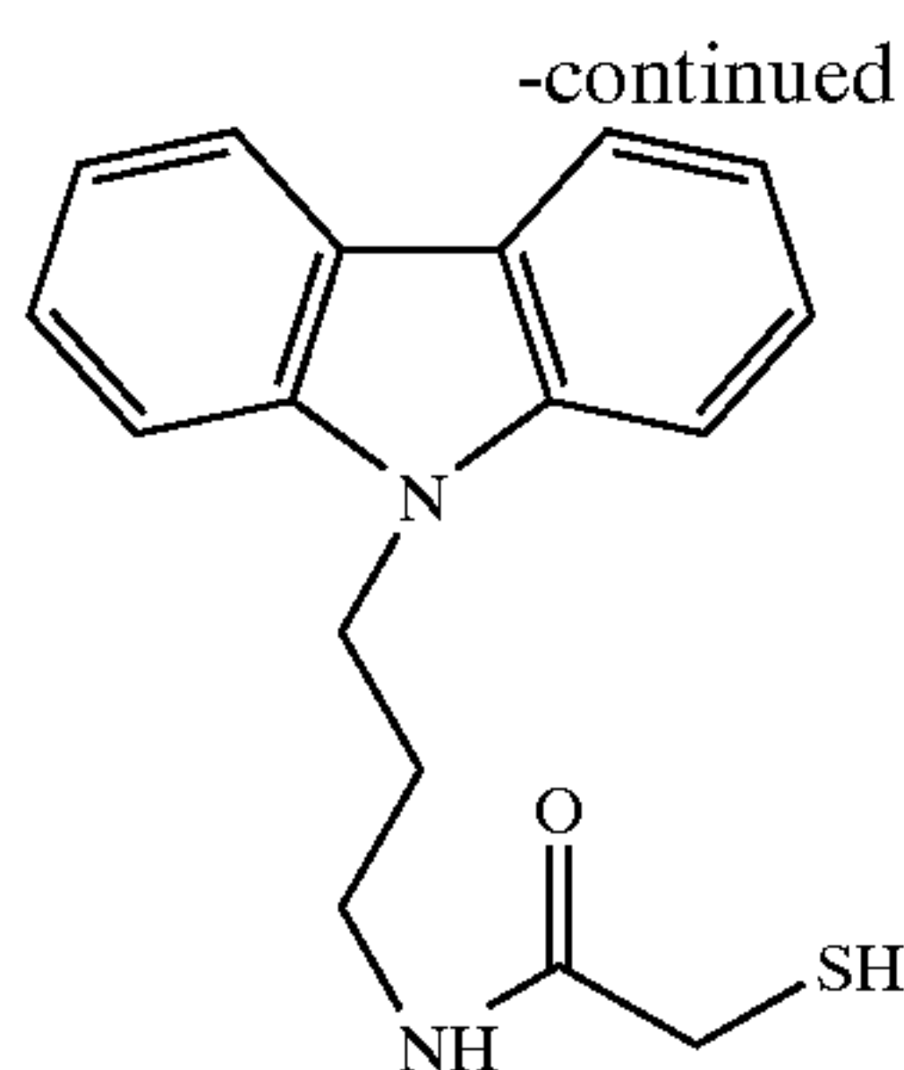
Compound "B"
