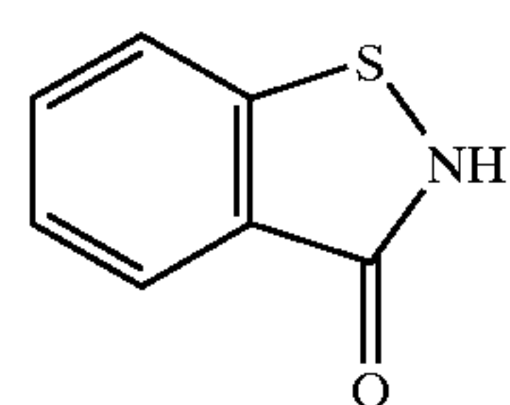
Compound "A"
