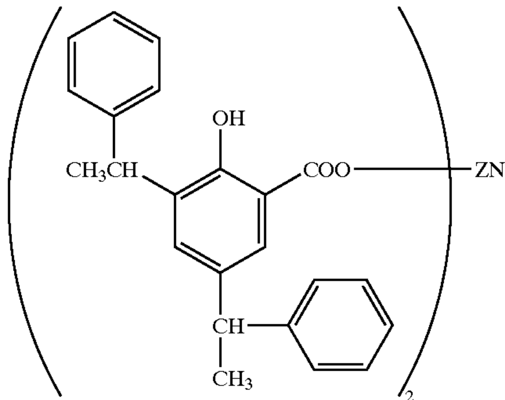
Compound "Z"
