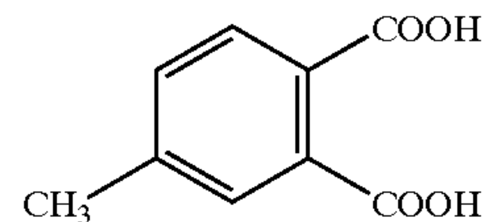
Compound "F"
