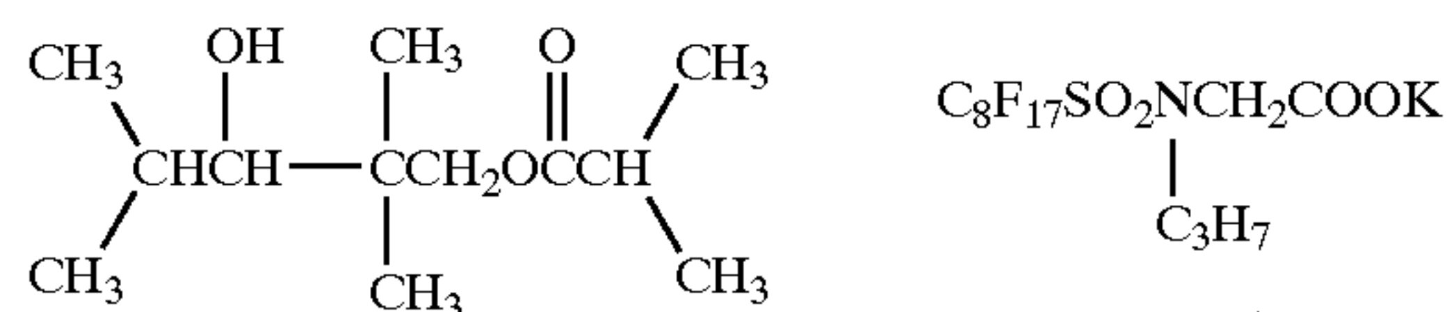
Compound "E"
