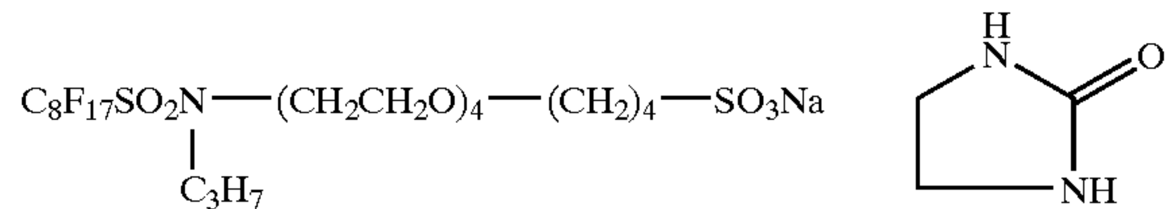
Compound "H"
