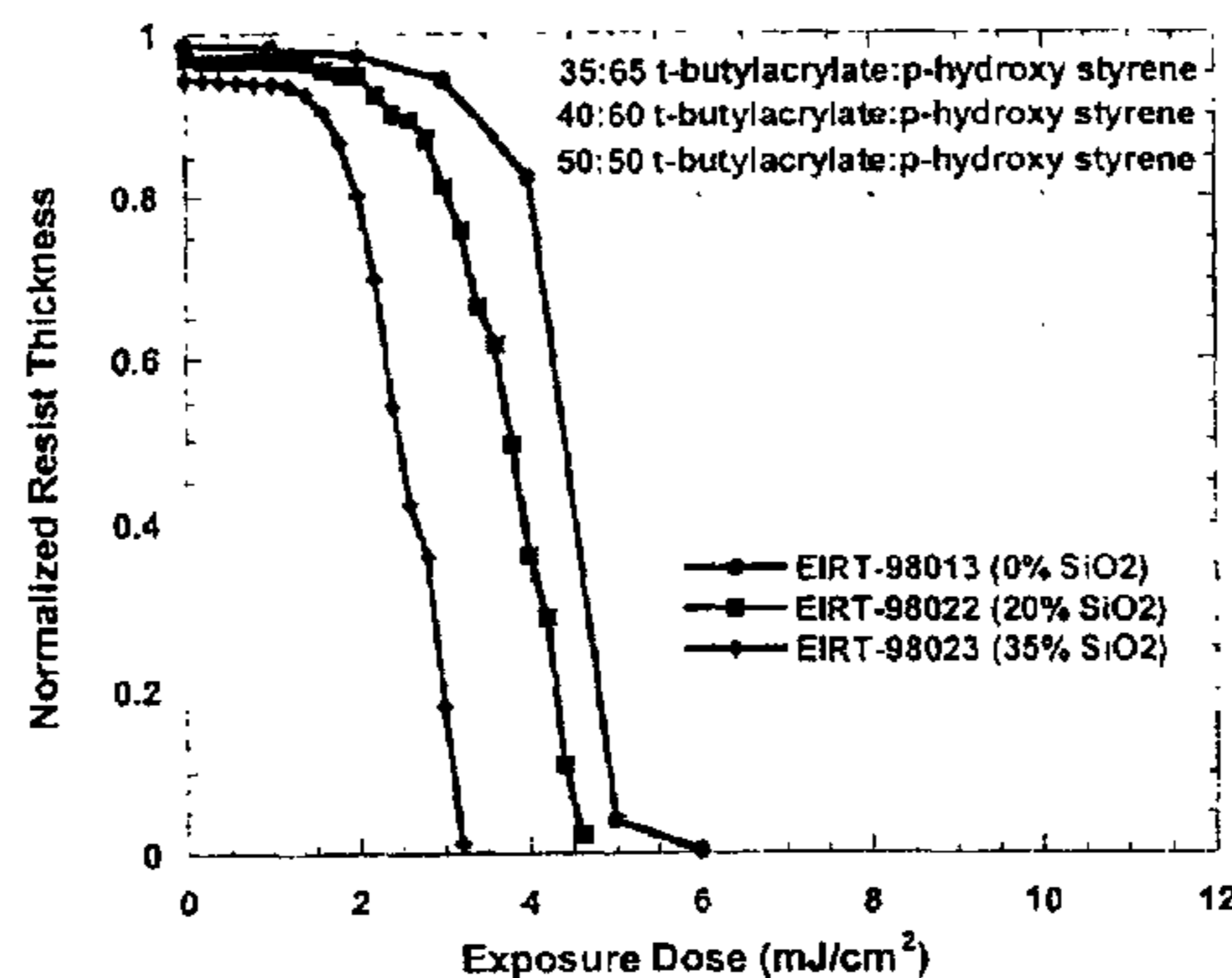
Comparison of contrast curves of three EIRT resists of improved formulation.
