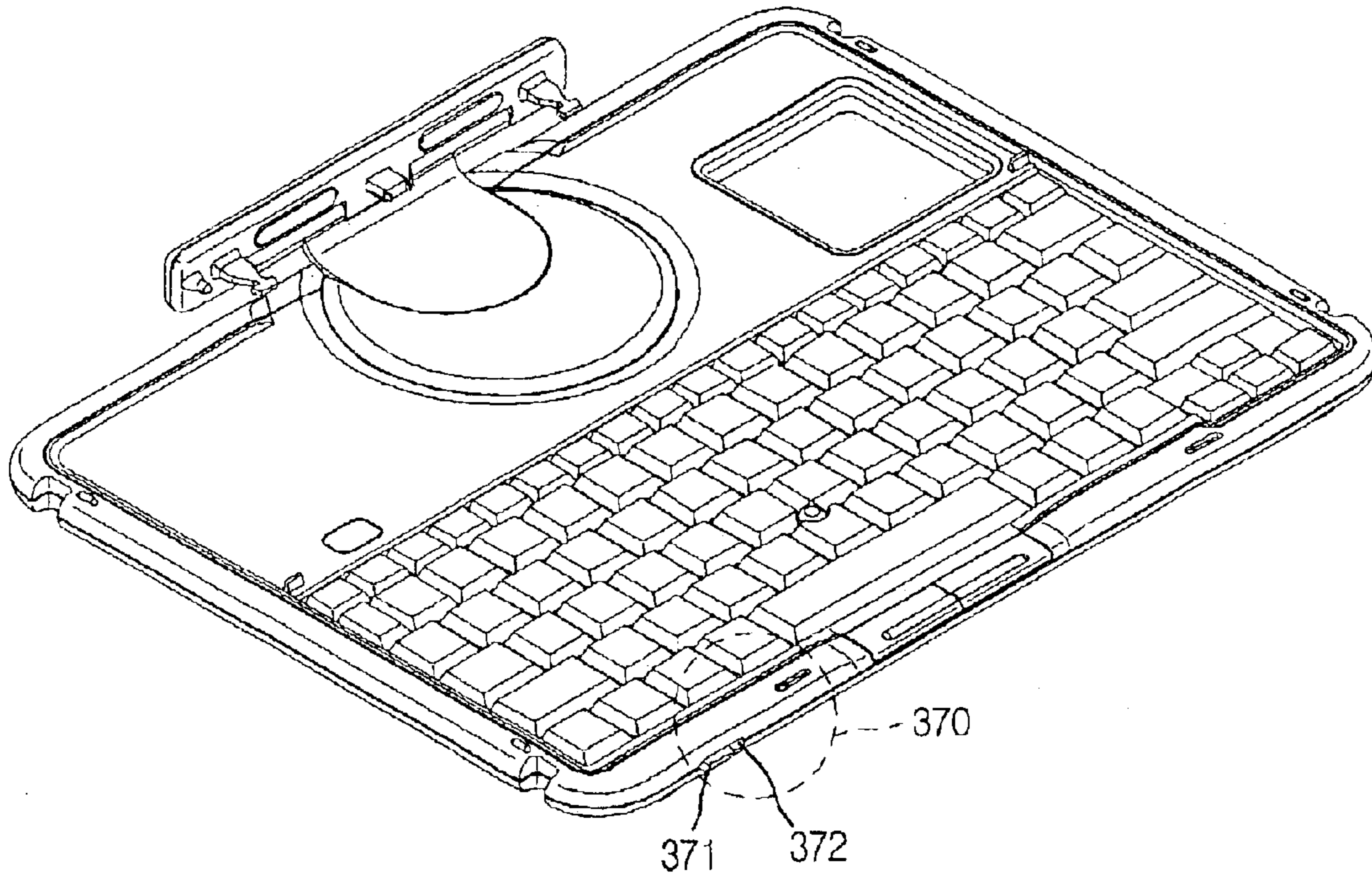
(Before being connected to main body)
