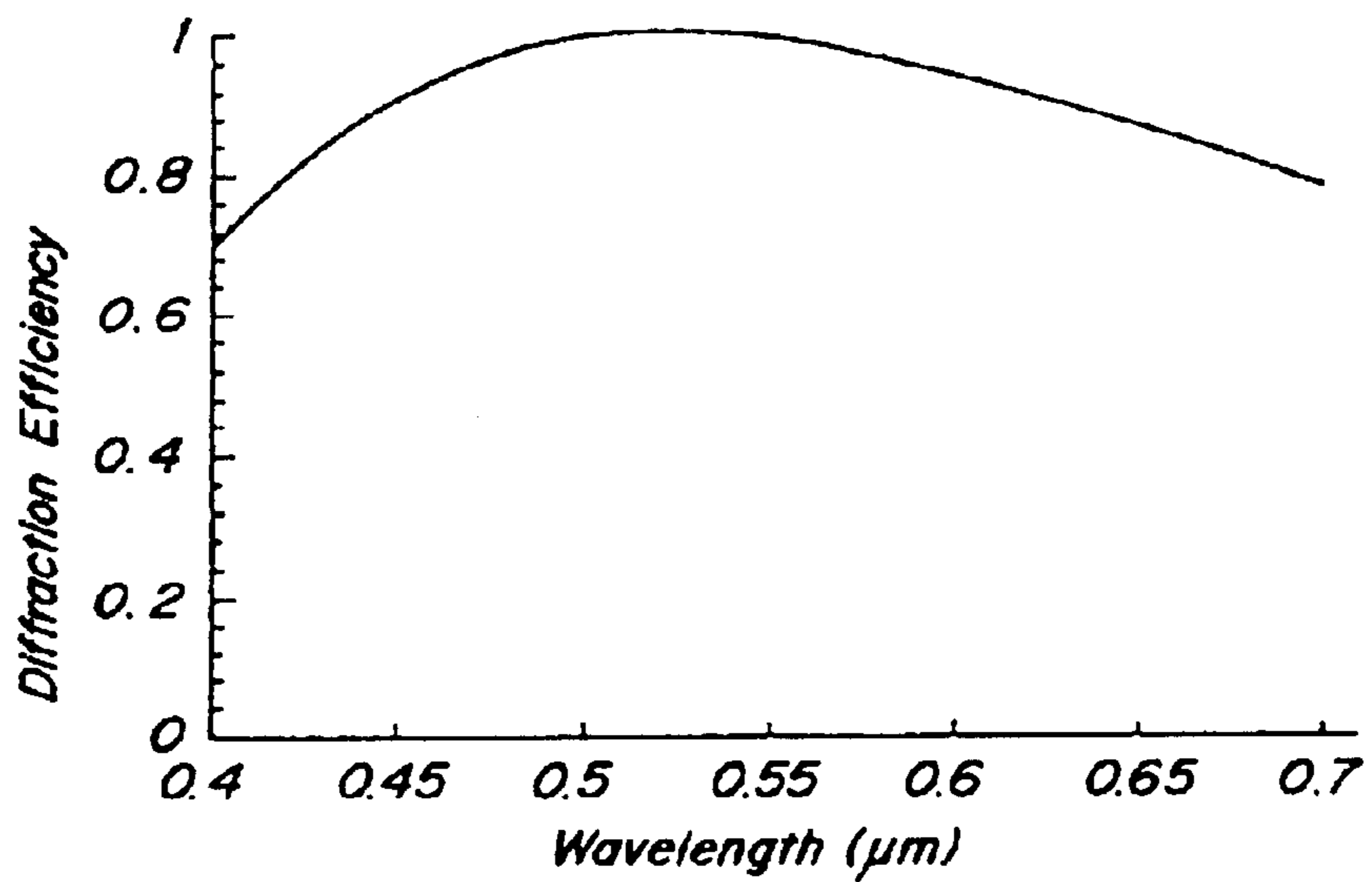
FIG. 2 PRIOR ART
