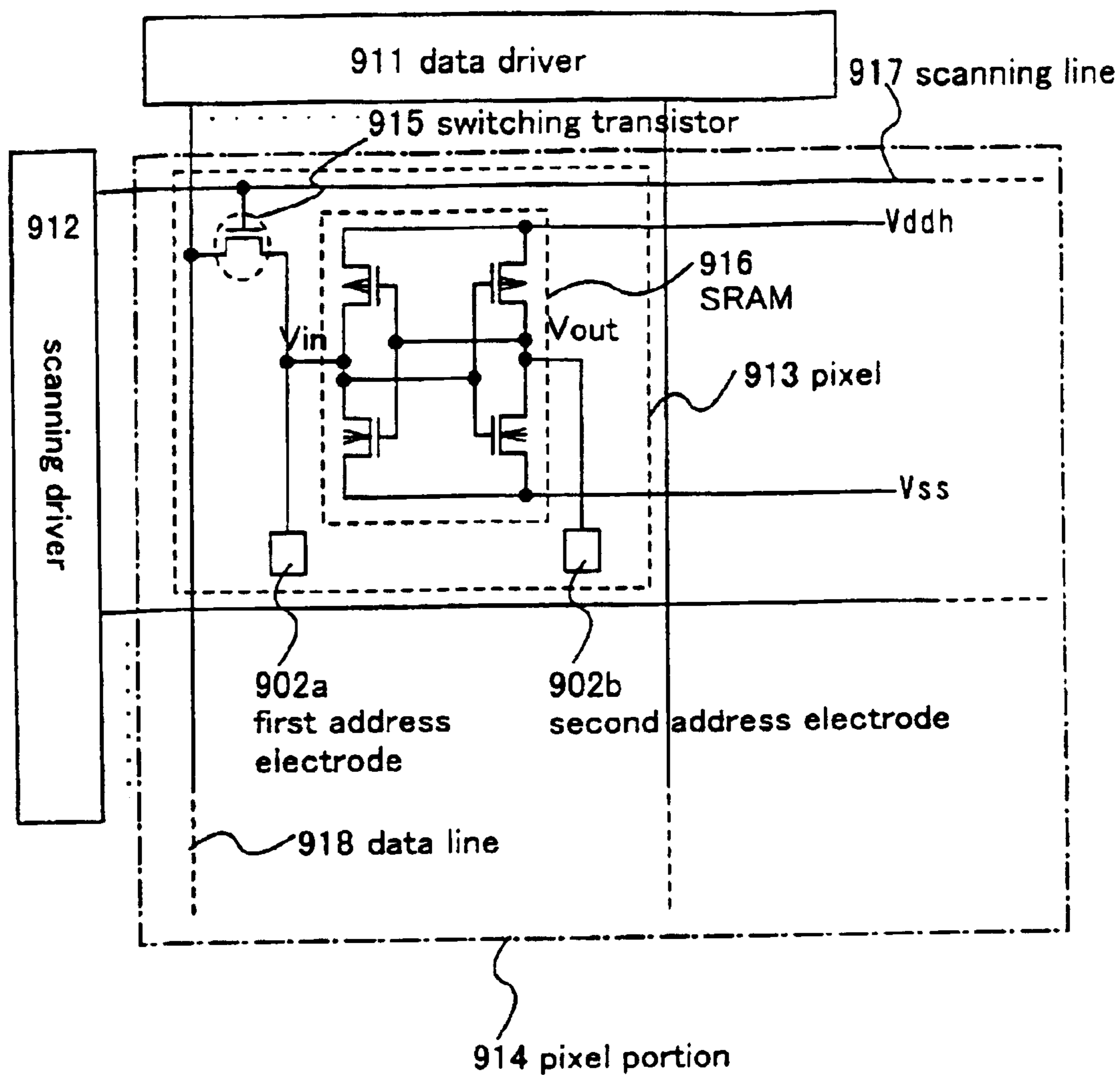
Fig. 21 (PRIOR ART)
