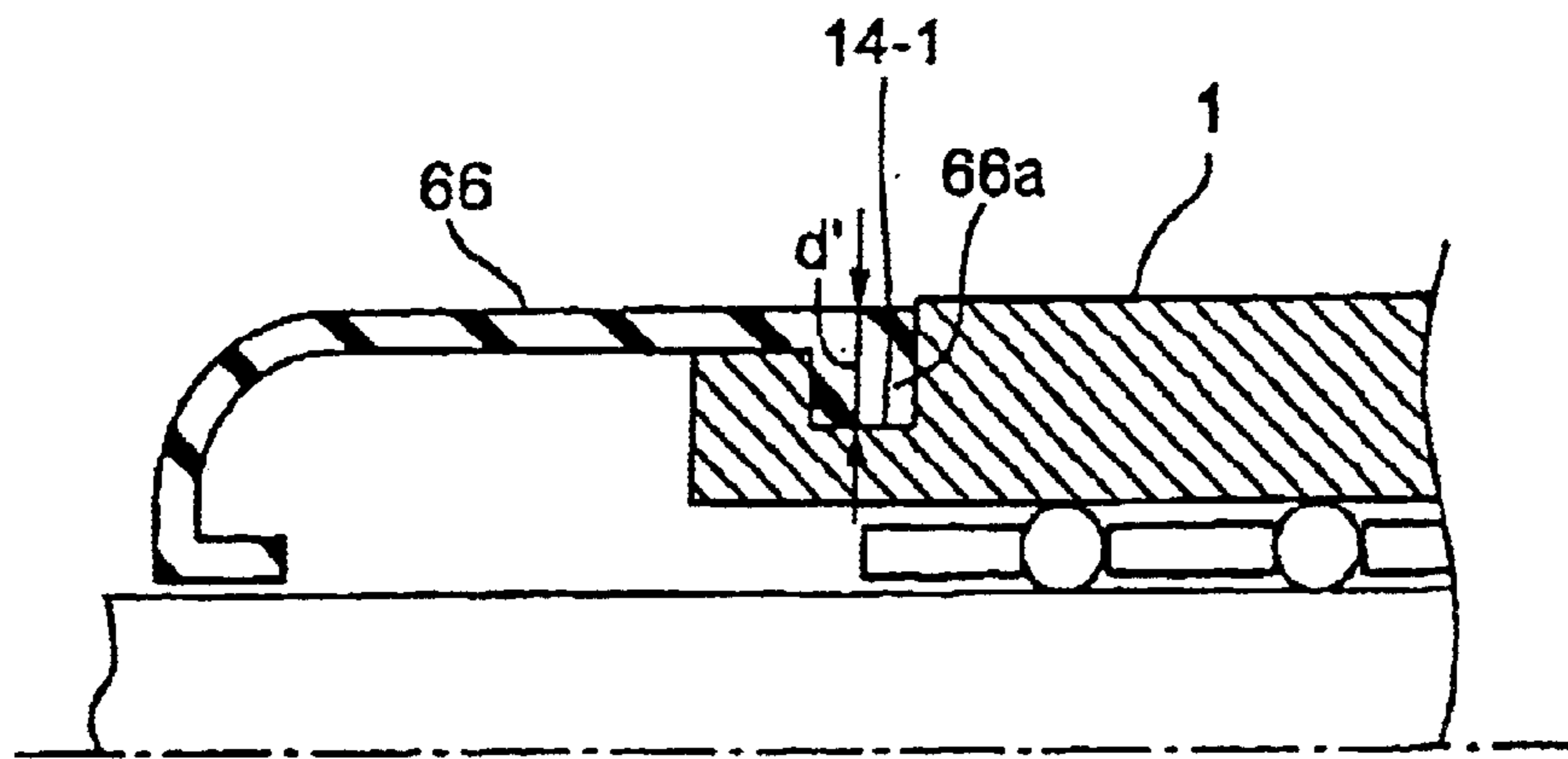
FIG. 21 (PRIOR ART)
