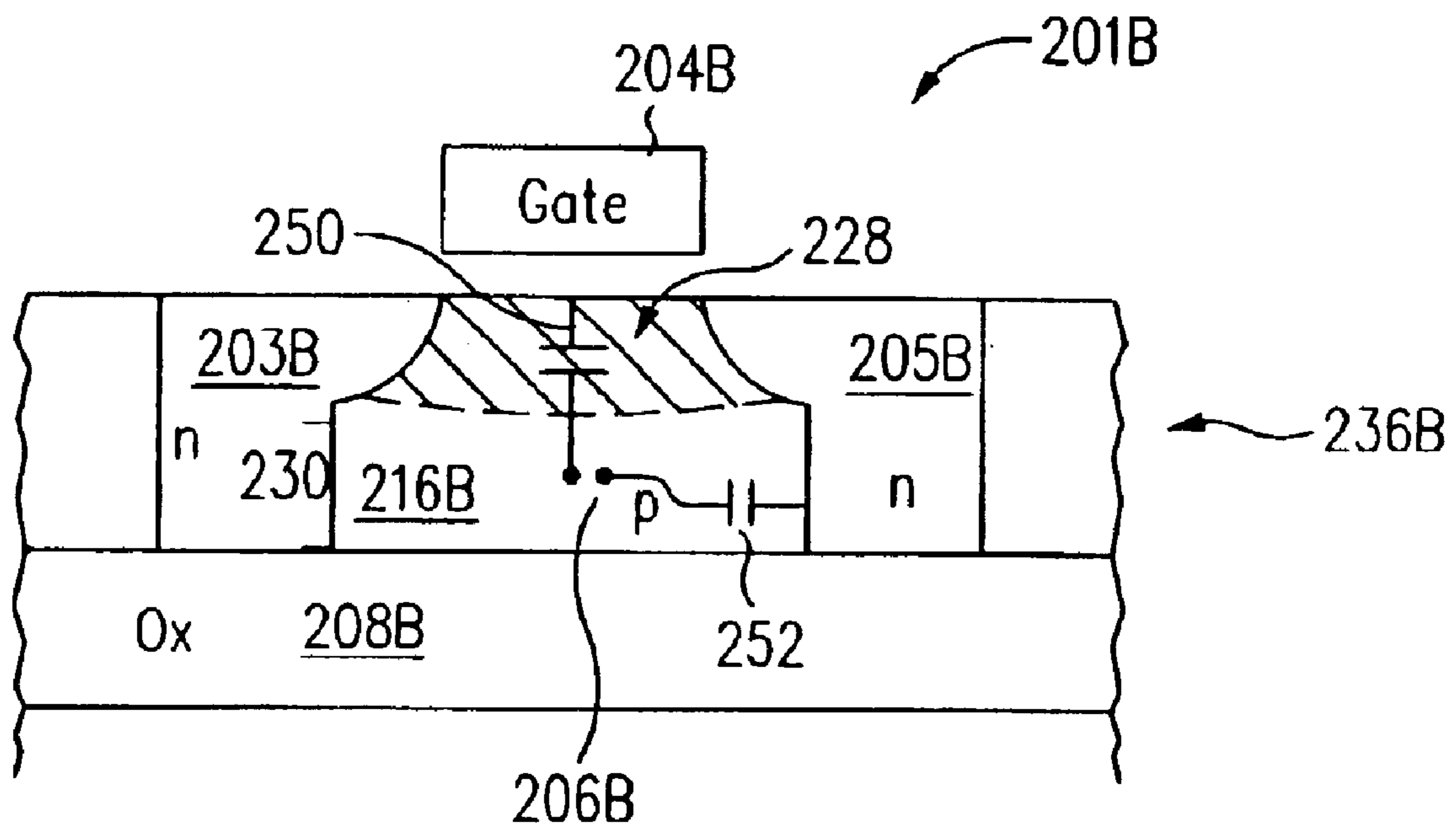
FIG. 2C (PRIOR ART)
