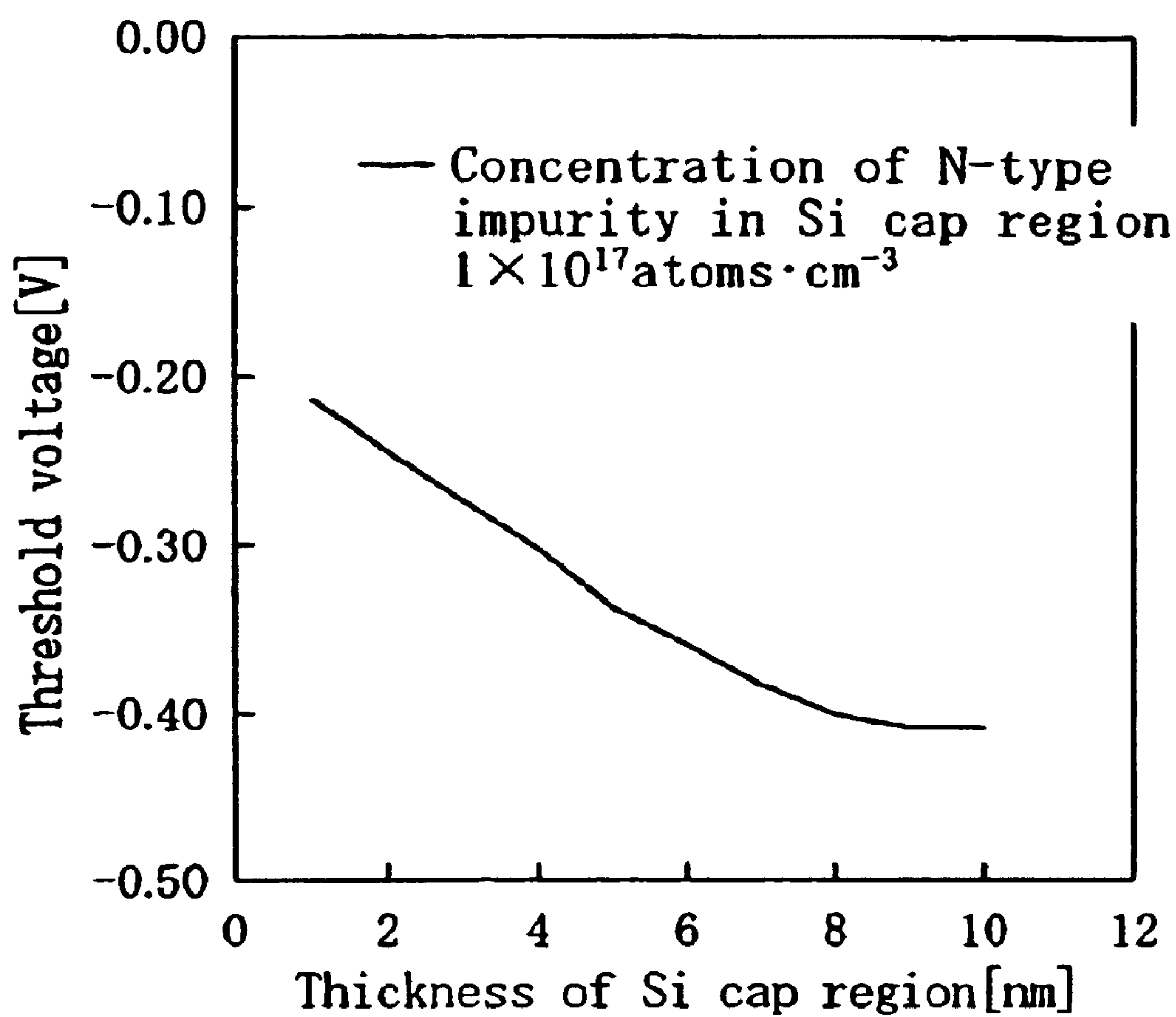
FIG. 16 (Prior Art)
