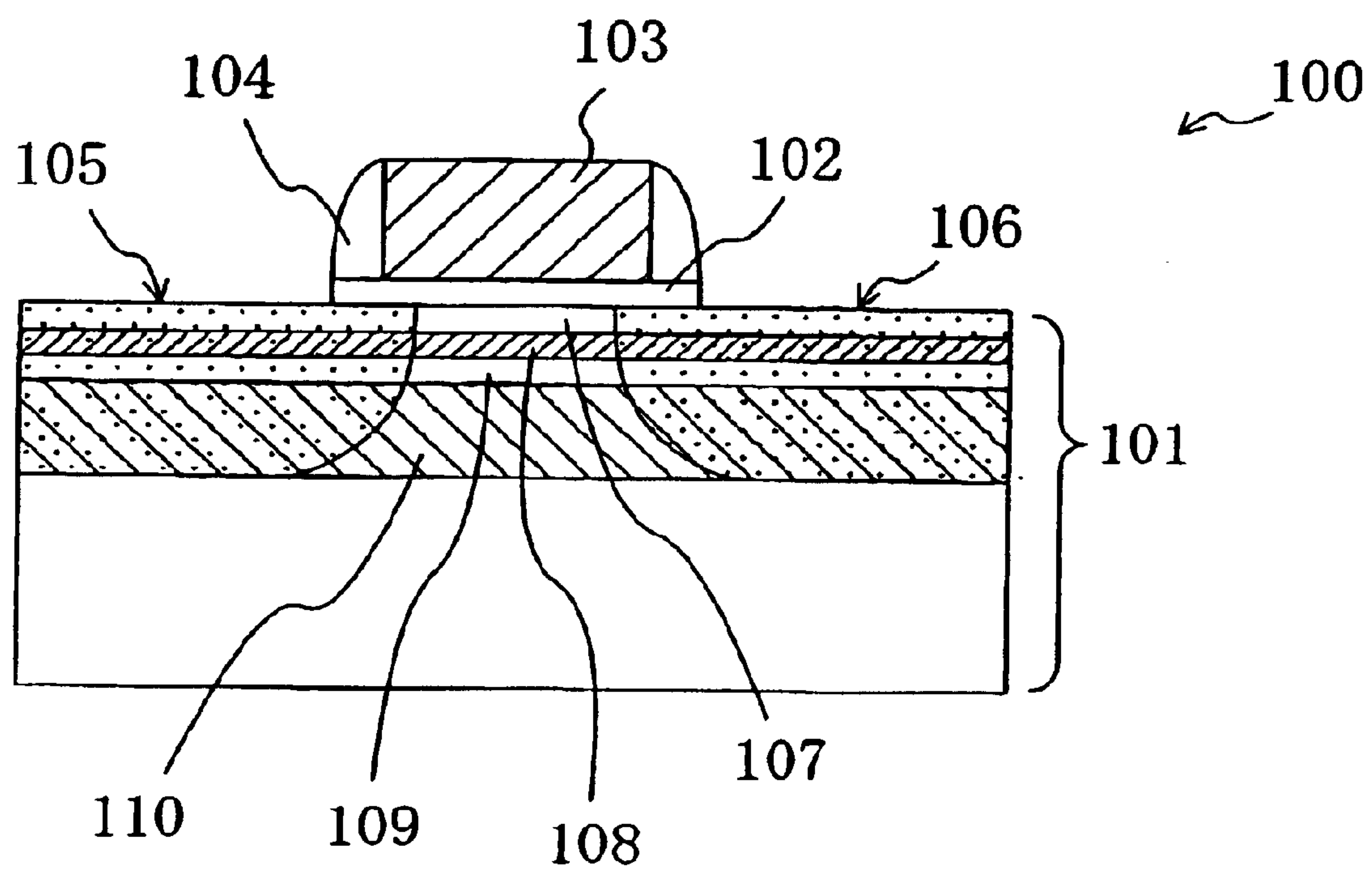
FIG. 15 (Prior Art)
