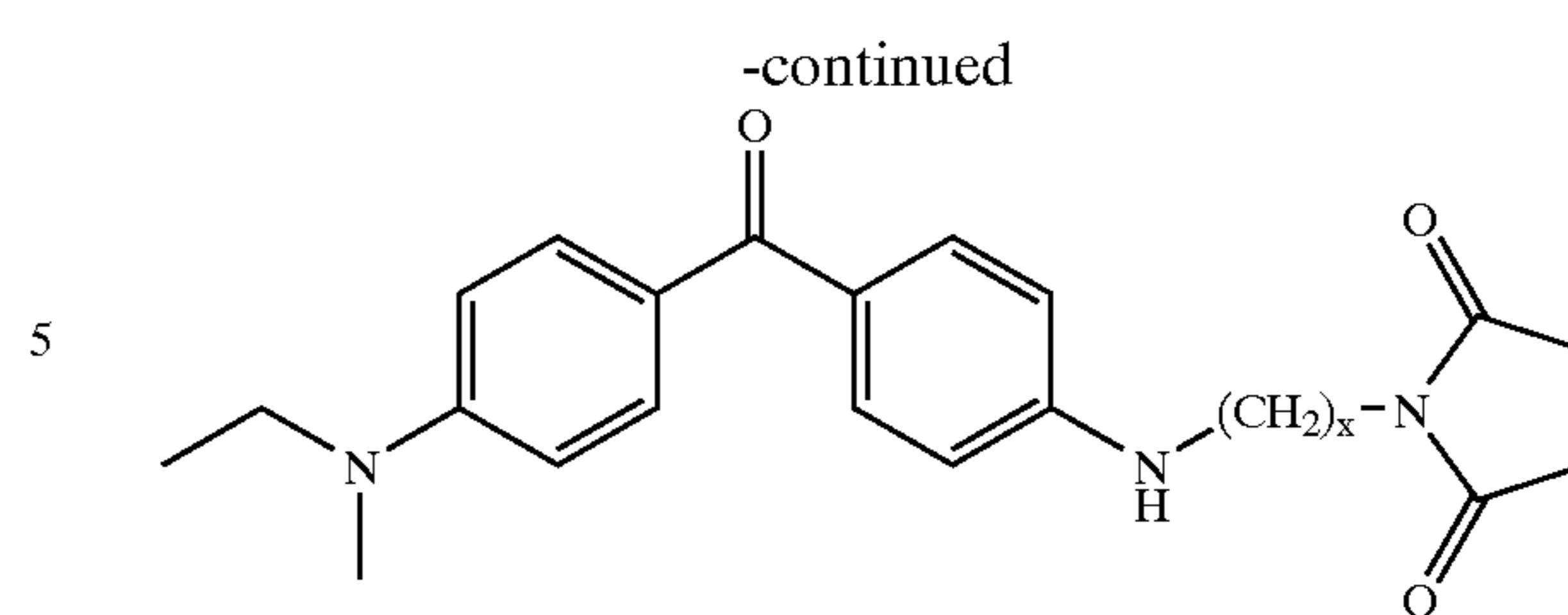
4(methylethylamino)-4'-(aliphatic maleimideamino)benzophenone
