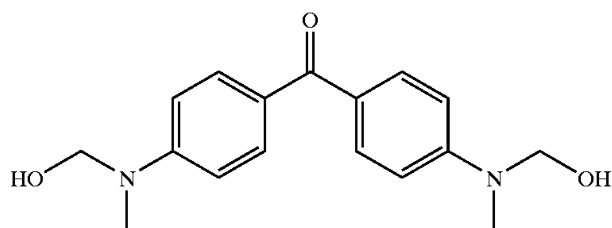
4-(diethylamino)-4'-(methylethylamino)benzophenone
