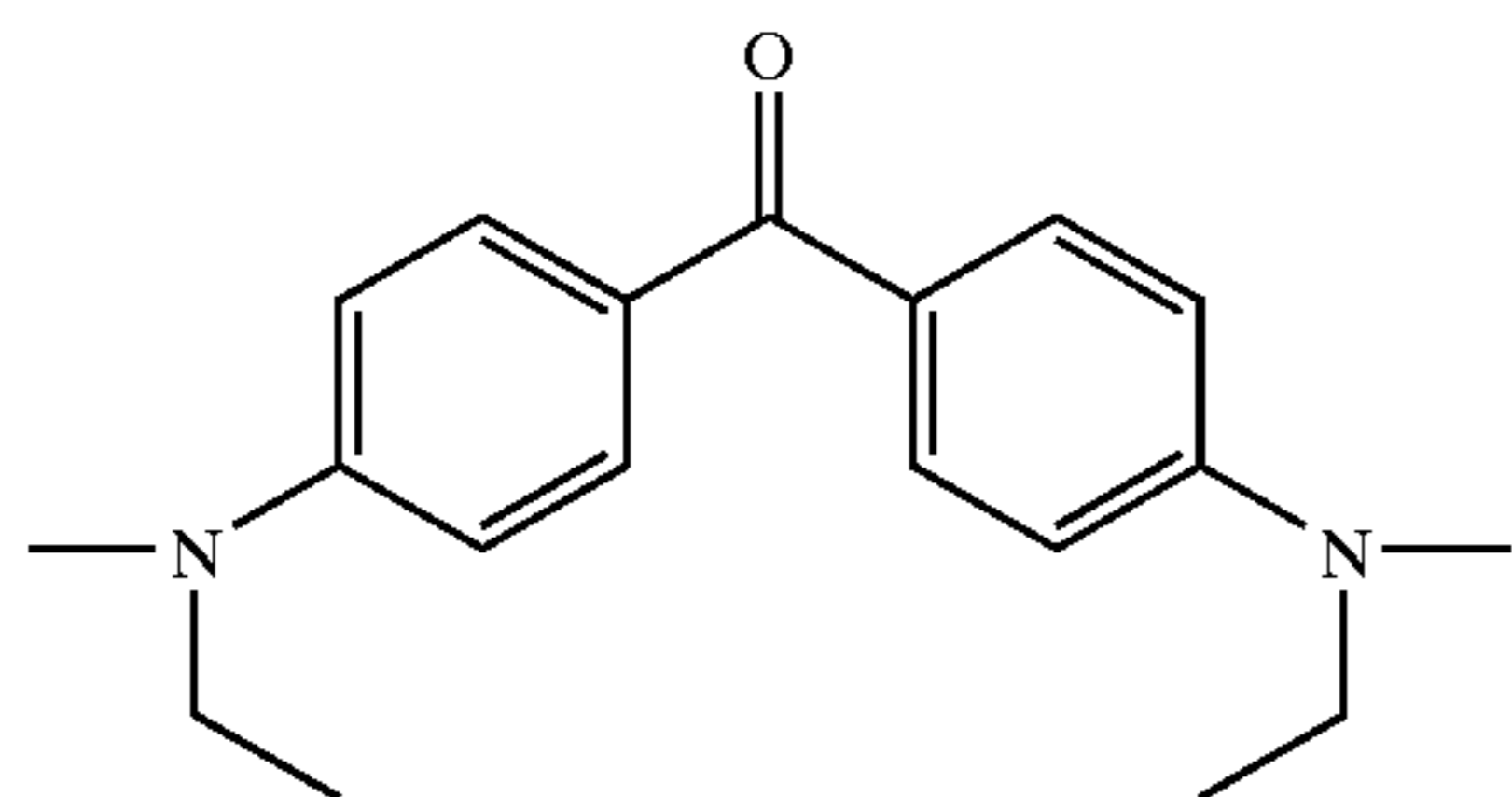
4,4'-bis(methylethylamino)benzophenone
