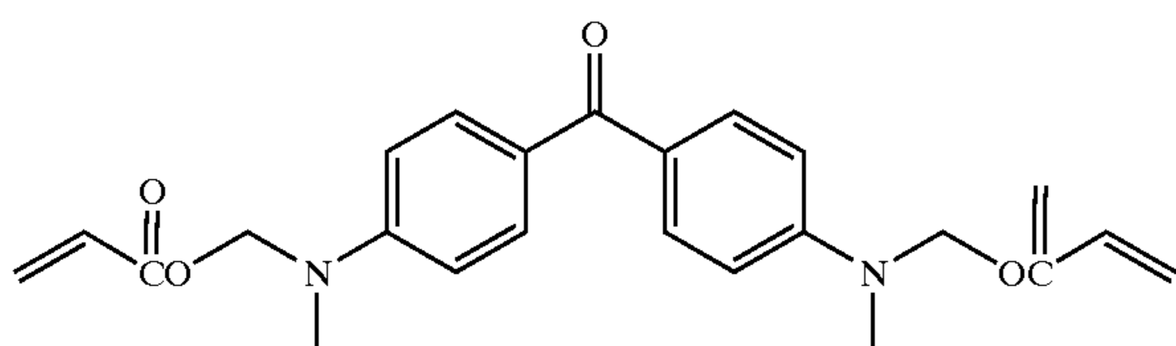
4,4'-bis(methylethanolamino)benzophenone
