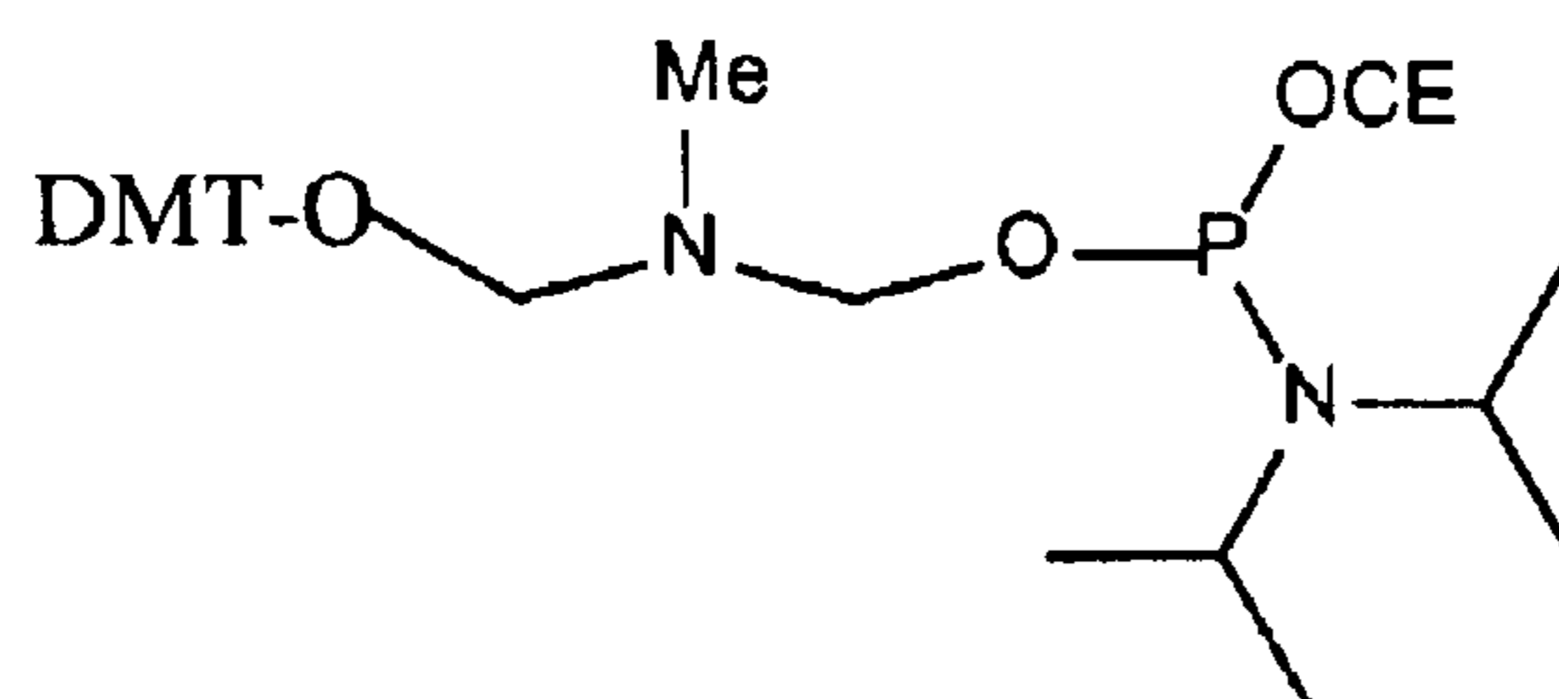
Neutral Phosphoramidite
