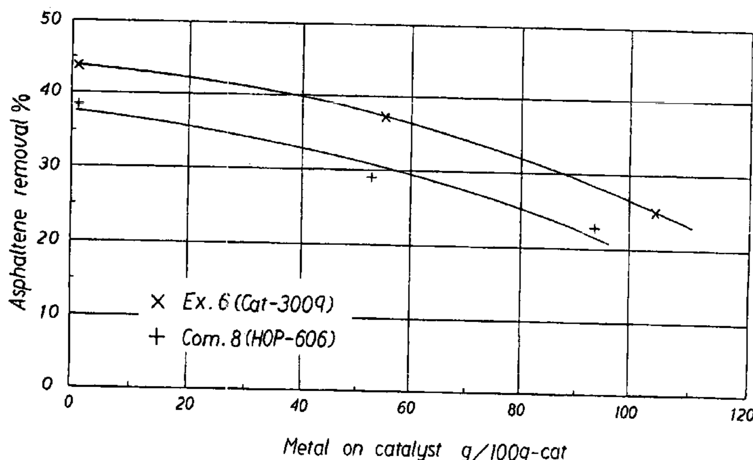
Aging tests with Ratawi AR & VR mixture
