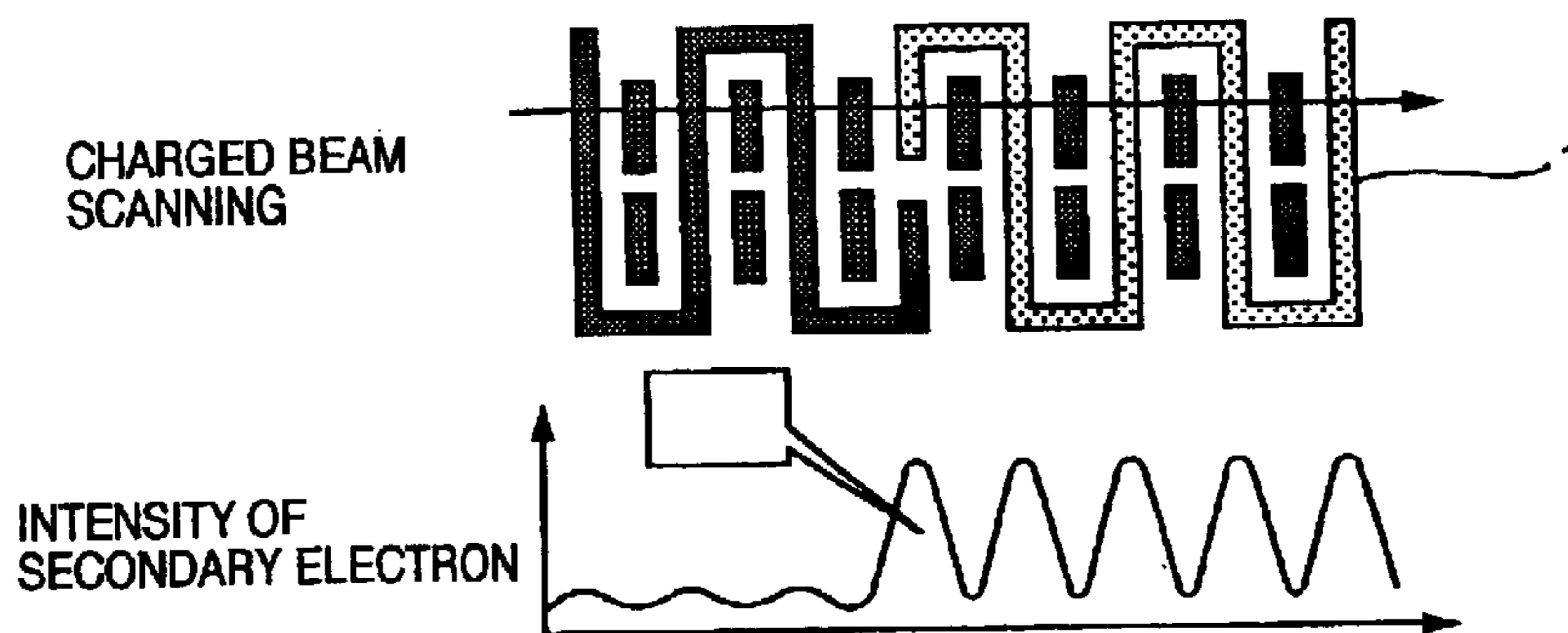
(A) LINE SCANNING SIGNAL PROCESSING SYSTEM
