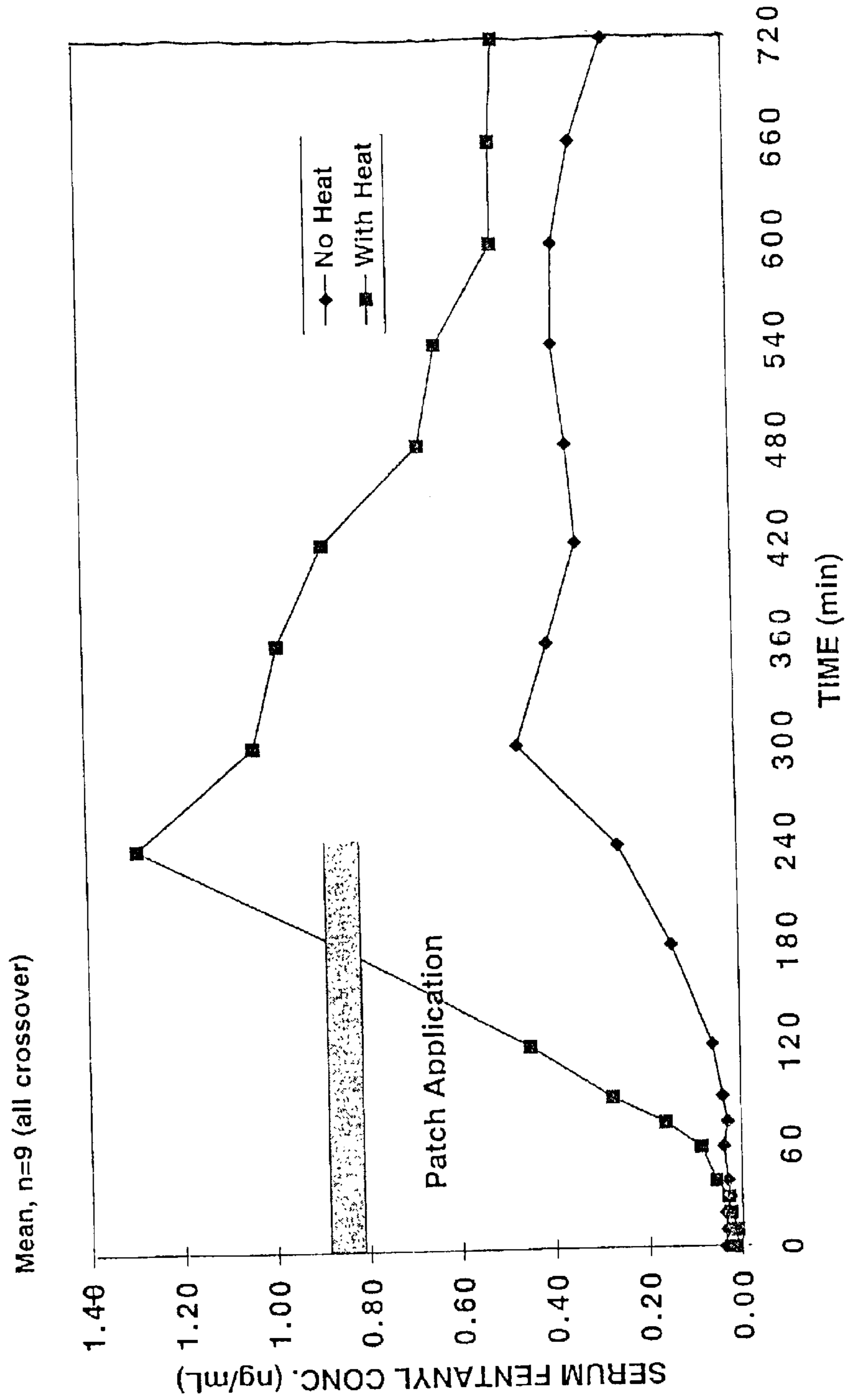
Serum Fentanyl Levels From 50 µg Patch: Effect of Heat
