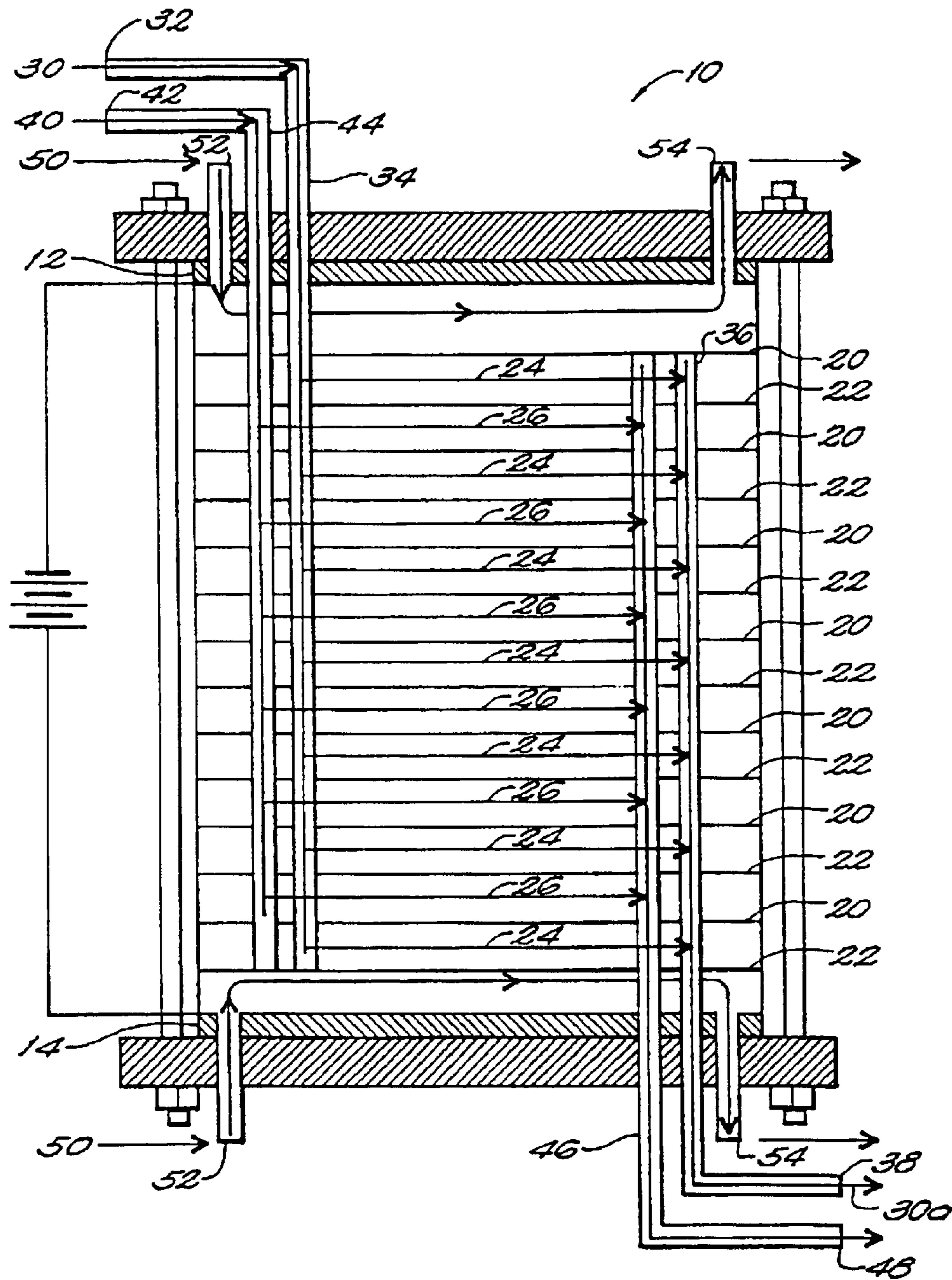
FIG. 1 (PRIOR ART)
