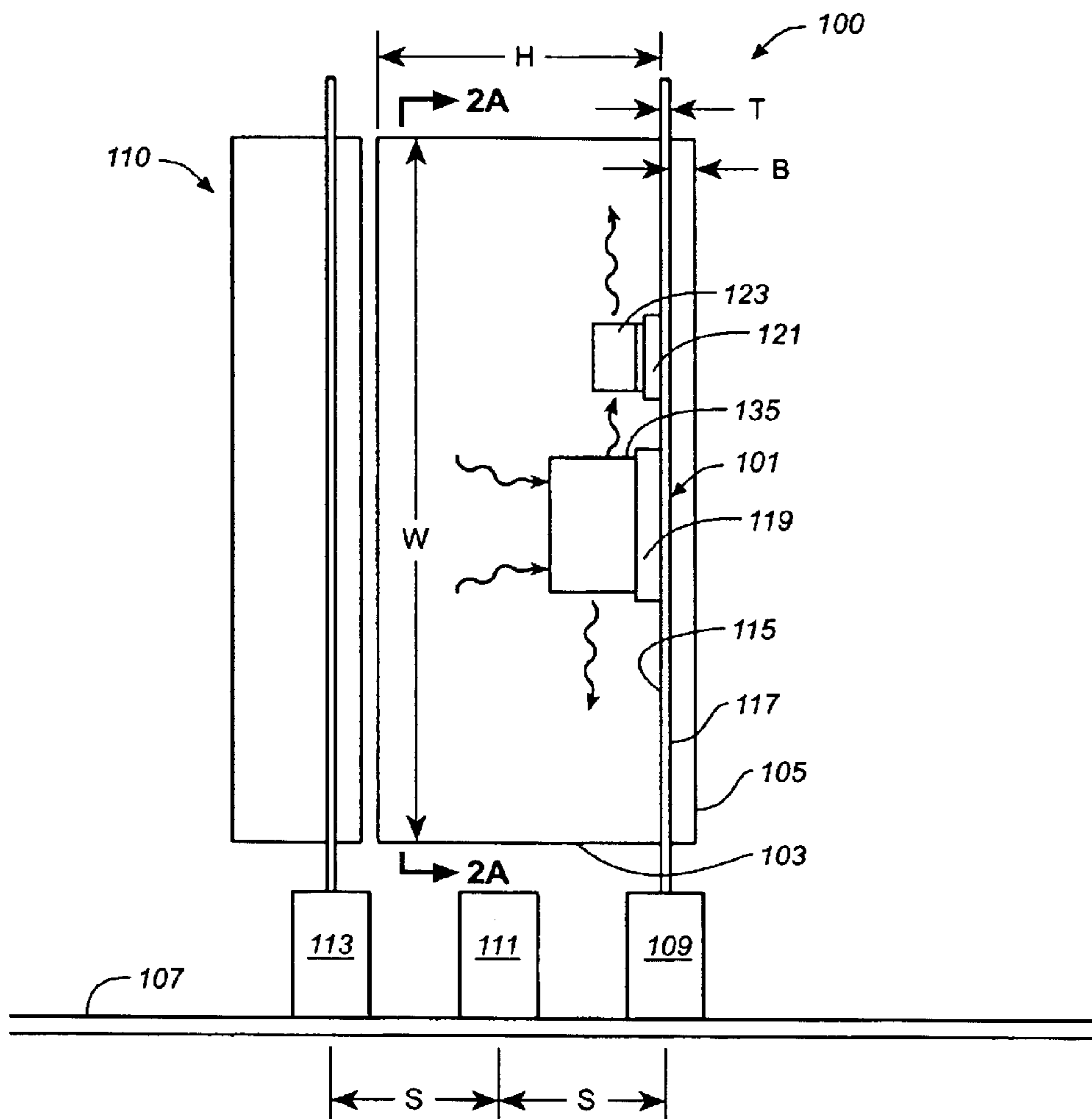
FIG. 1 (PRIOR ART)
