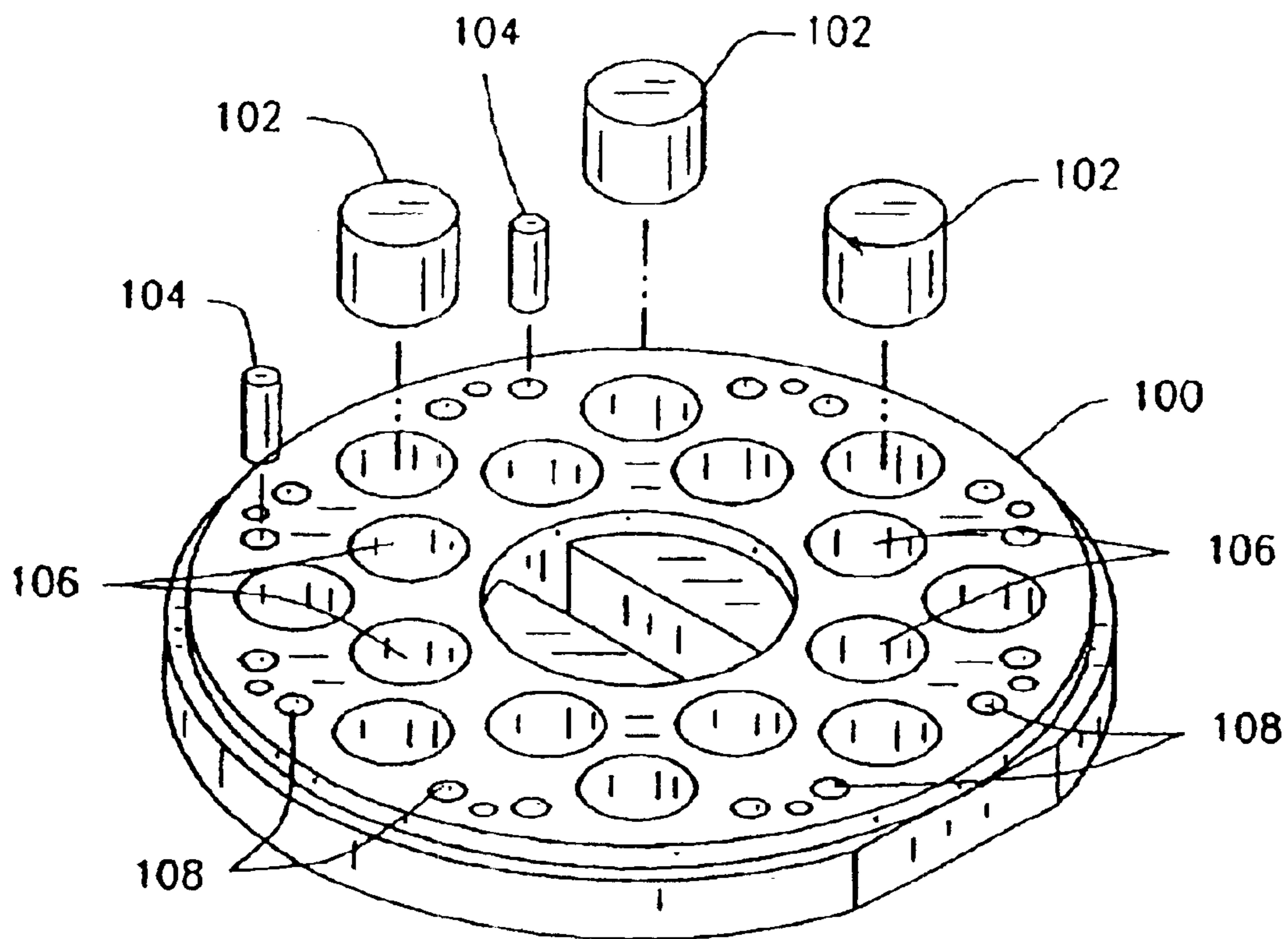
FIG. 1 PRIOR ART
