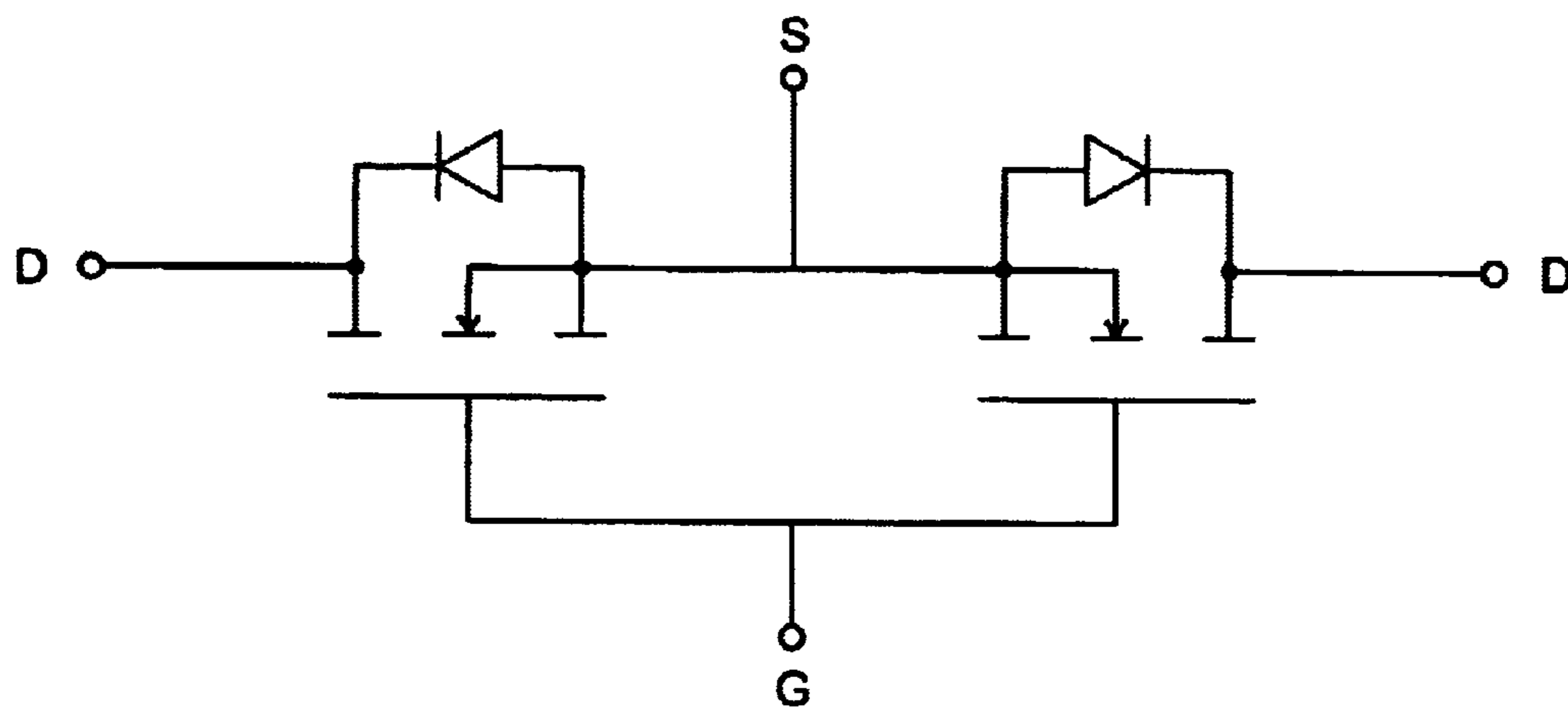
FIG. 5 (PRIOR ART)
