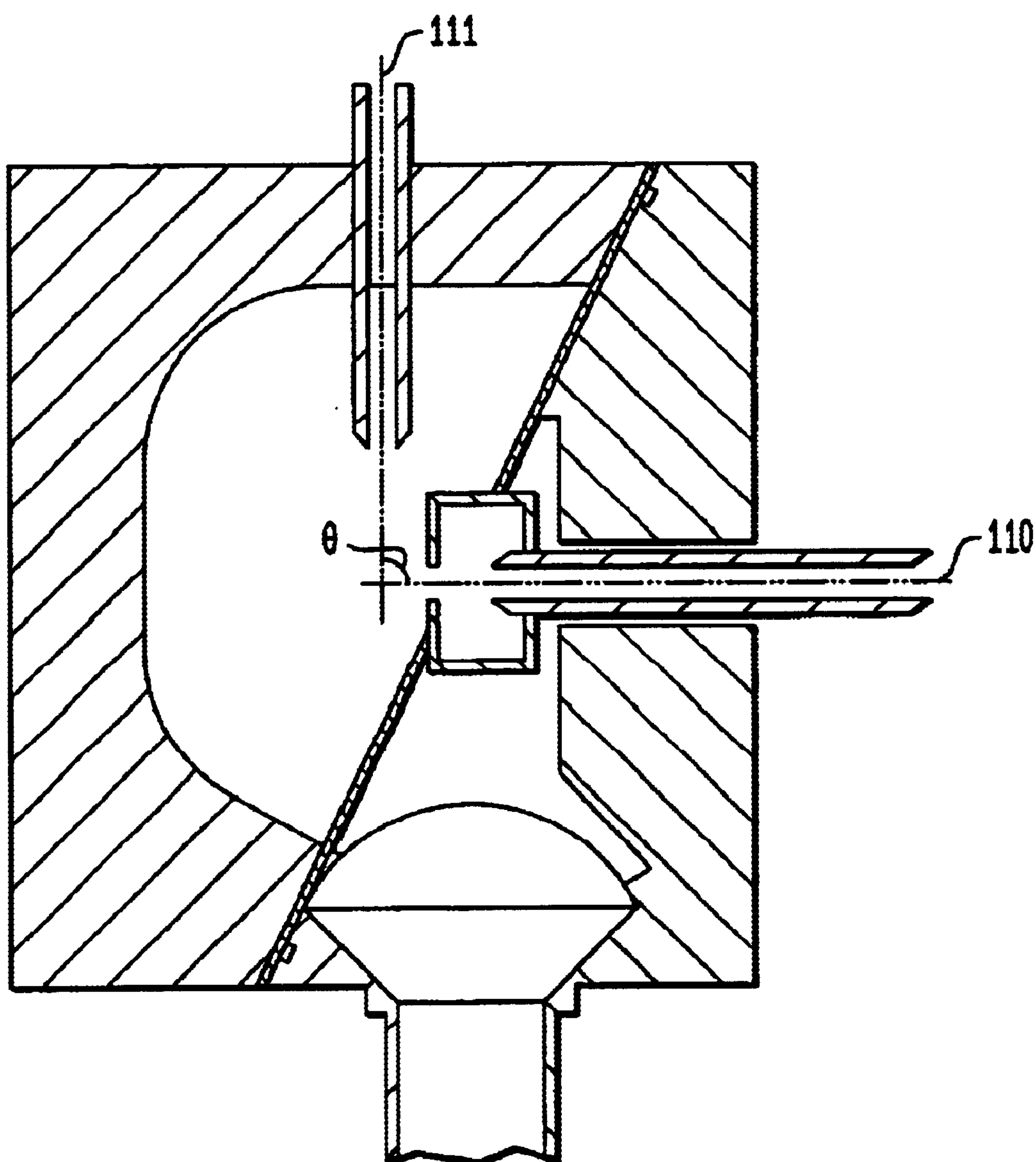
FIG. 3 (PRIOR ART)
