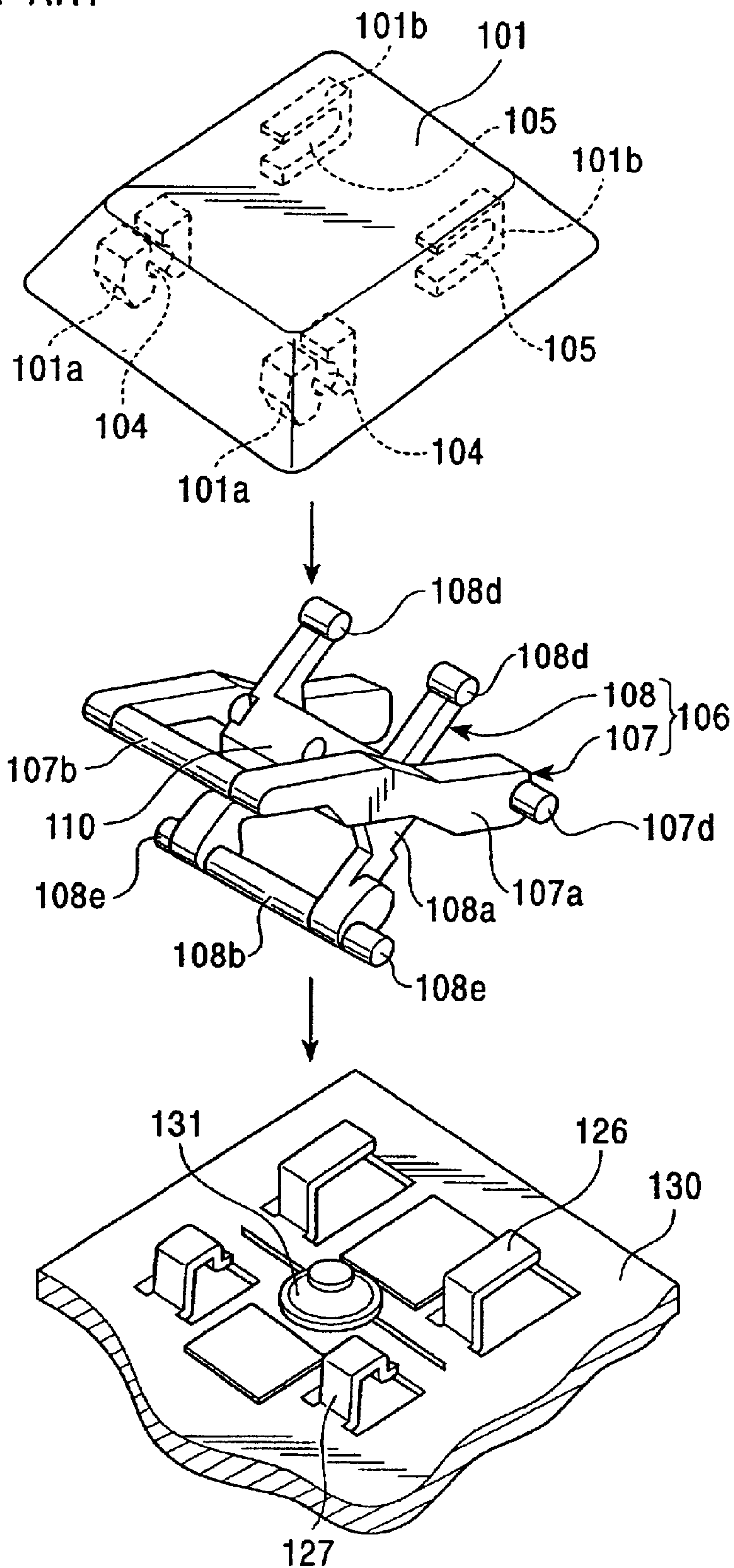
FIG. 27 PRIOR ART
