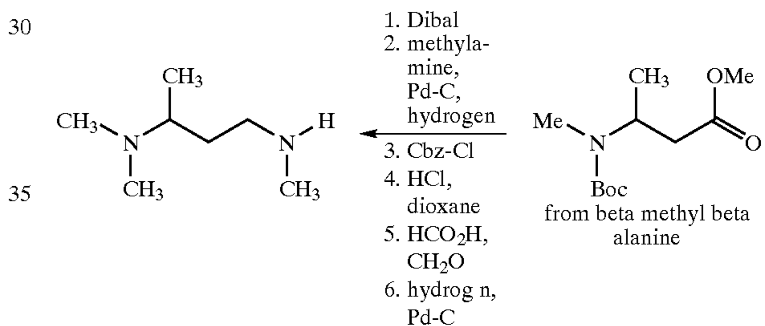
Synthetic Scheme 3
