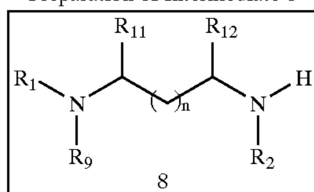
Synthetic Scheme 3
