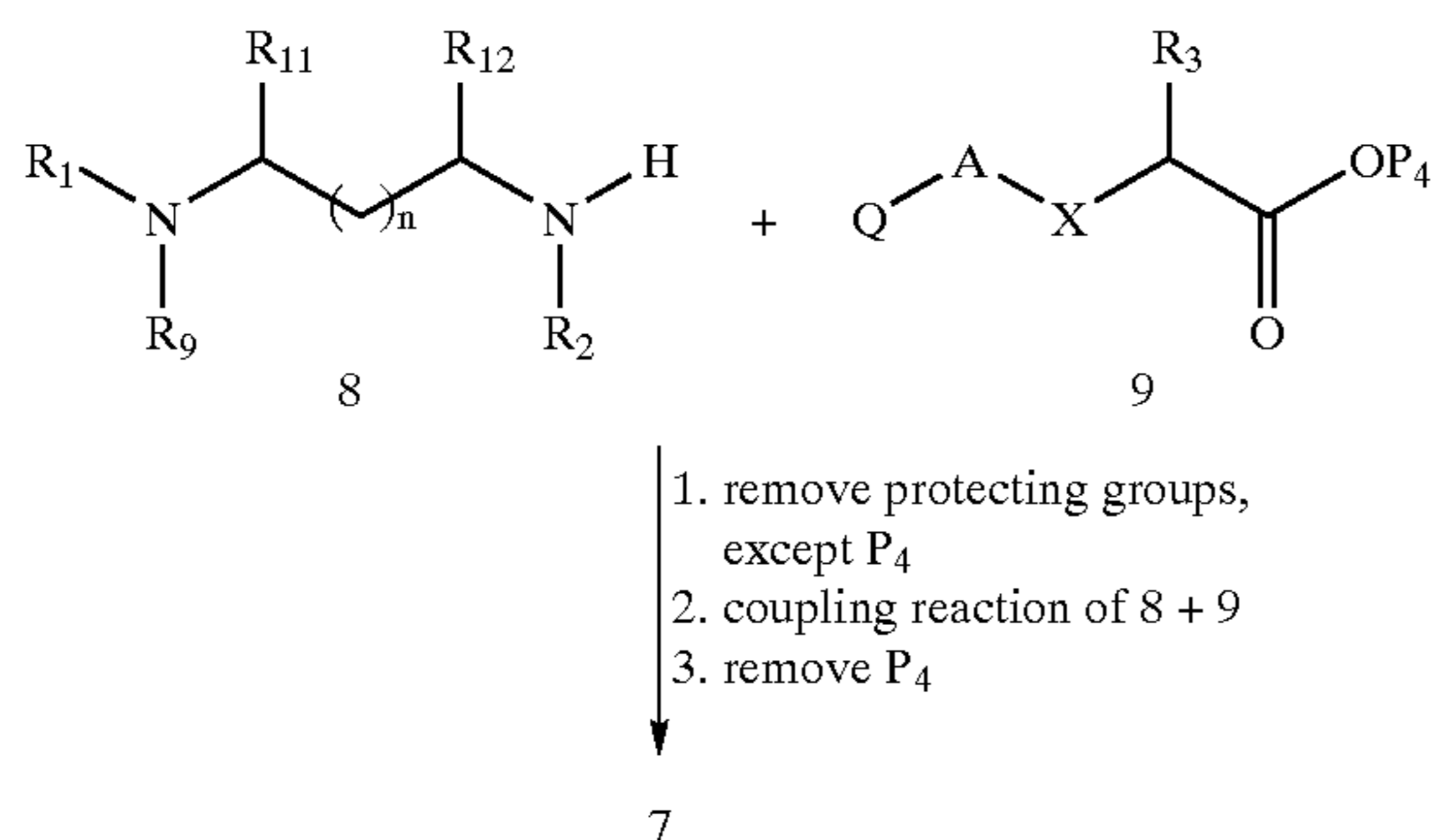
Synthetic Scheme 2
