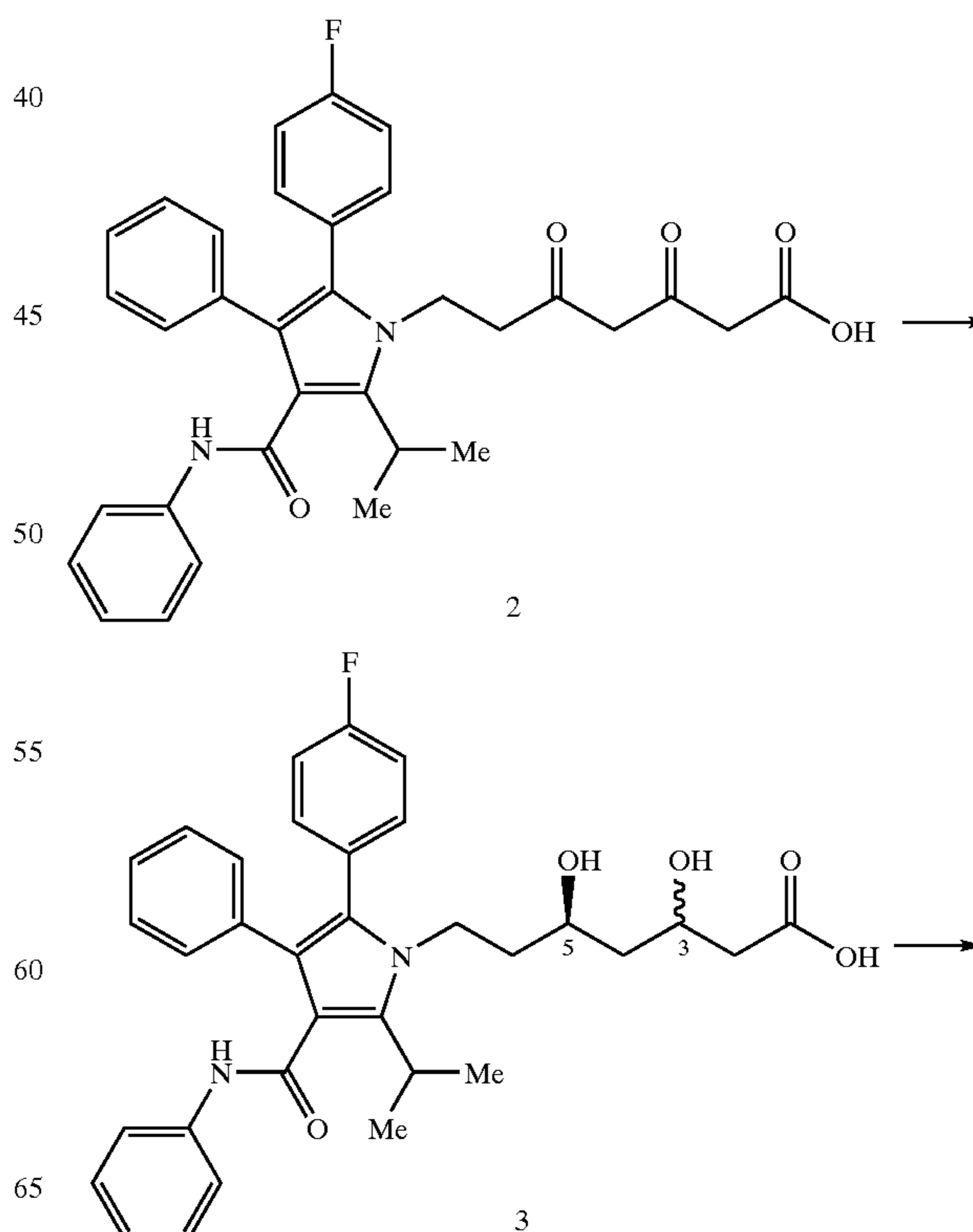
Scheme 1
