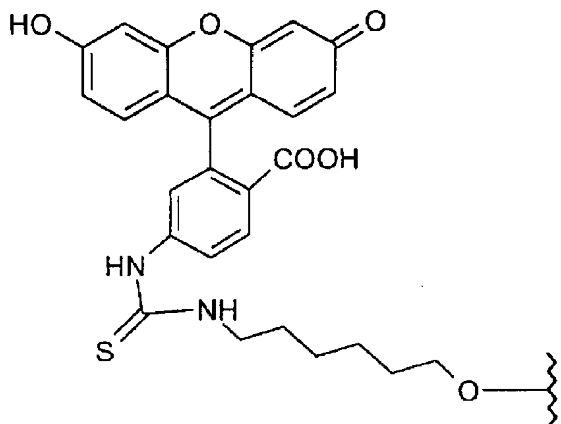
Fluorescein (Thiourea)
