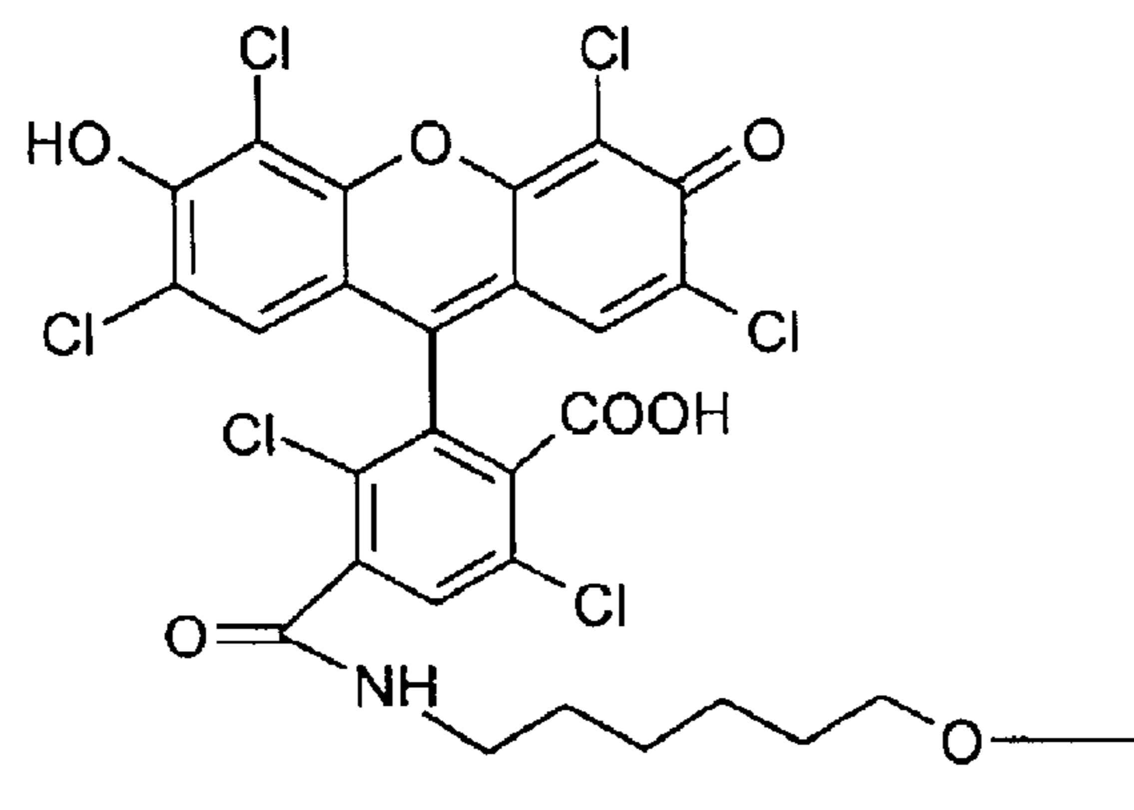
Hexachlorofluorescein
