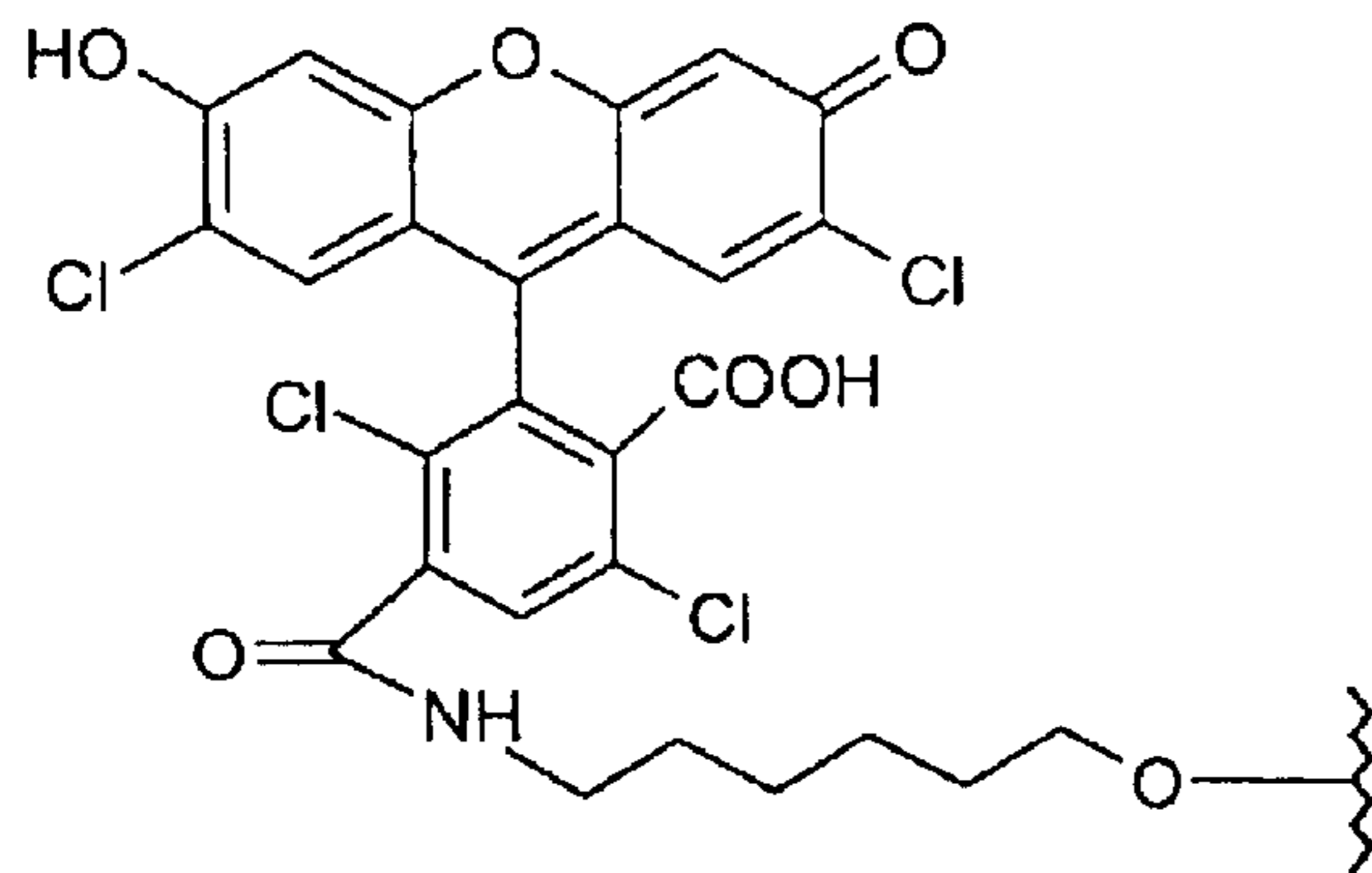
Tetrachlorofluorescein
