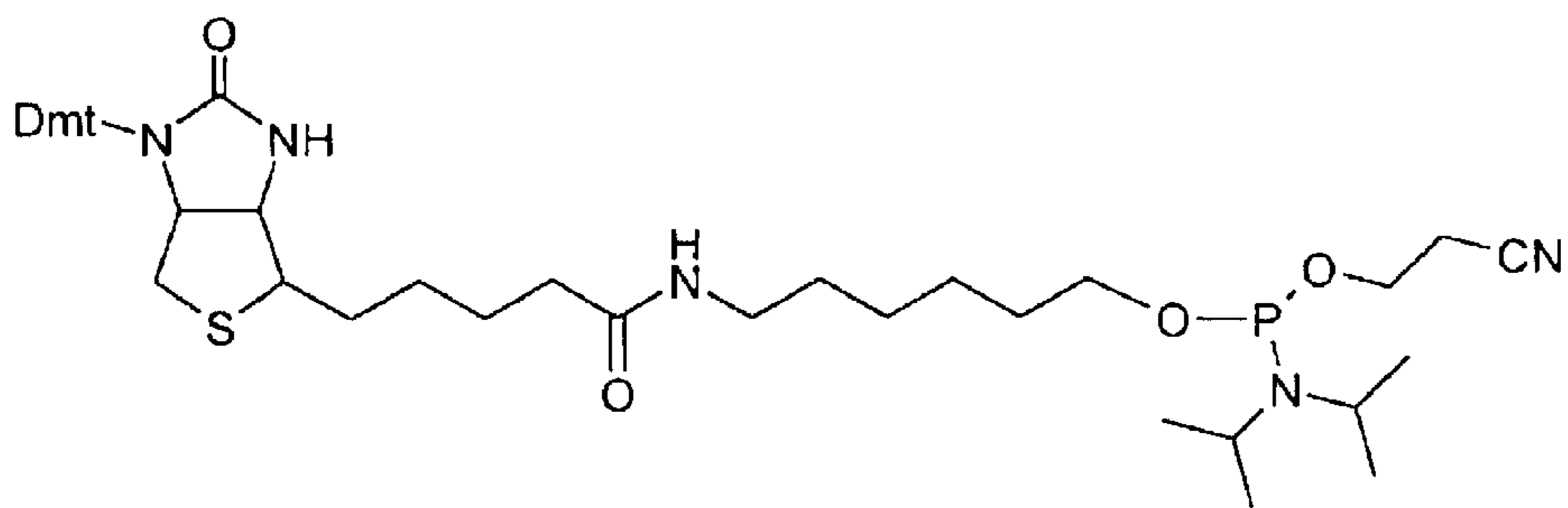
Biotin phosphoramidite 5 (monofunctional)
