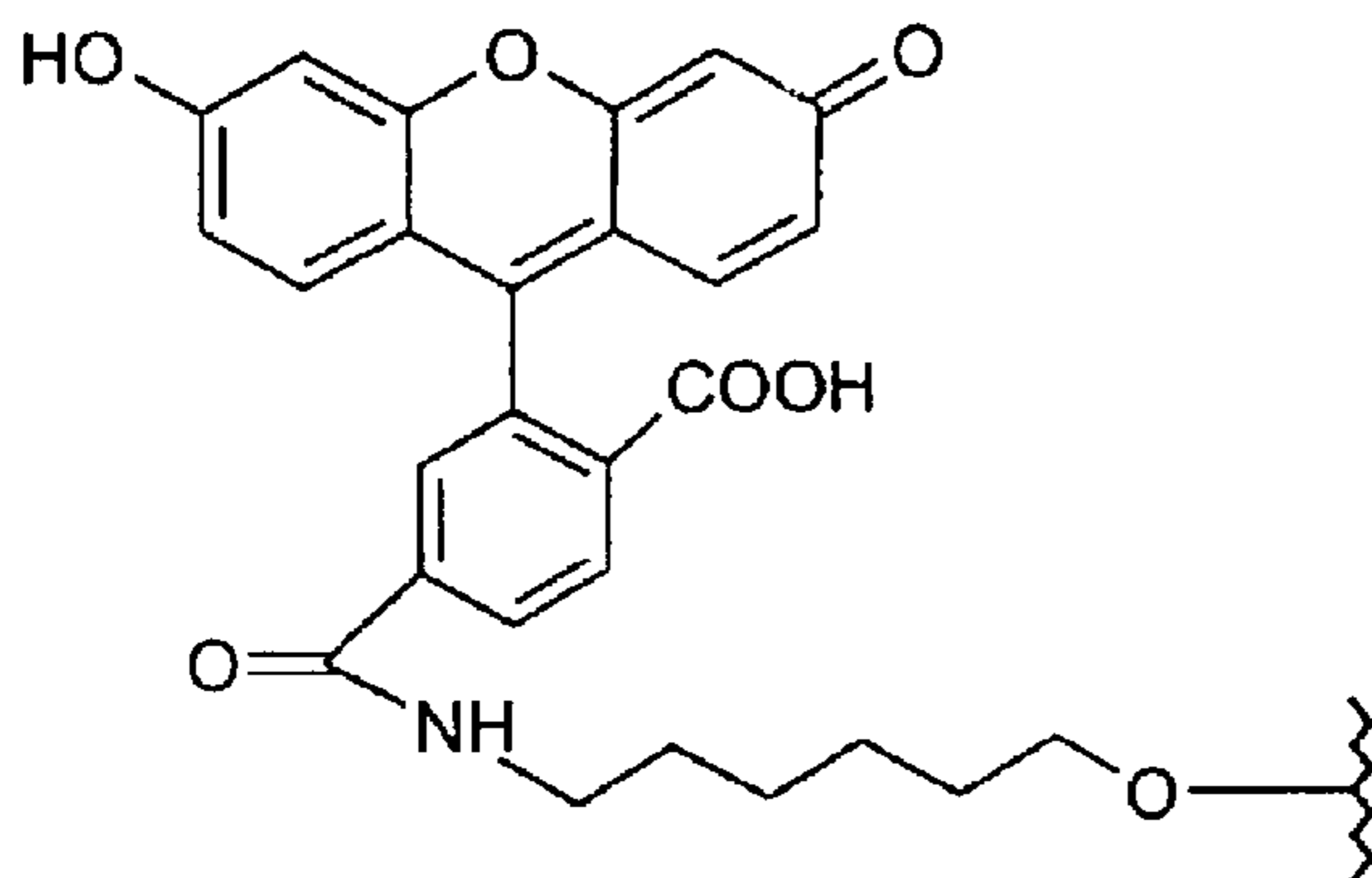
Fluorescein (Amide)
