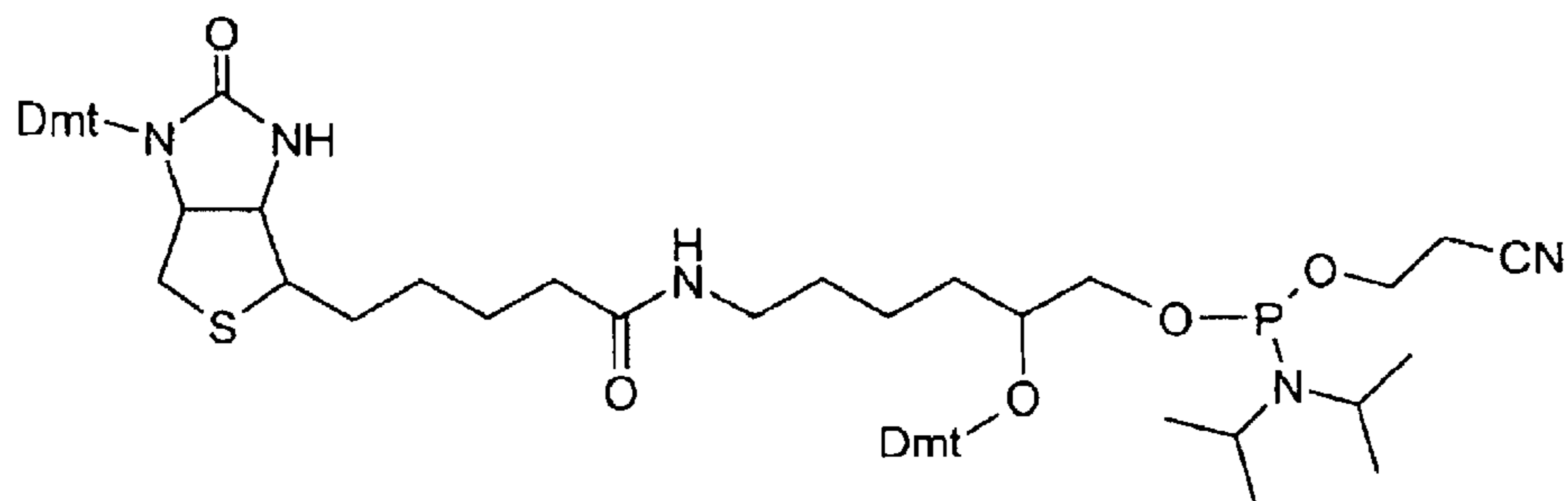
Biotin phosphoramidite 6 (bifunctional)
