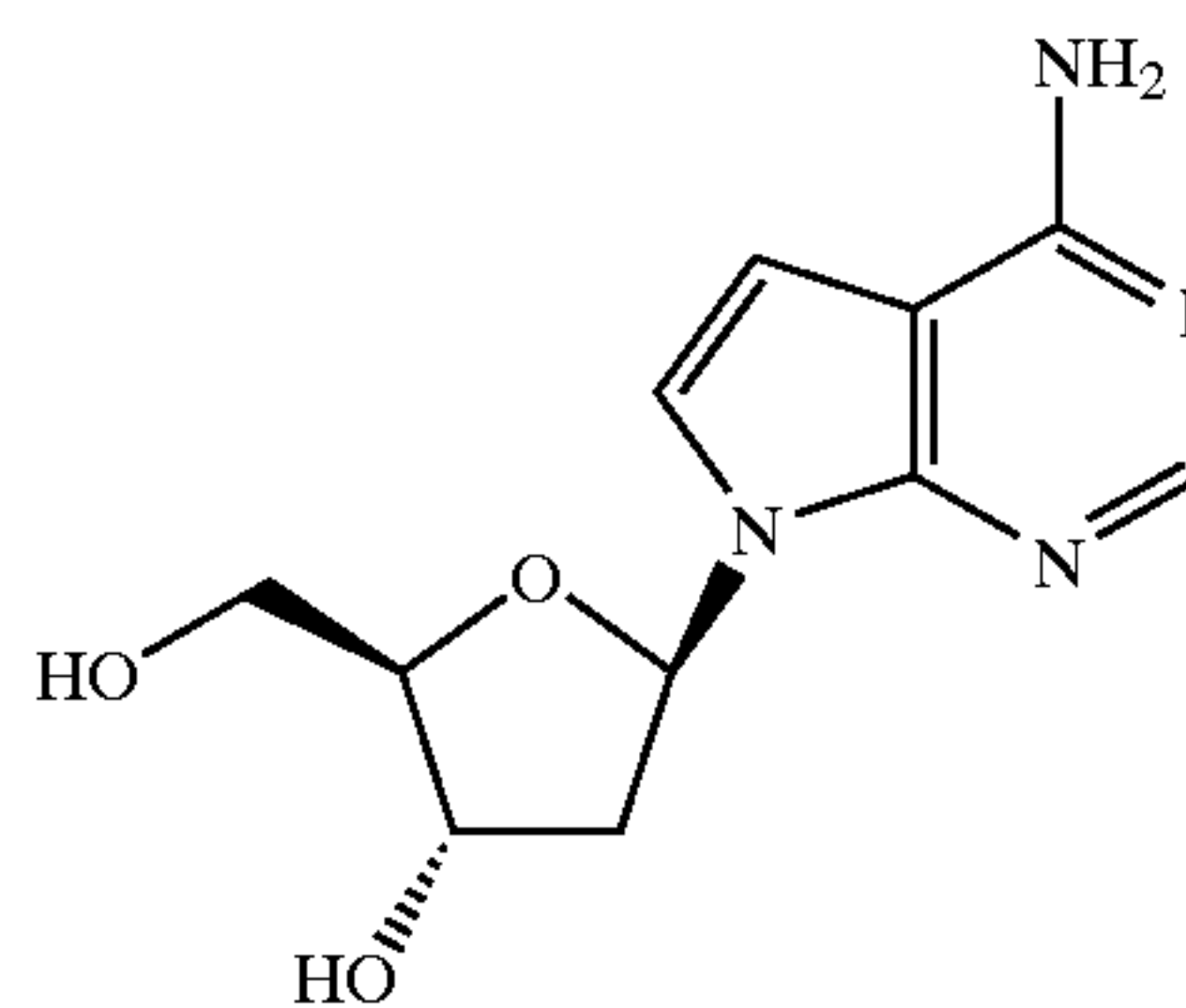
2-Amino-7-(2-deoxy-β-D-ribofuranosyl)-7H-pyrrolo [2,3-d]pyrimidine
