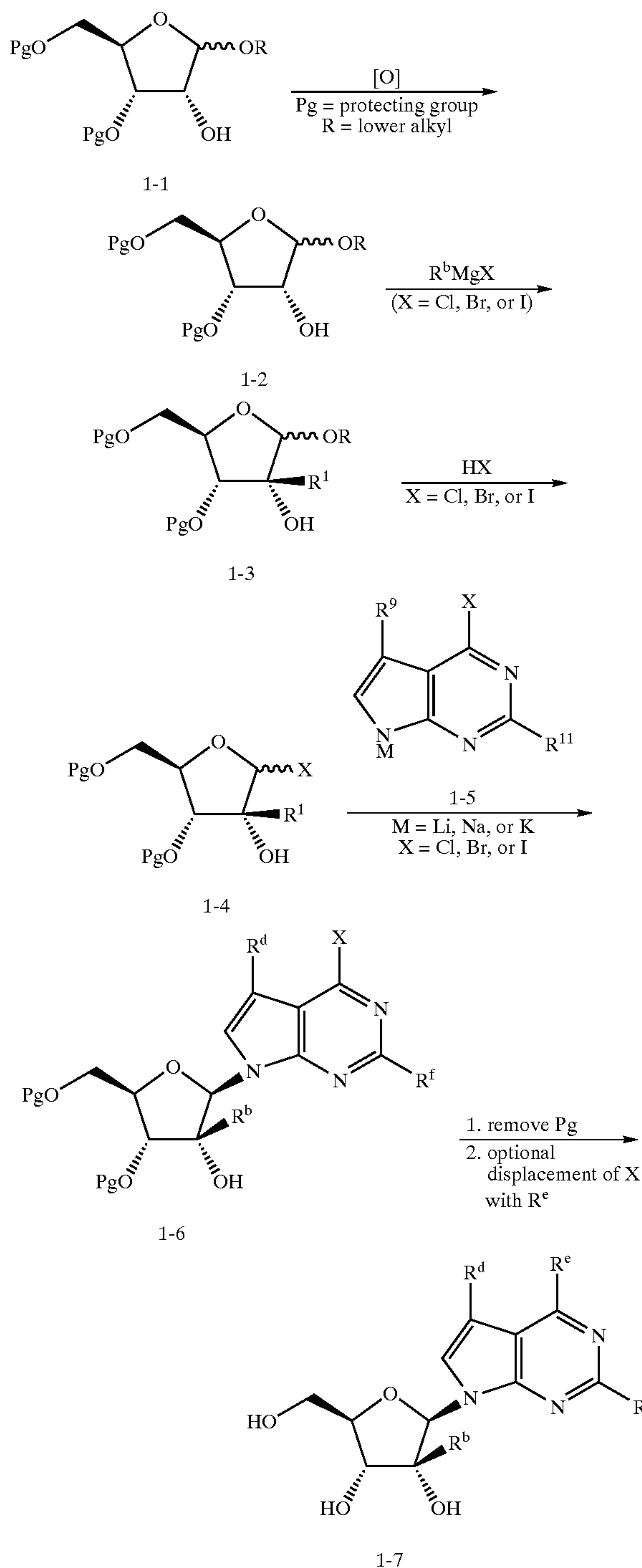
Scheme 1
