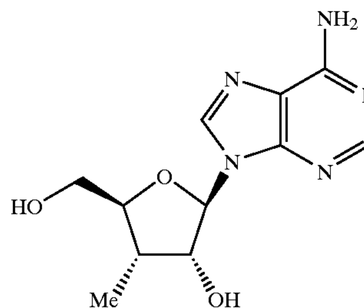
3'-Deoxy-3'-methyladenosine
