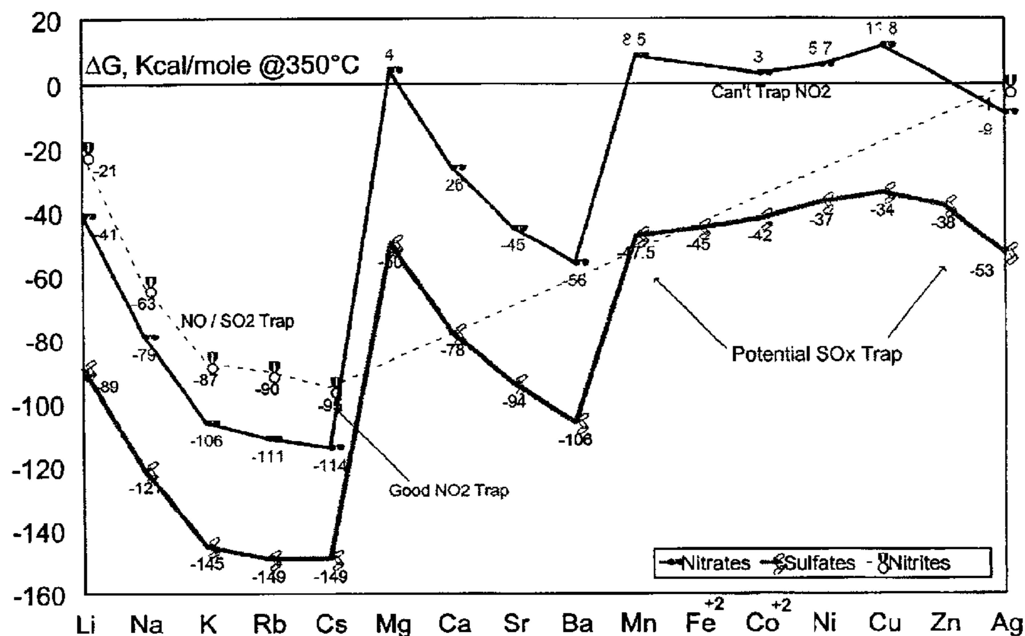
Free Energies of Formation of Nitrates, Sulfates, & Nitrites
