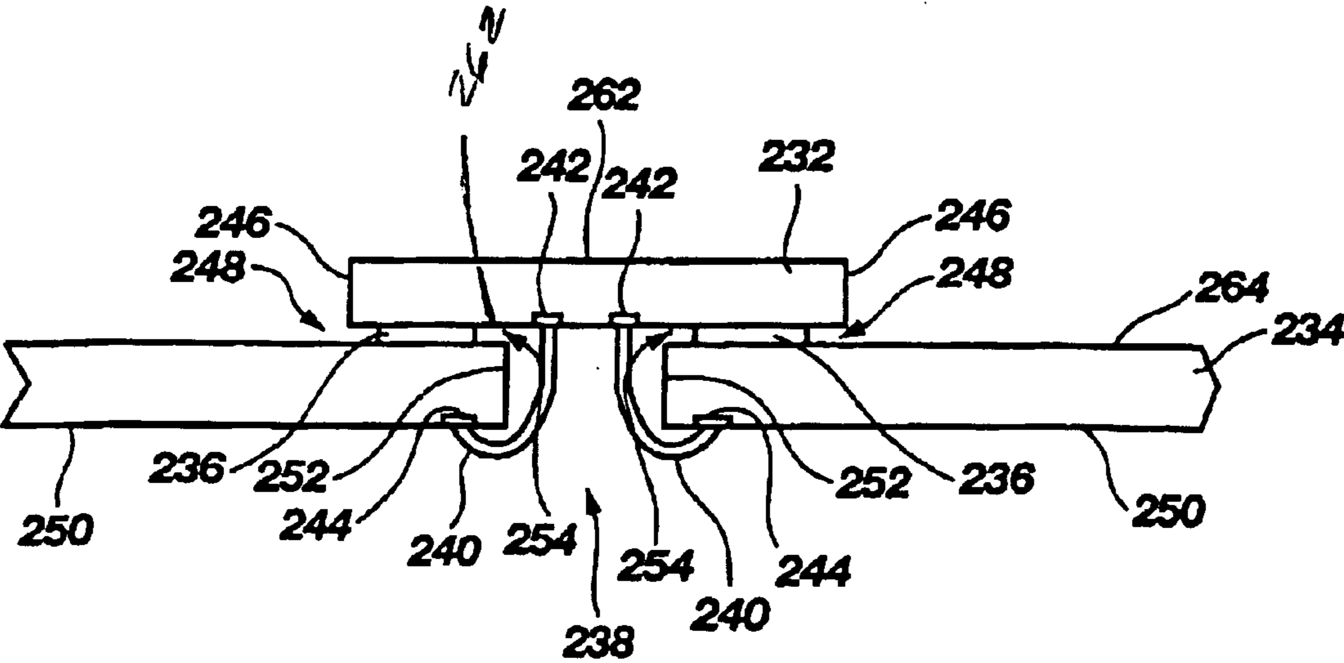
Fig. 16 (PRIOR ART)
