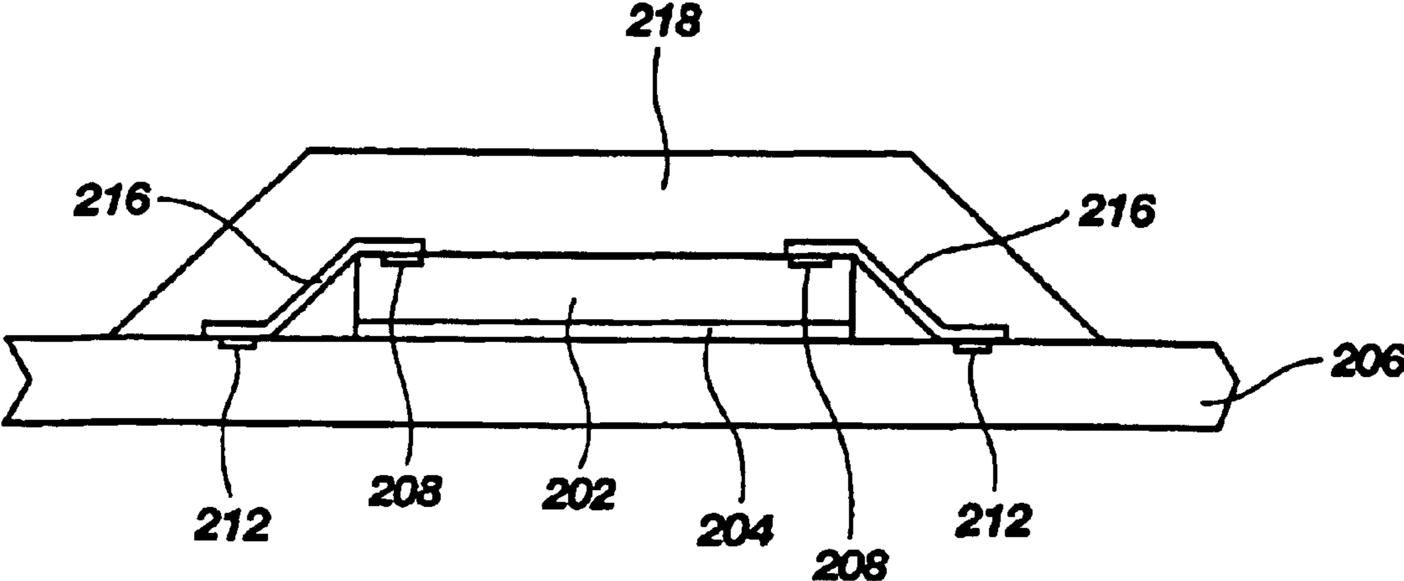
Fig. 15 (PRIOR ART)
