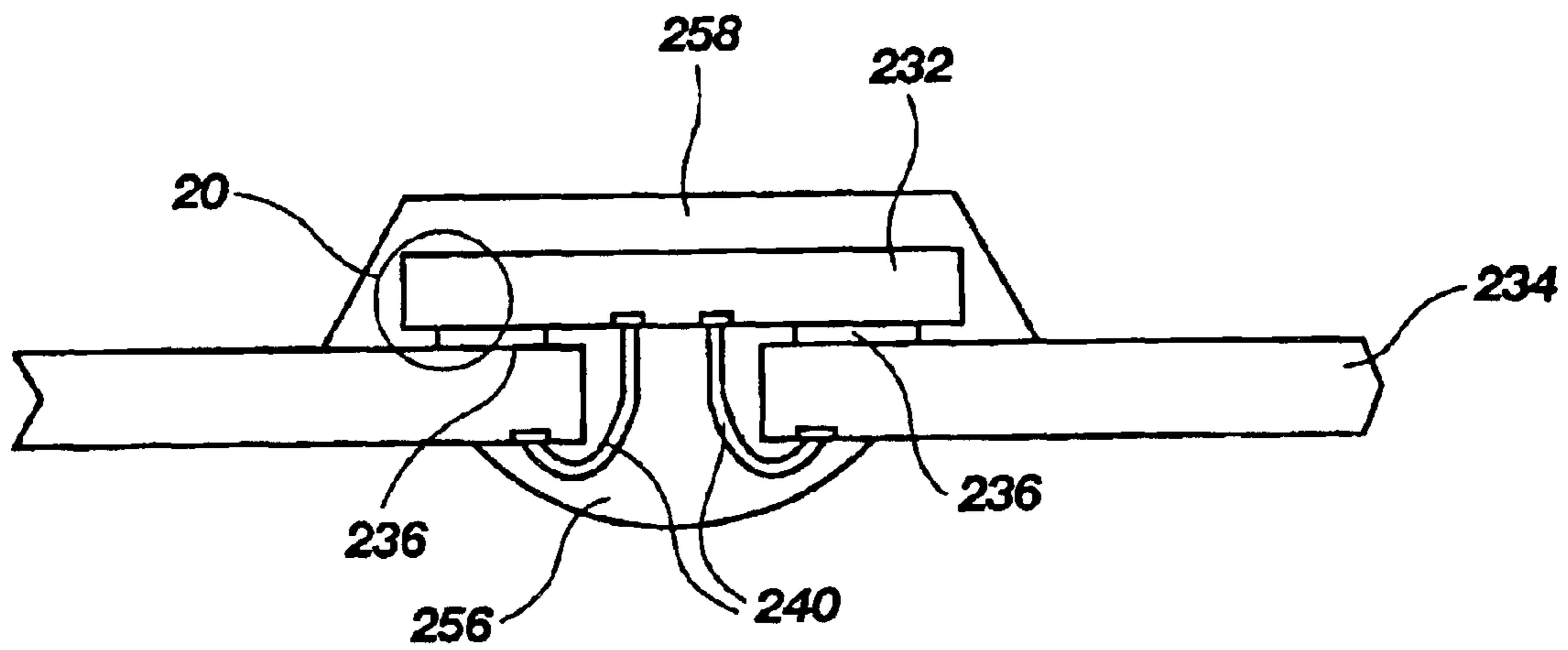
Fig. 18 (PRIOR ART)
