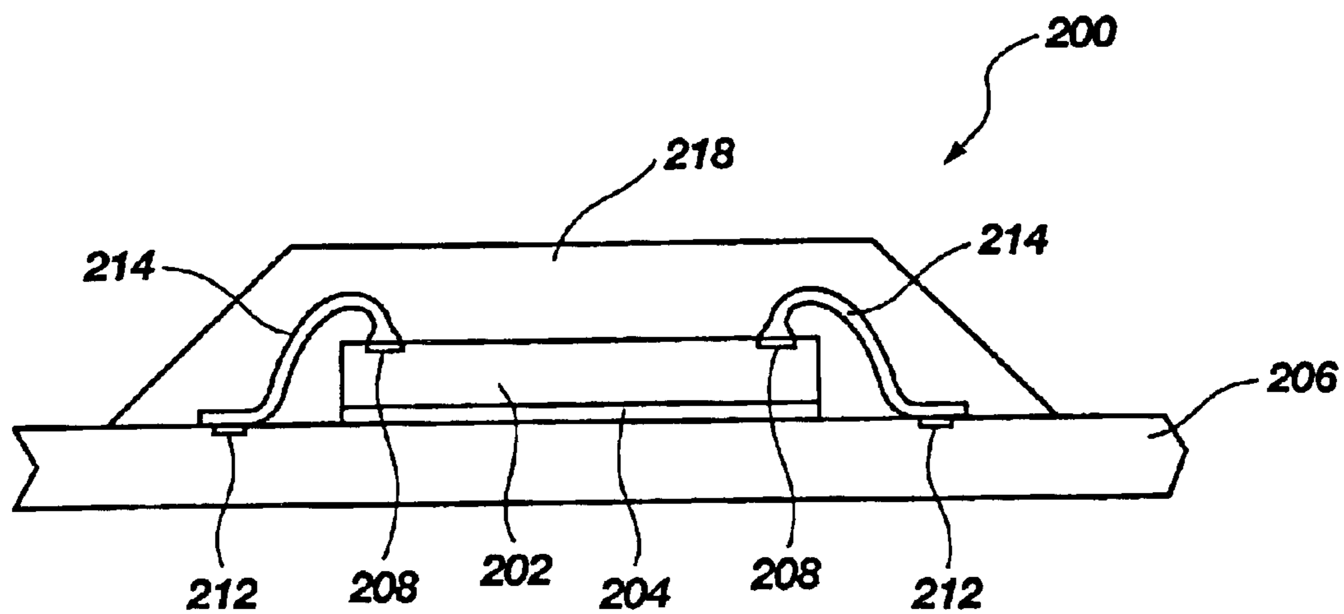
Fig. 14 (PRIOR ART)
