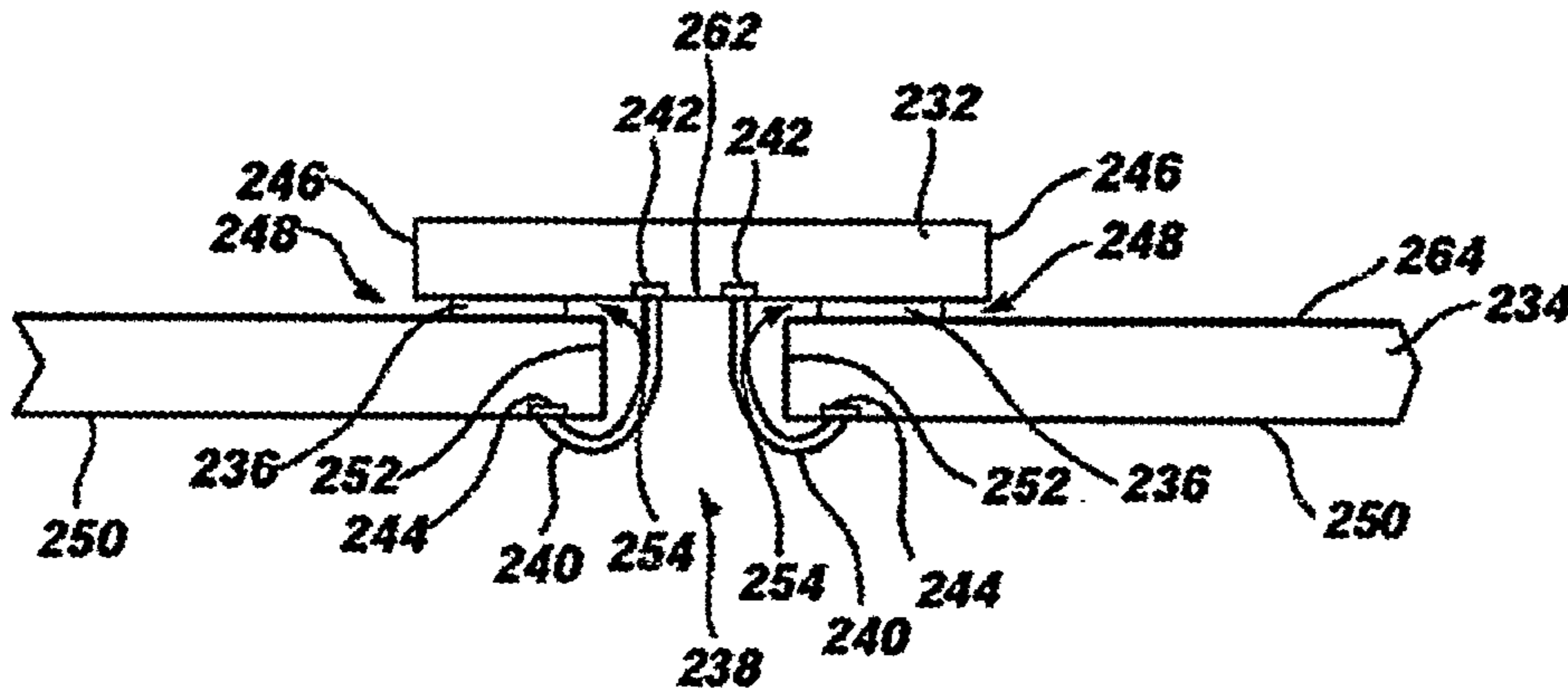
Fig. 16 (PRIOR ART)
