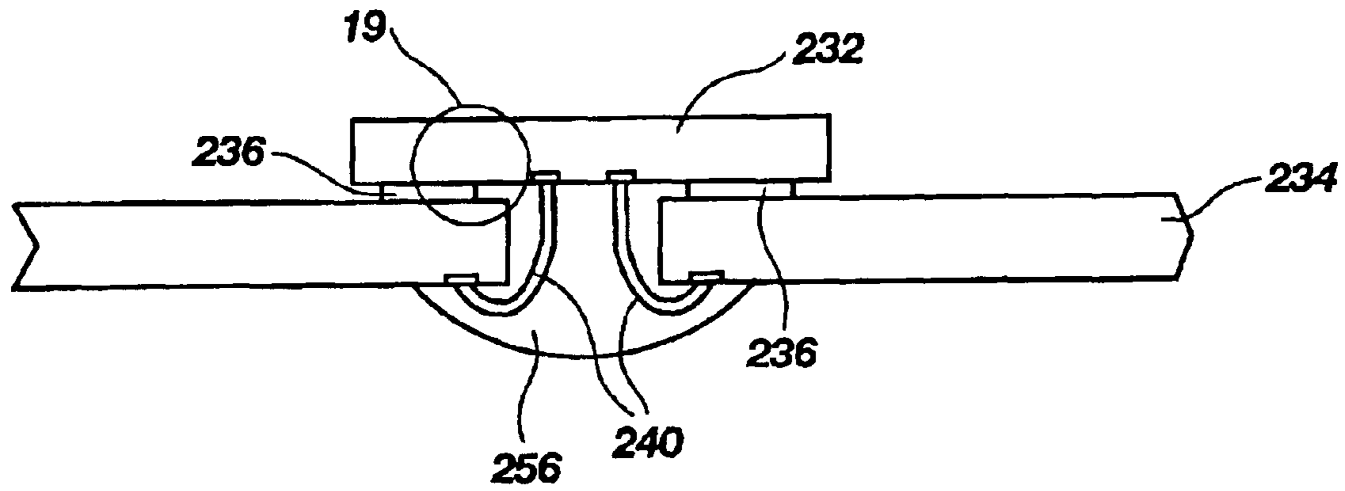
Fig. 17 (PRIOR ART)
