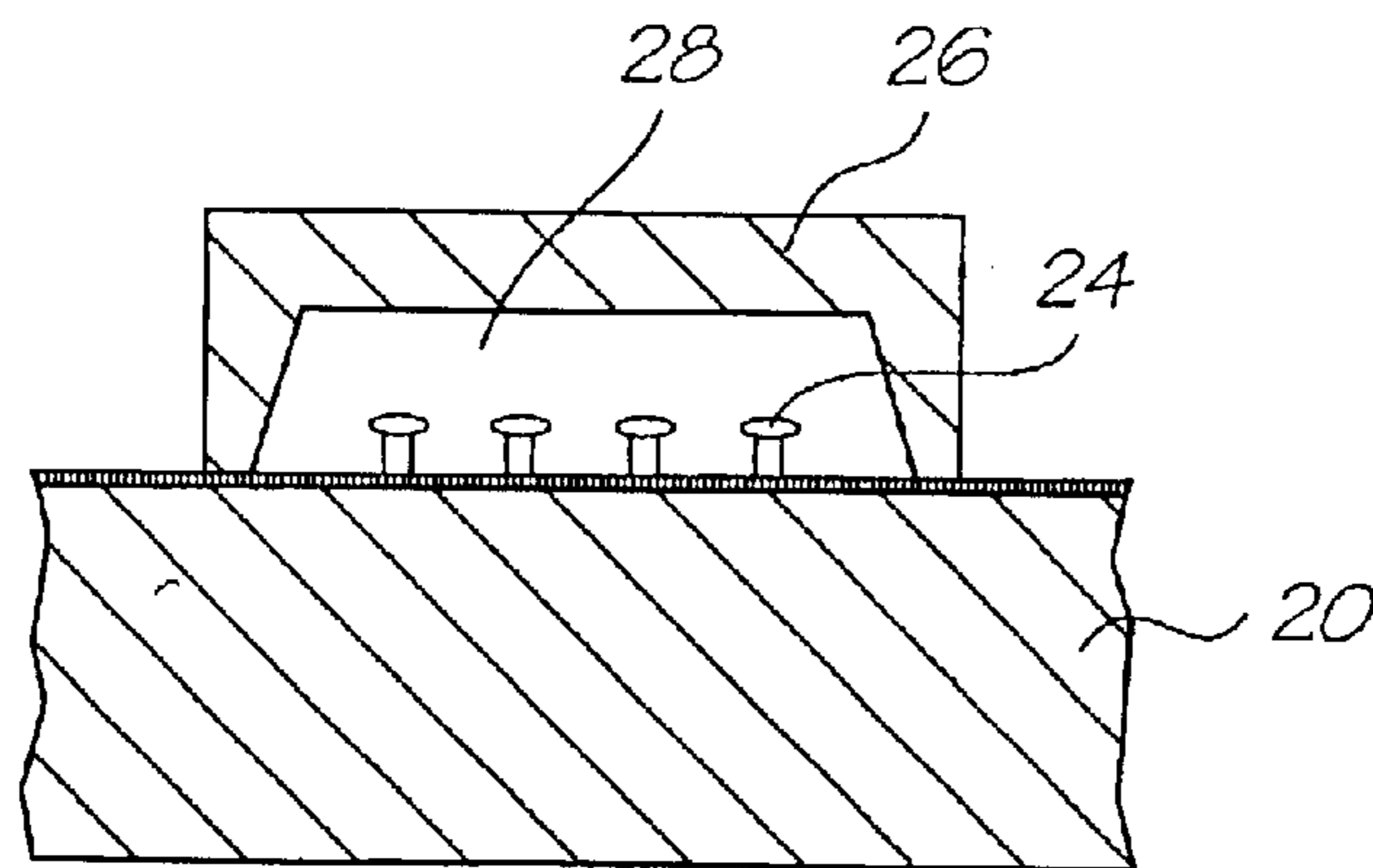
FIG. 3 (Prior Art)
