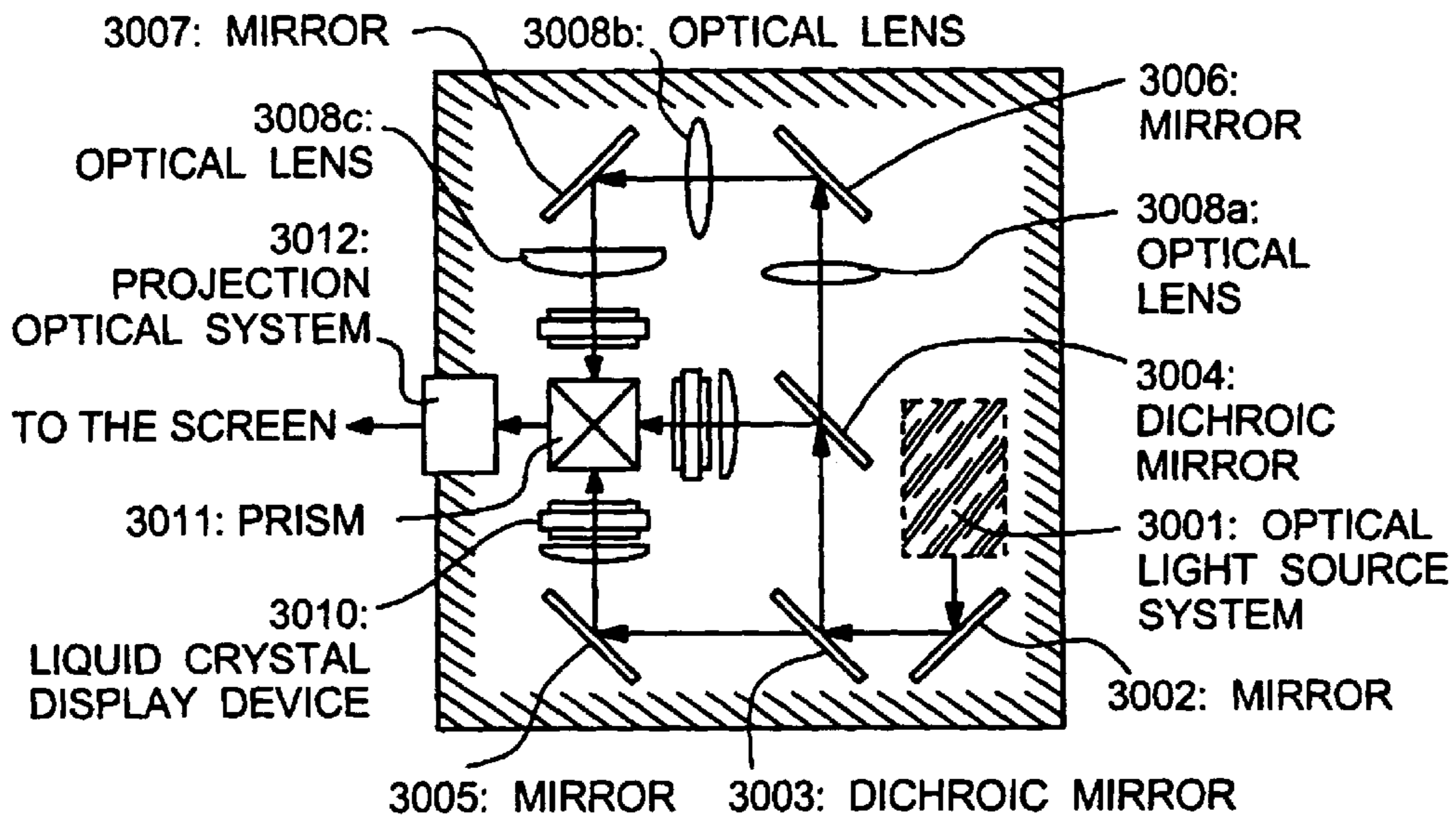
FIG. 25(A): OPTICAL ENGINE (3-PLATE TYPE)
