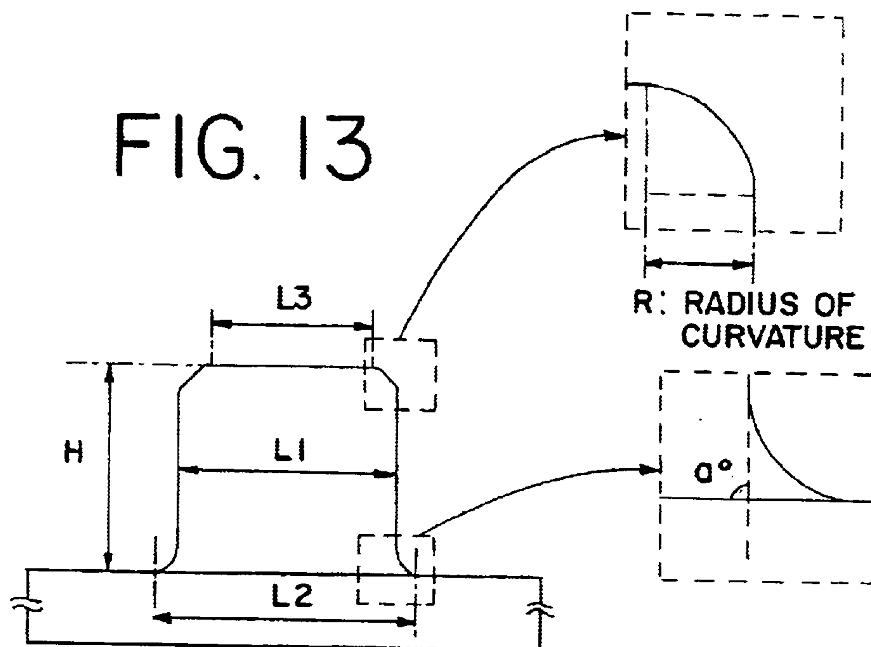
SECTIONAL TYPICAL VIEW OF SPACER
