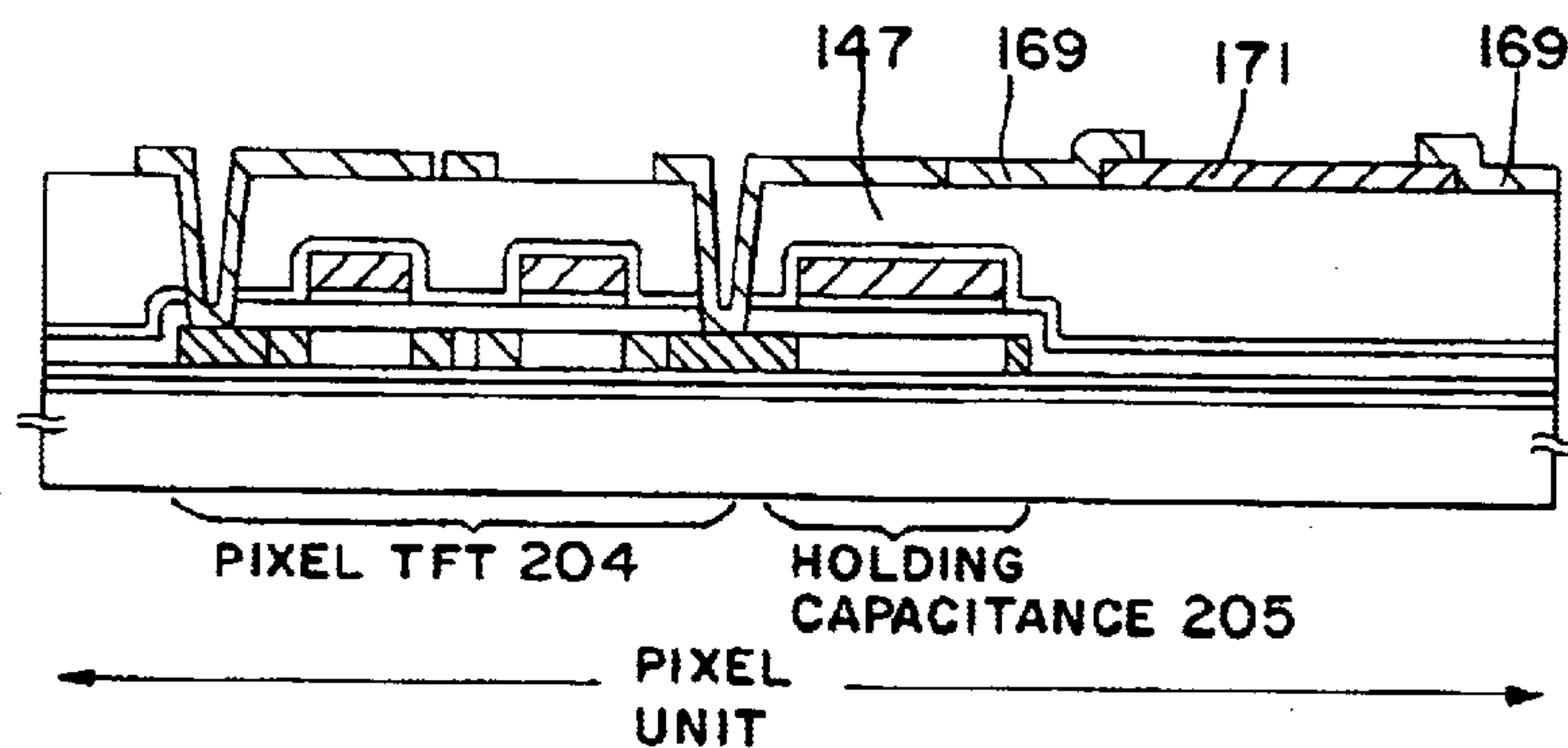
SECTIONAL VIEW OF PIXEL UNIT
