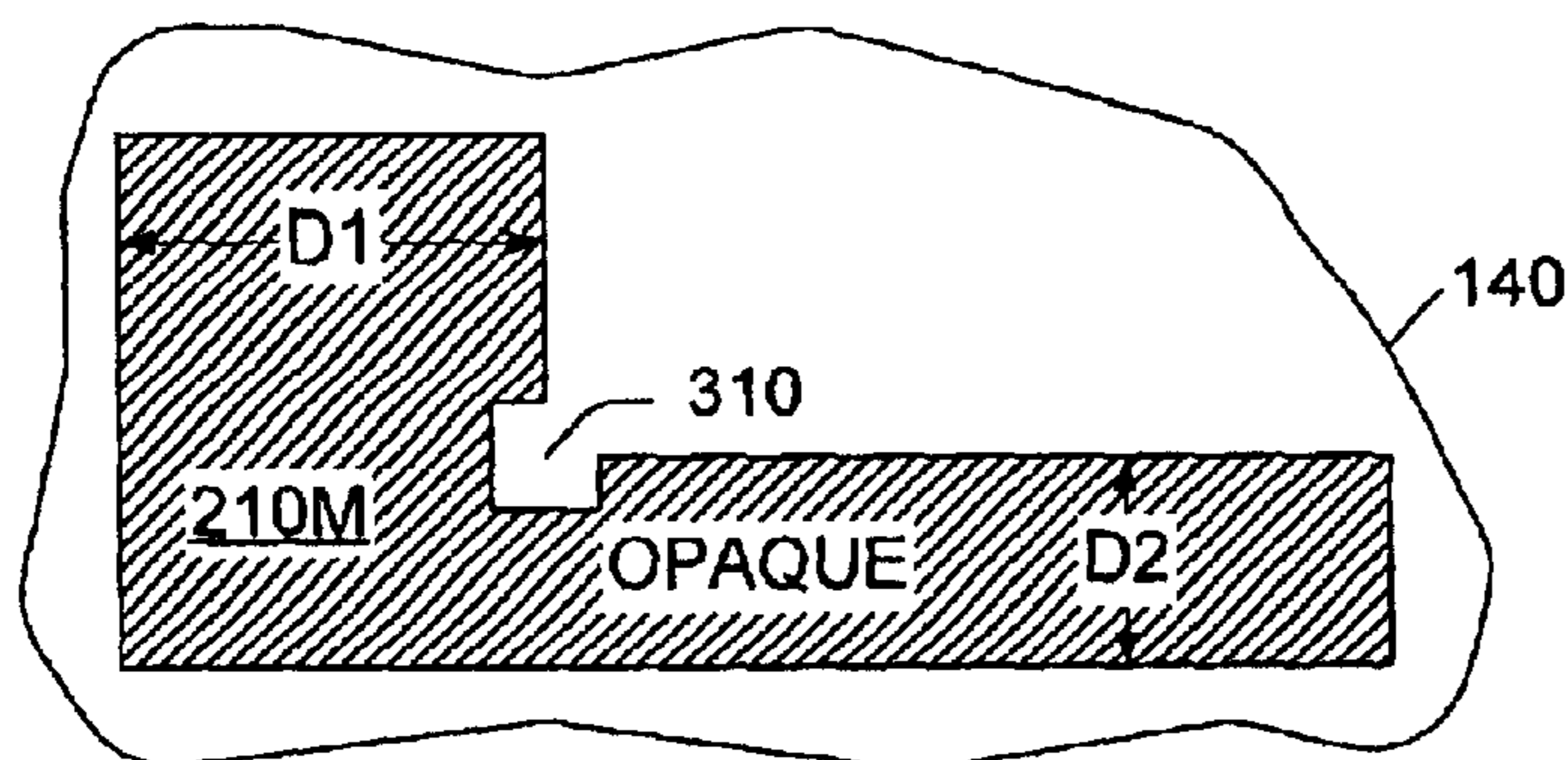
FIG. 3 PRIOR ART
