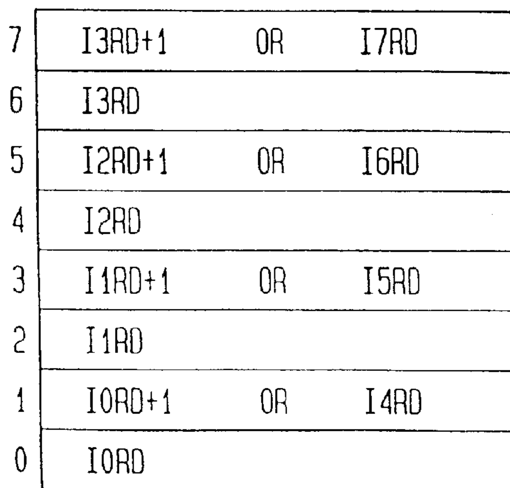
FIG. 5B TEMPORARY BUFFER 403
