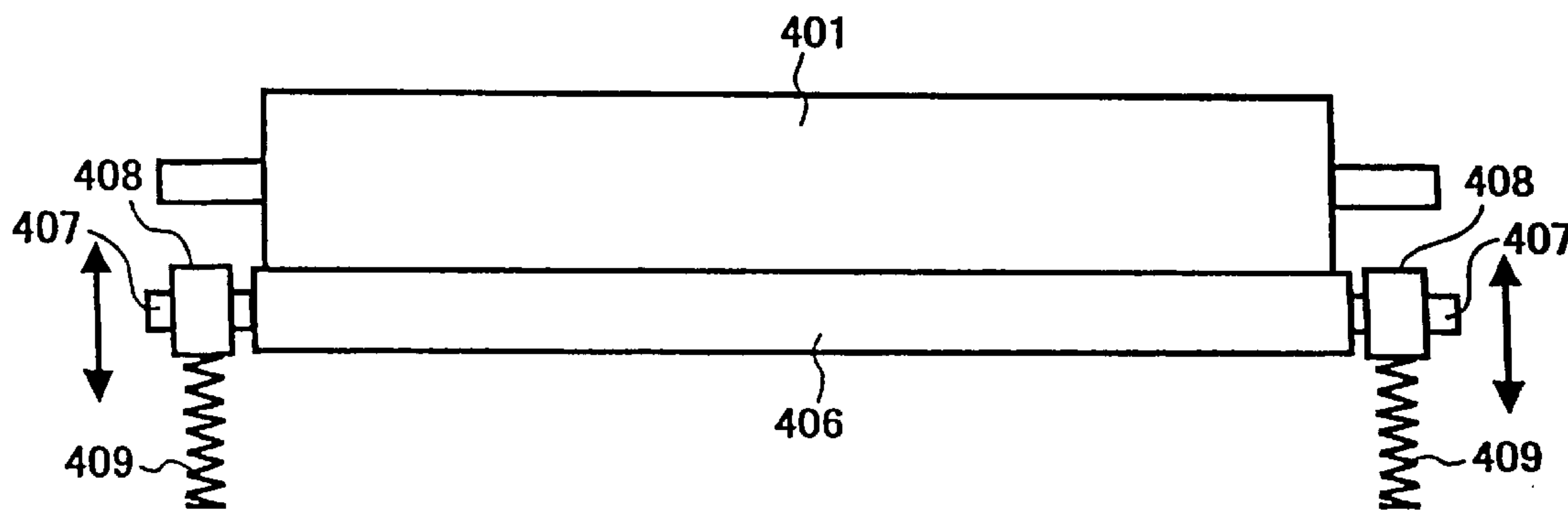
FIG. 27 BACKGROUND ART
