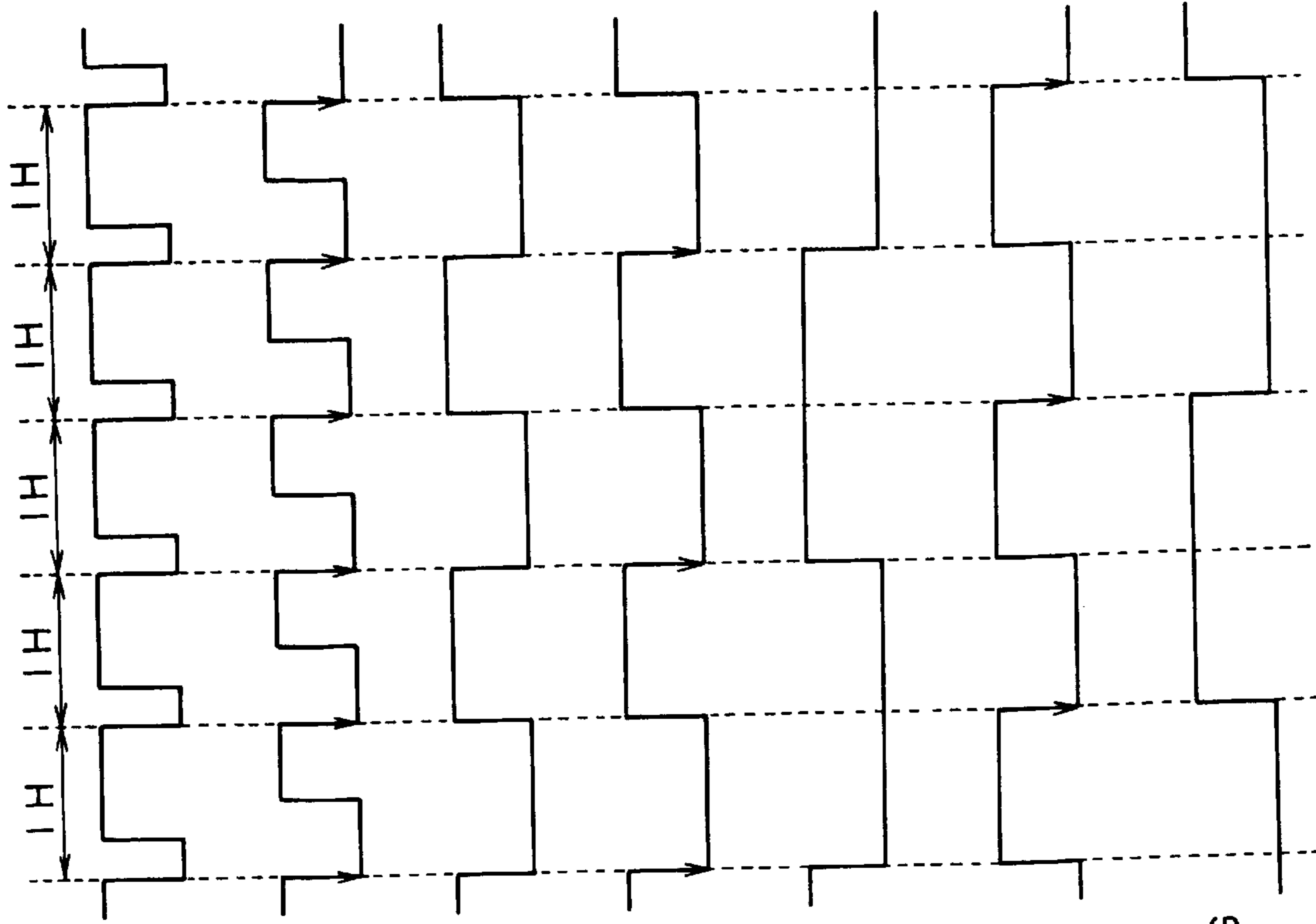
INVERSE TIMING SIGNAL HT3
