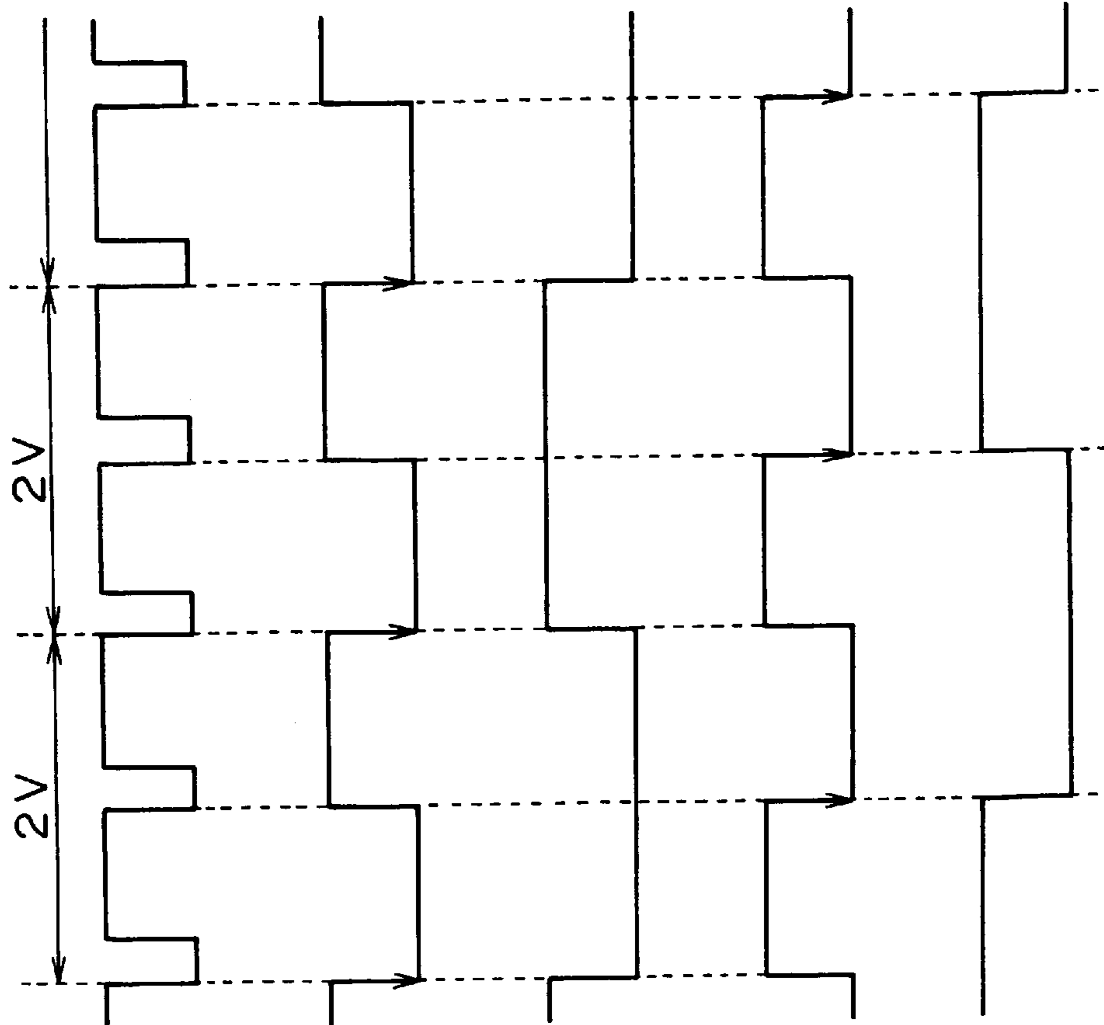
INVERSE TIMING SIGNAL HT2
