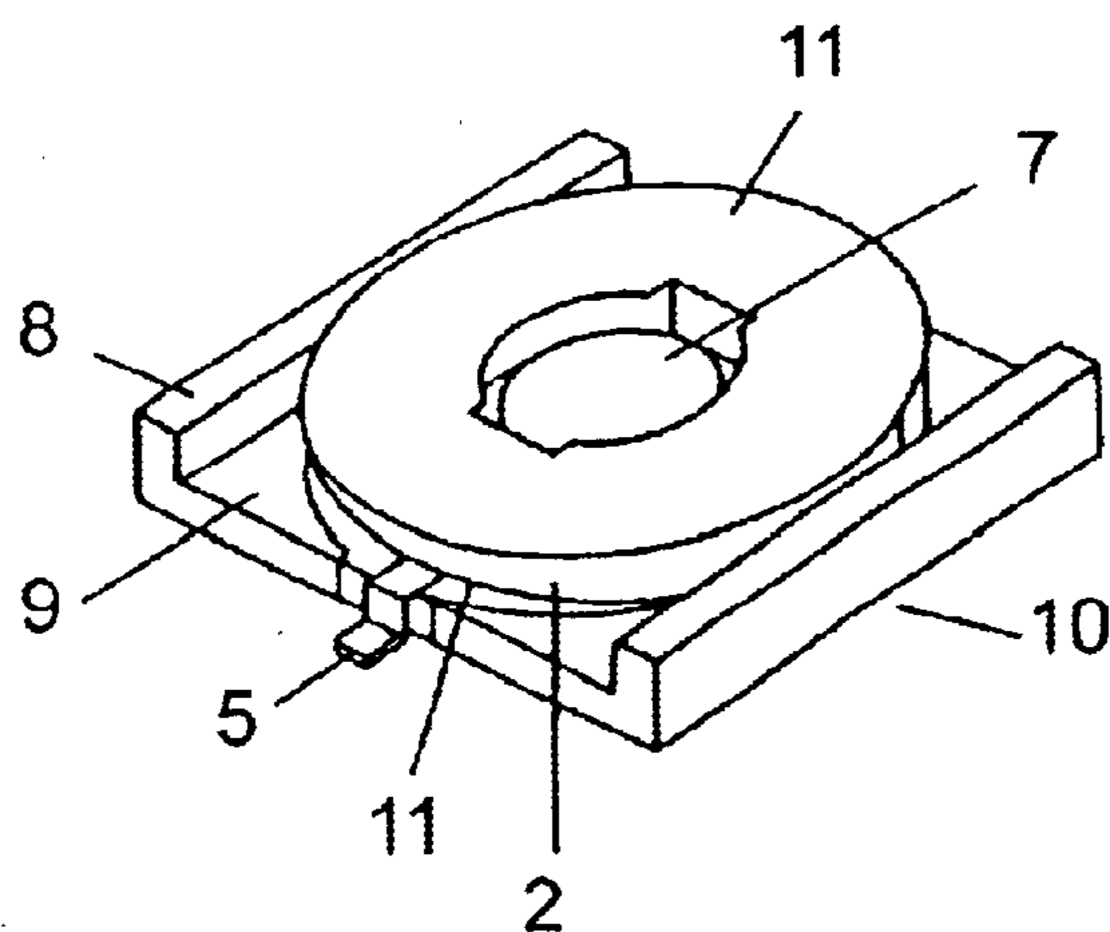
FIG. 48 PRIOR ART
