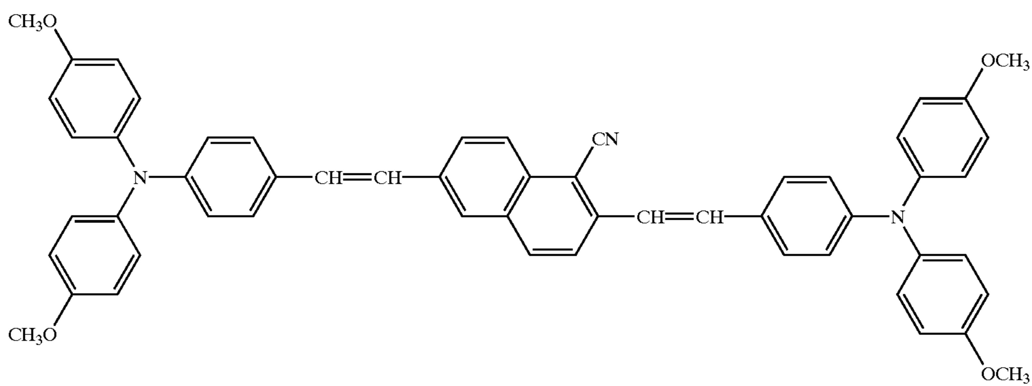
Structural formula (29)-3
