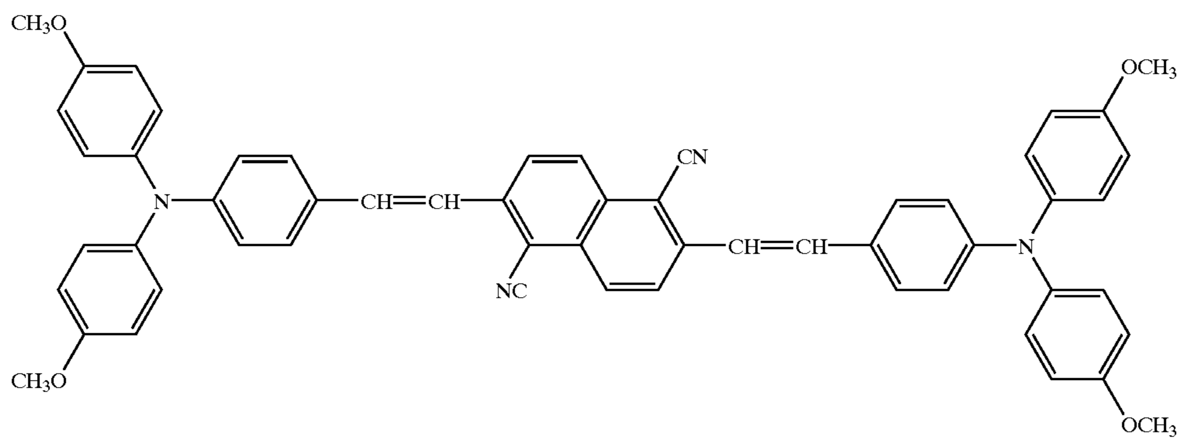
Structural formula (20)-3
