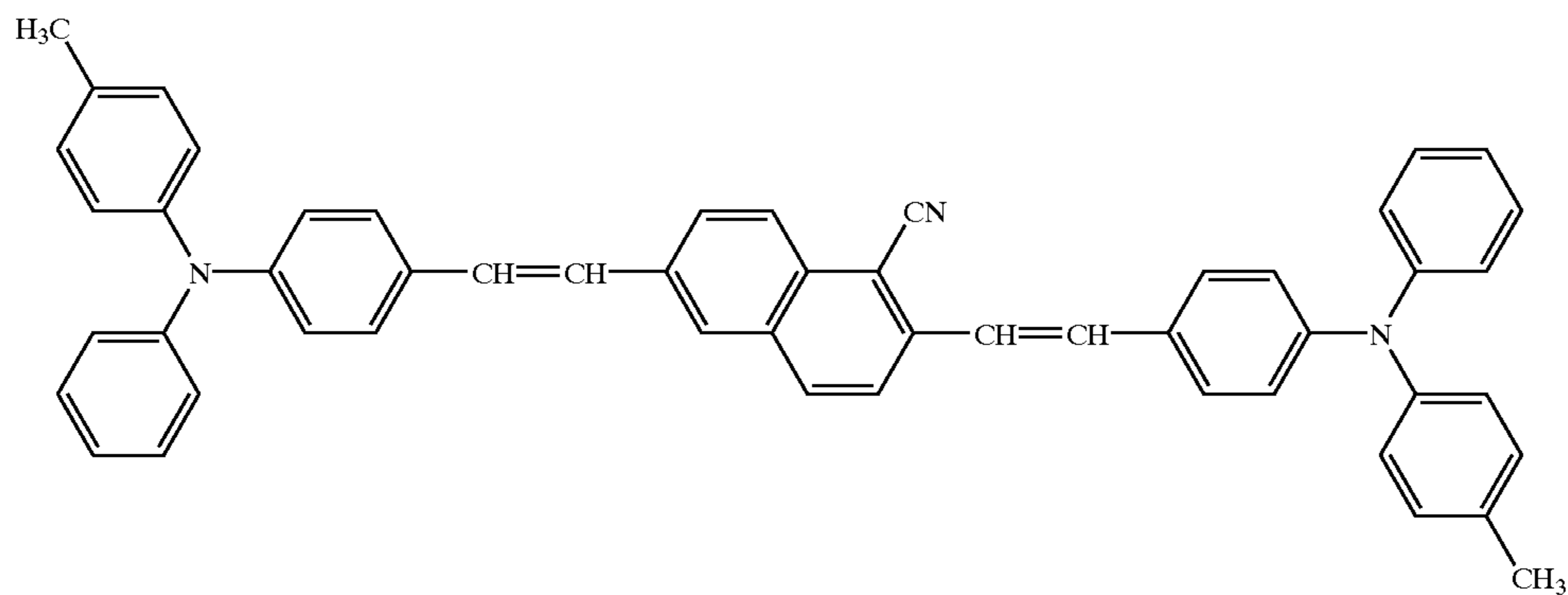
Structural formula (29)-4
