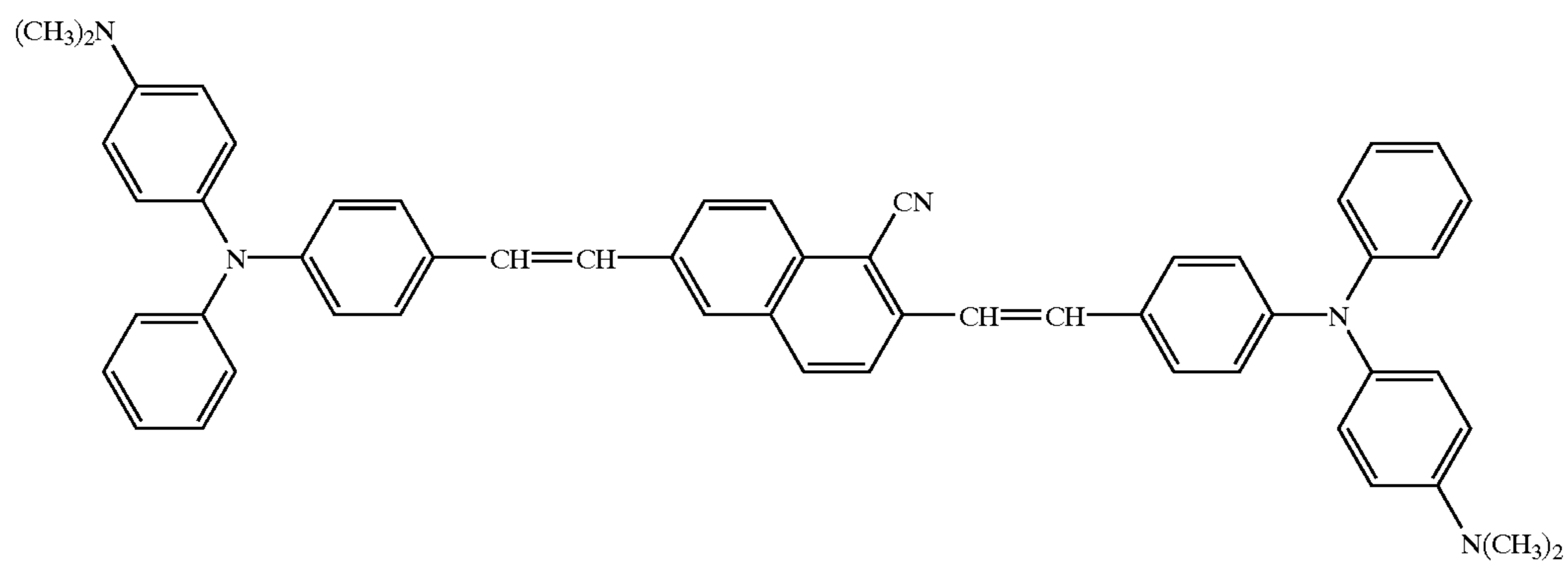
Structural formula (29)-6
