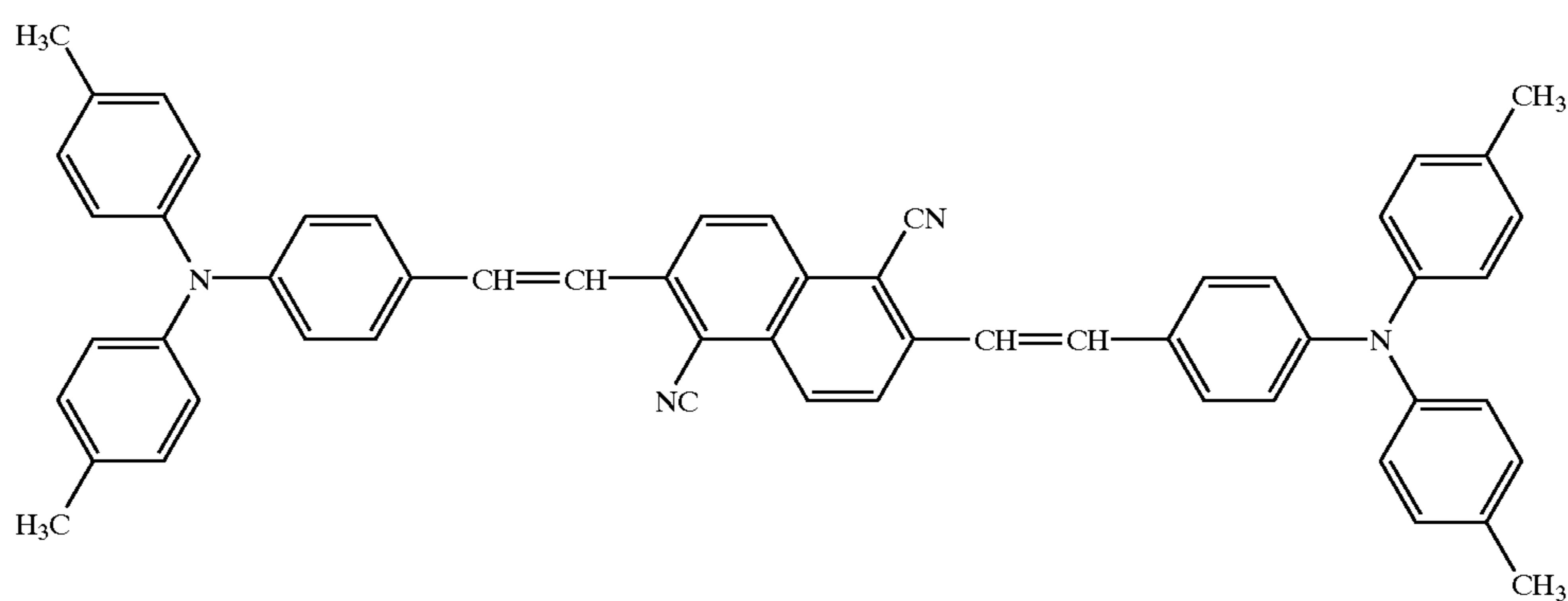
Structural formula (20)-5
