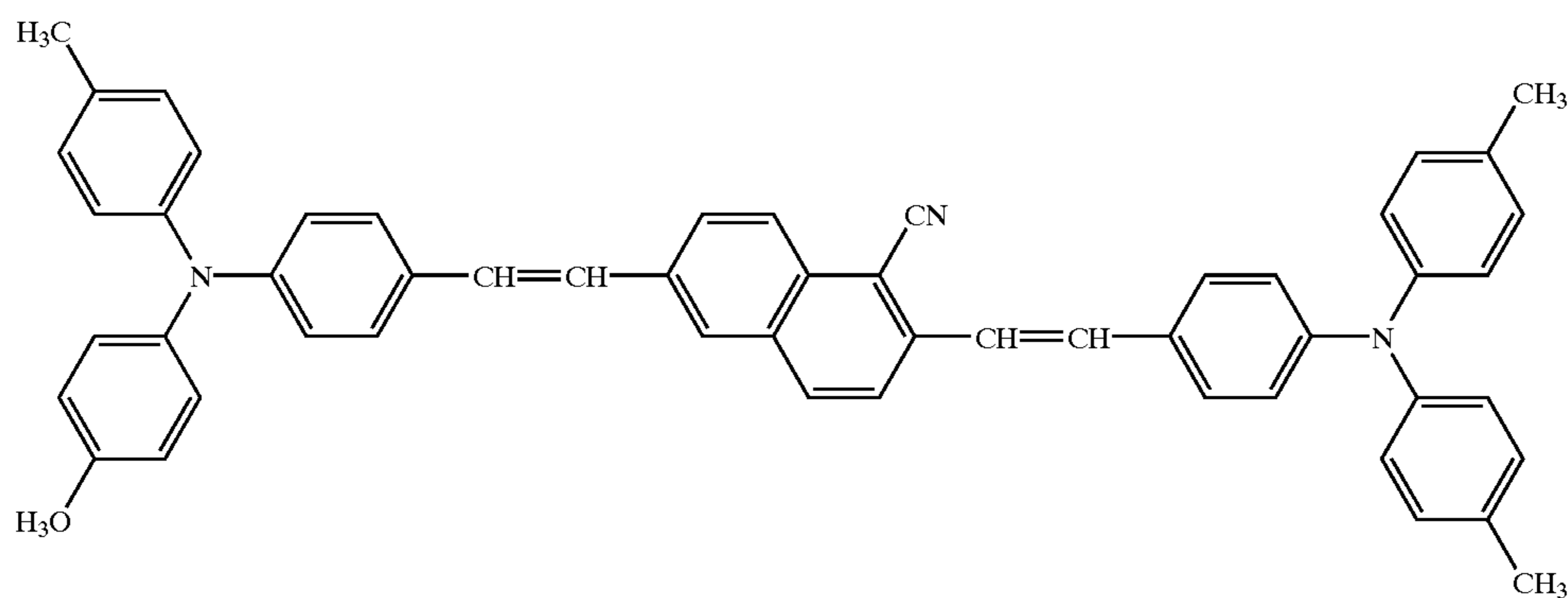
Structural formula (29)-5
