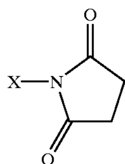
Formula [XII]
