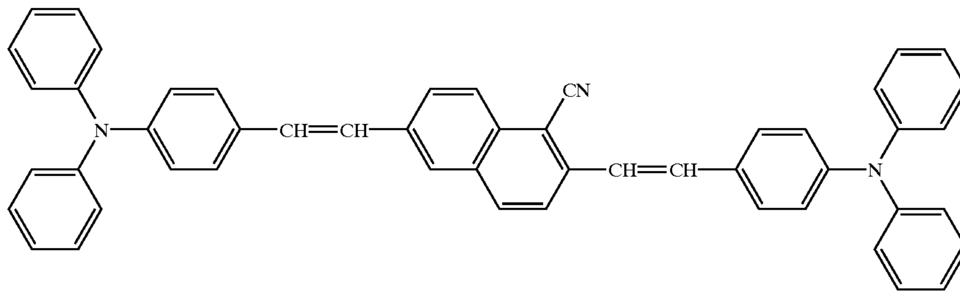
Structural formula (29)-2
