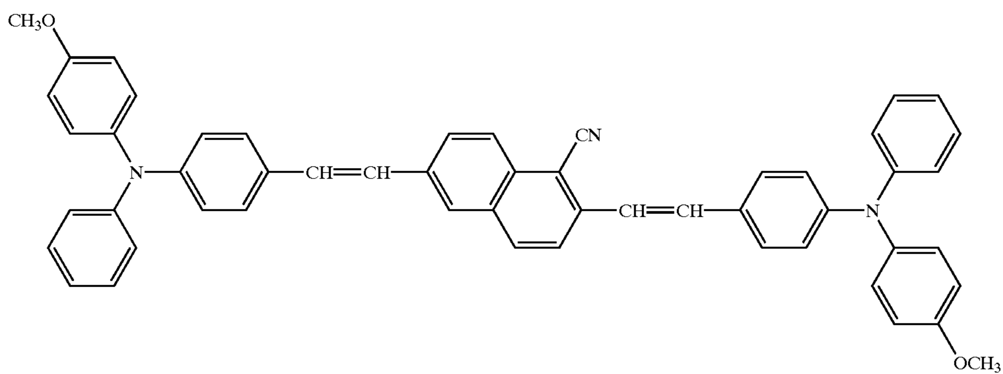
Structural formula (29)-2
