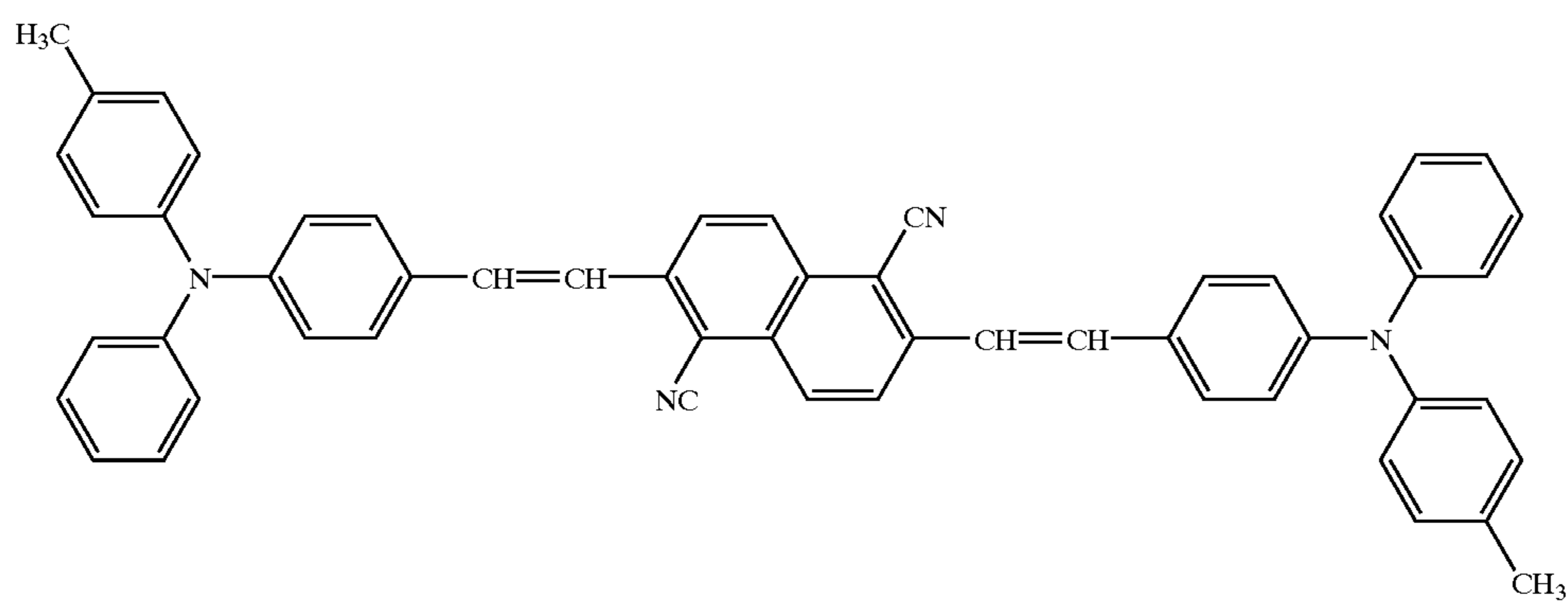
Structural formula (20)-4
