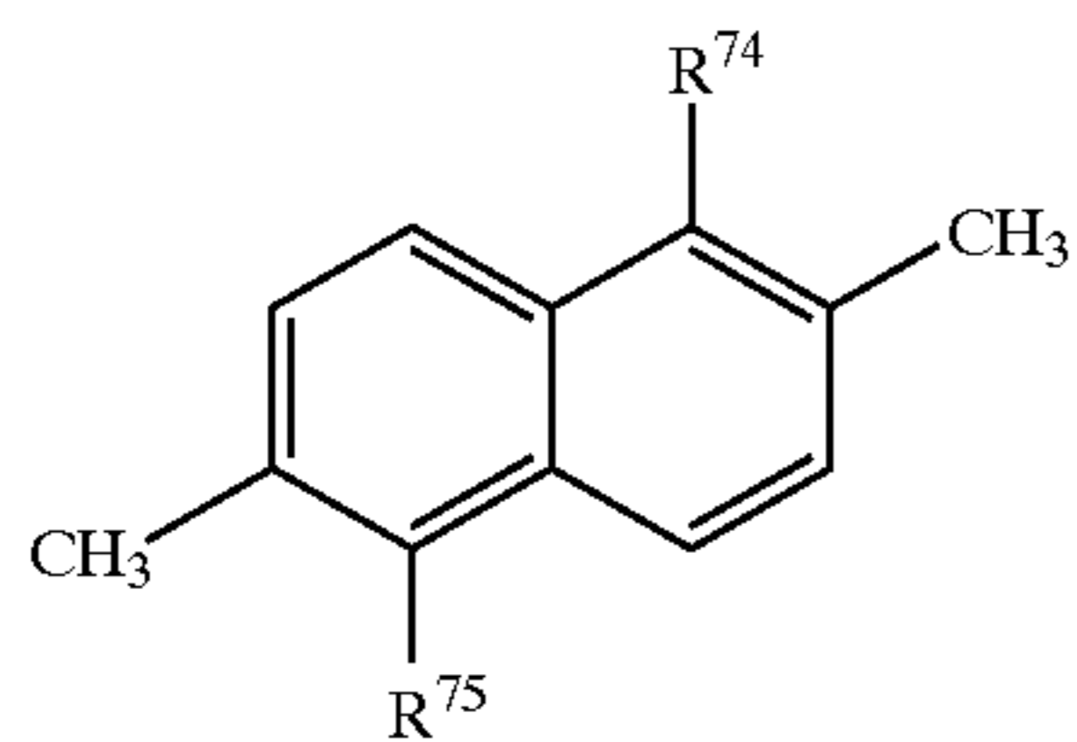
Formula [XII]
