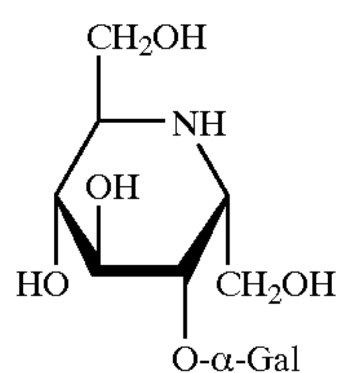
5-O-α-D-Galactopyranosyl-α-homonojirimycin
