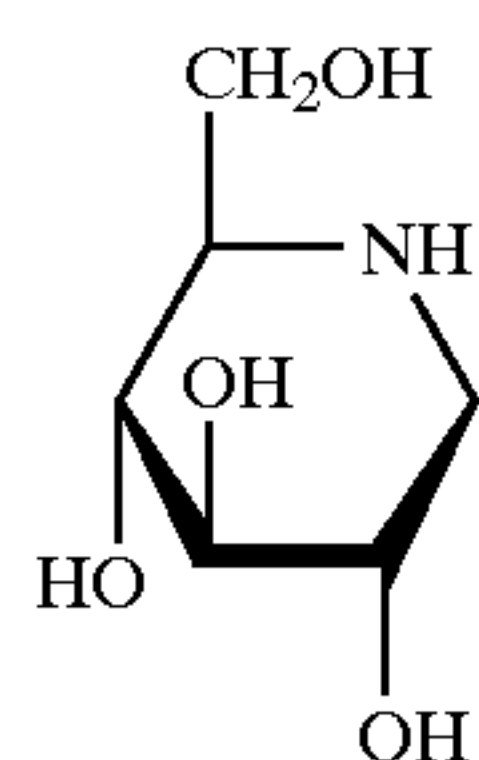
1-Deoxy-nojirimycin
