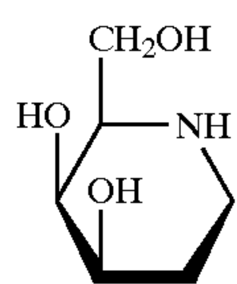
4-epi-fagomine
