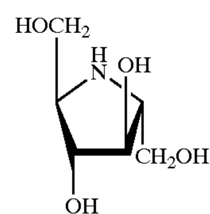
2,5-Dideoxy-2,5-imino-D-mannitol
