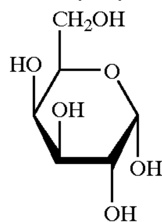
α-D-Galactose
