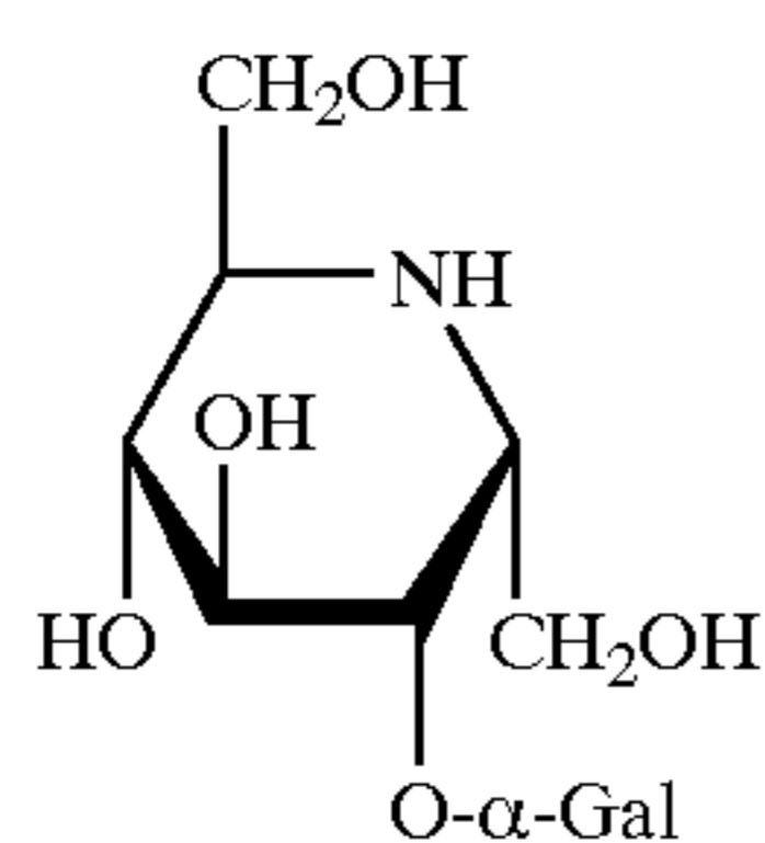
5-O- \alpha -D-Galactopyranosyl- \alpha -homonojirimycin
