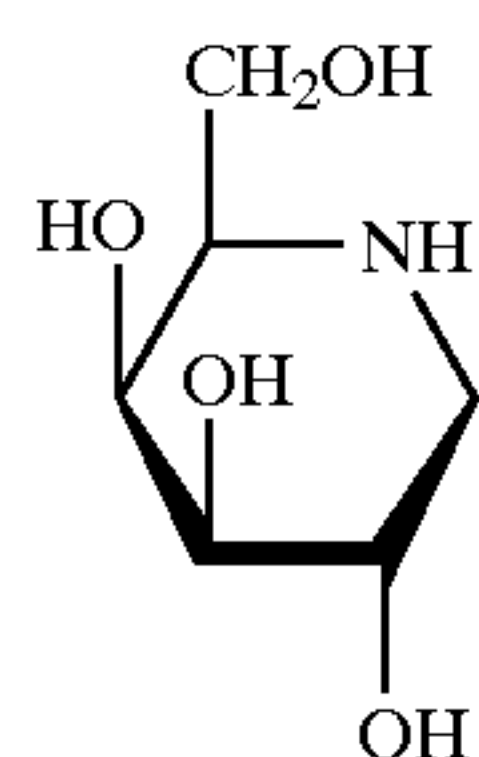
1-Deoxy-Galactonojirimycin
