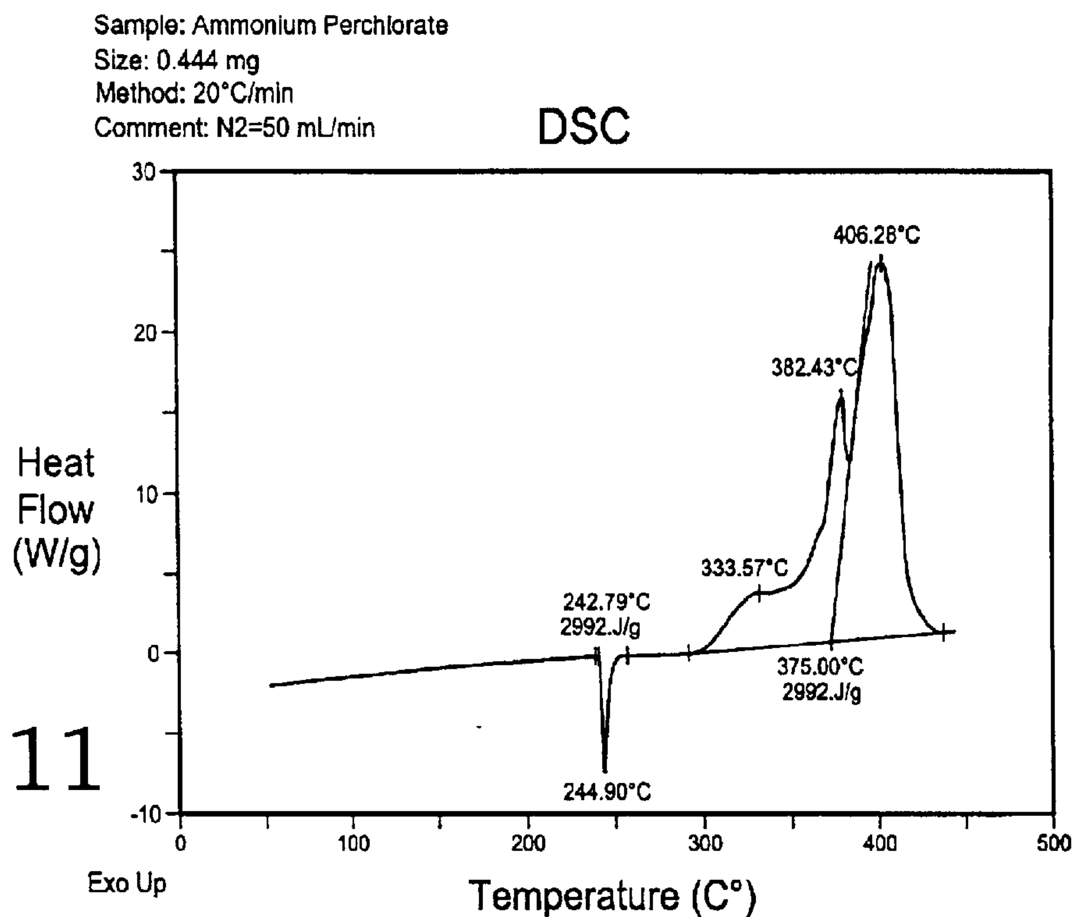
DSC thermogram of Ammonium Perchlorate, sample weight is 0.444 mg
