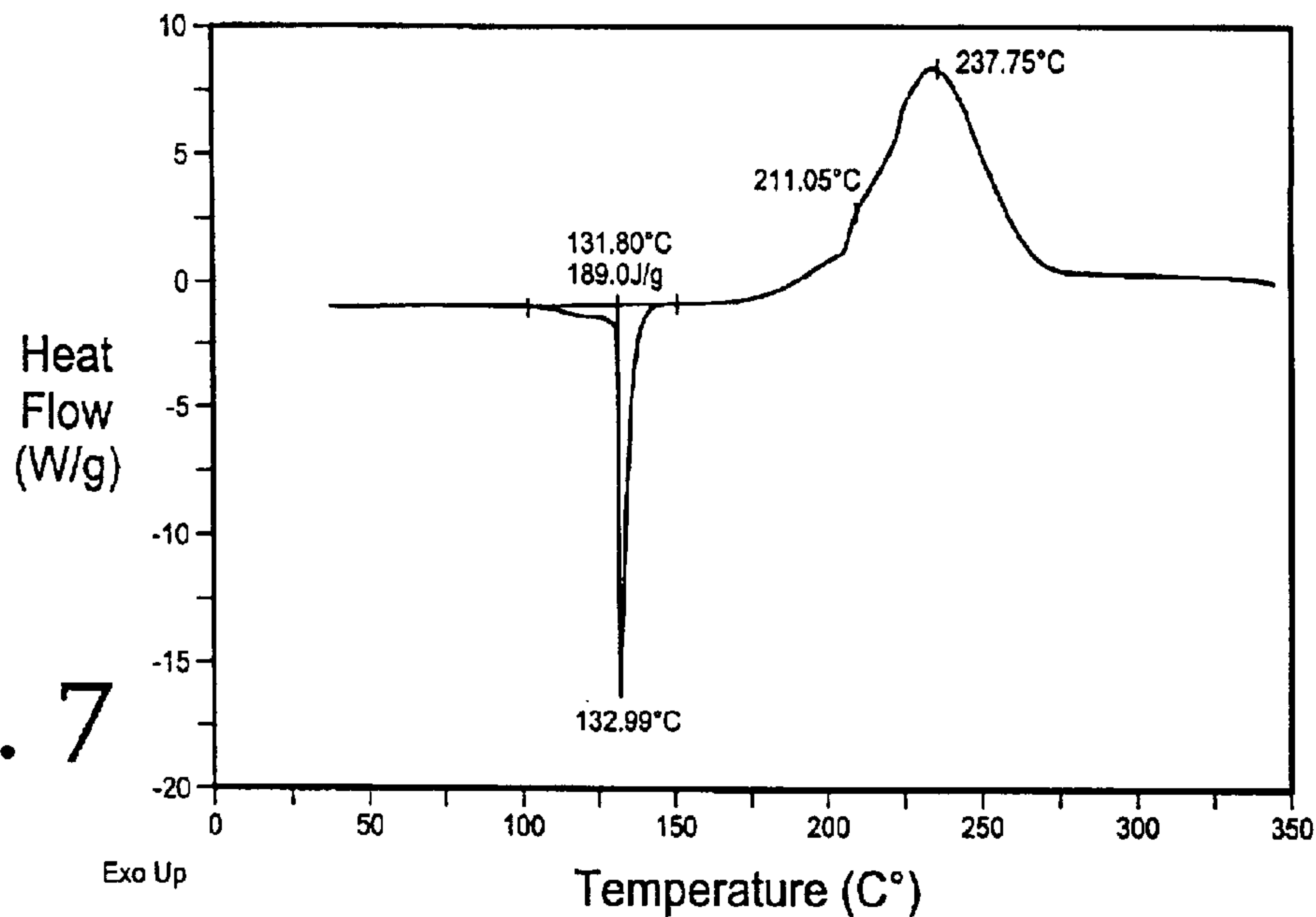
DSC thermogram of DADP, sample weight is 0.699 mg
