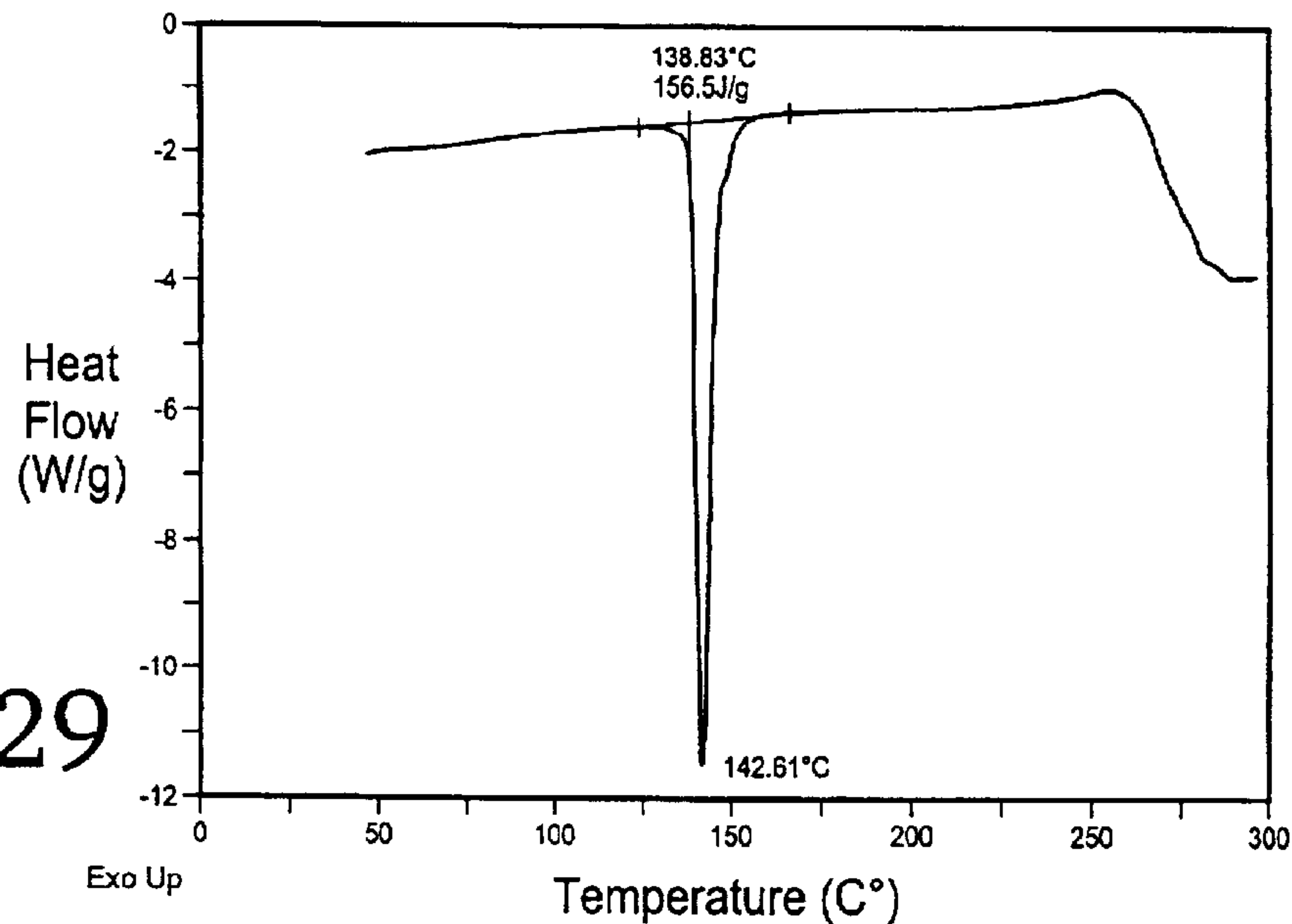
DSC thermogram of Tetracaine, sample weight is 0.581 mg
