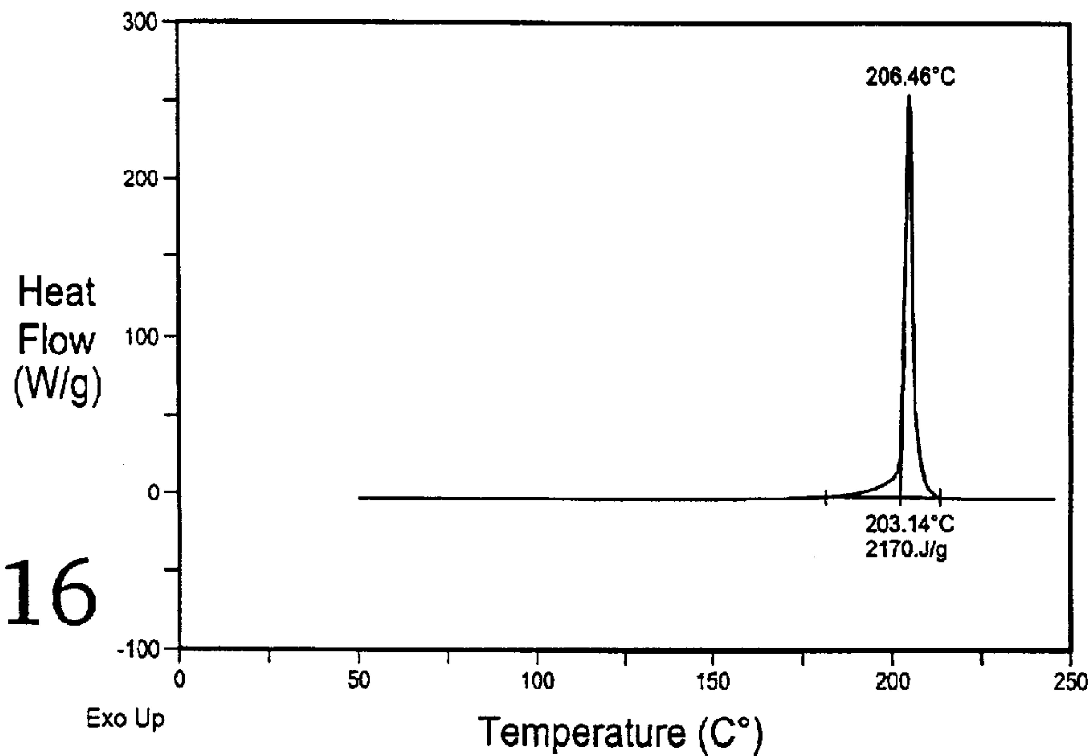
DSC thermogram of Mil. Spec. Ammo., sample weight is 0.215 mg
