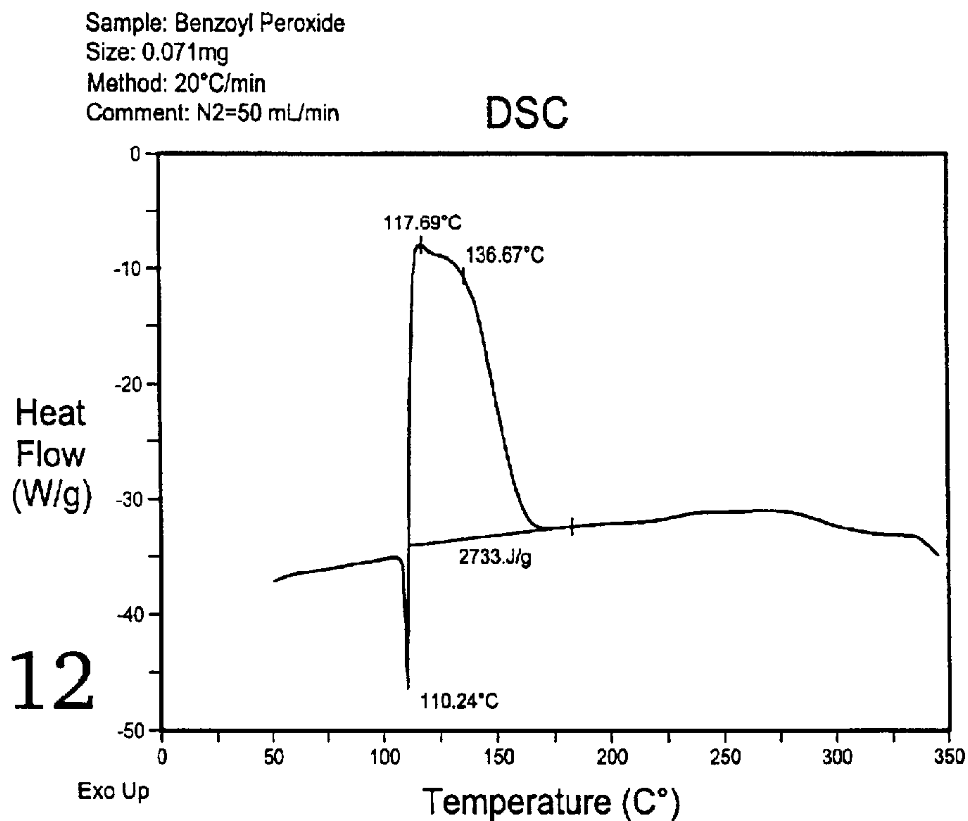
DSC thermogram of Benzoyl Peroxide, sample weight is 0.071 mg
