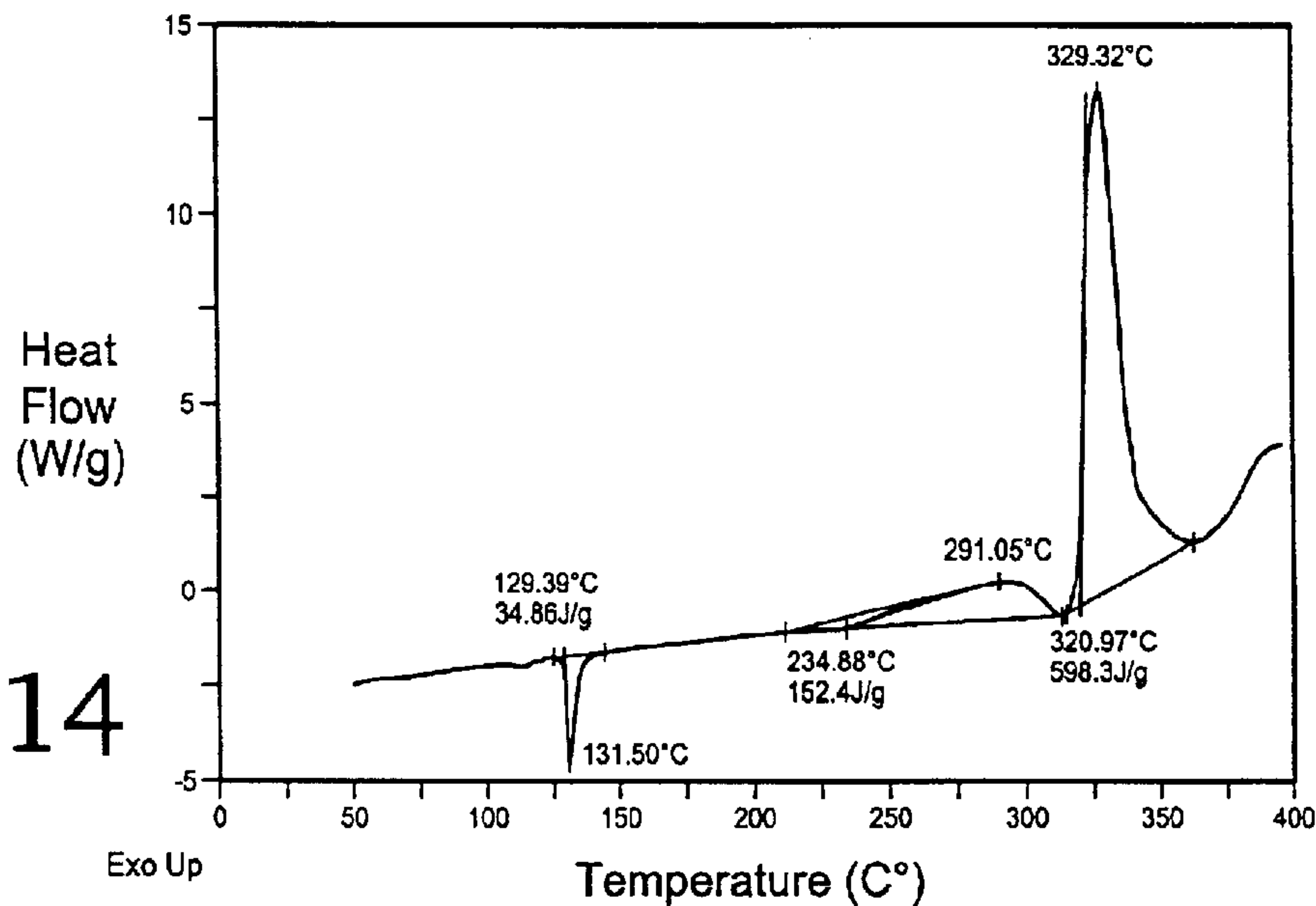
DSC thermogram of Black Powder, sample weight is 0.489 mg
