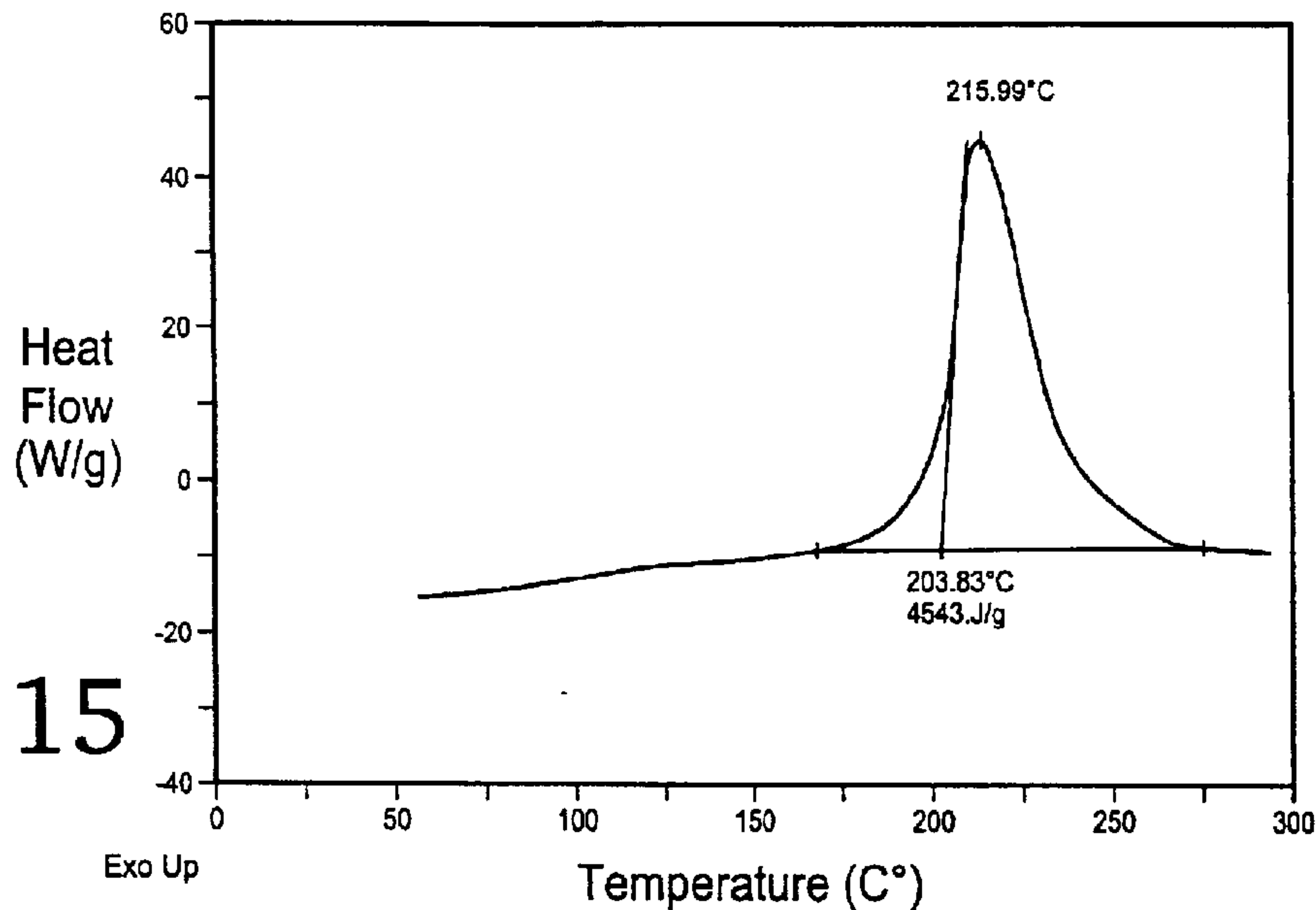
DSC thermogram of Smokeless Remington,, sample weight is 0.071 mg
