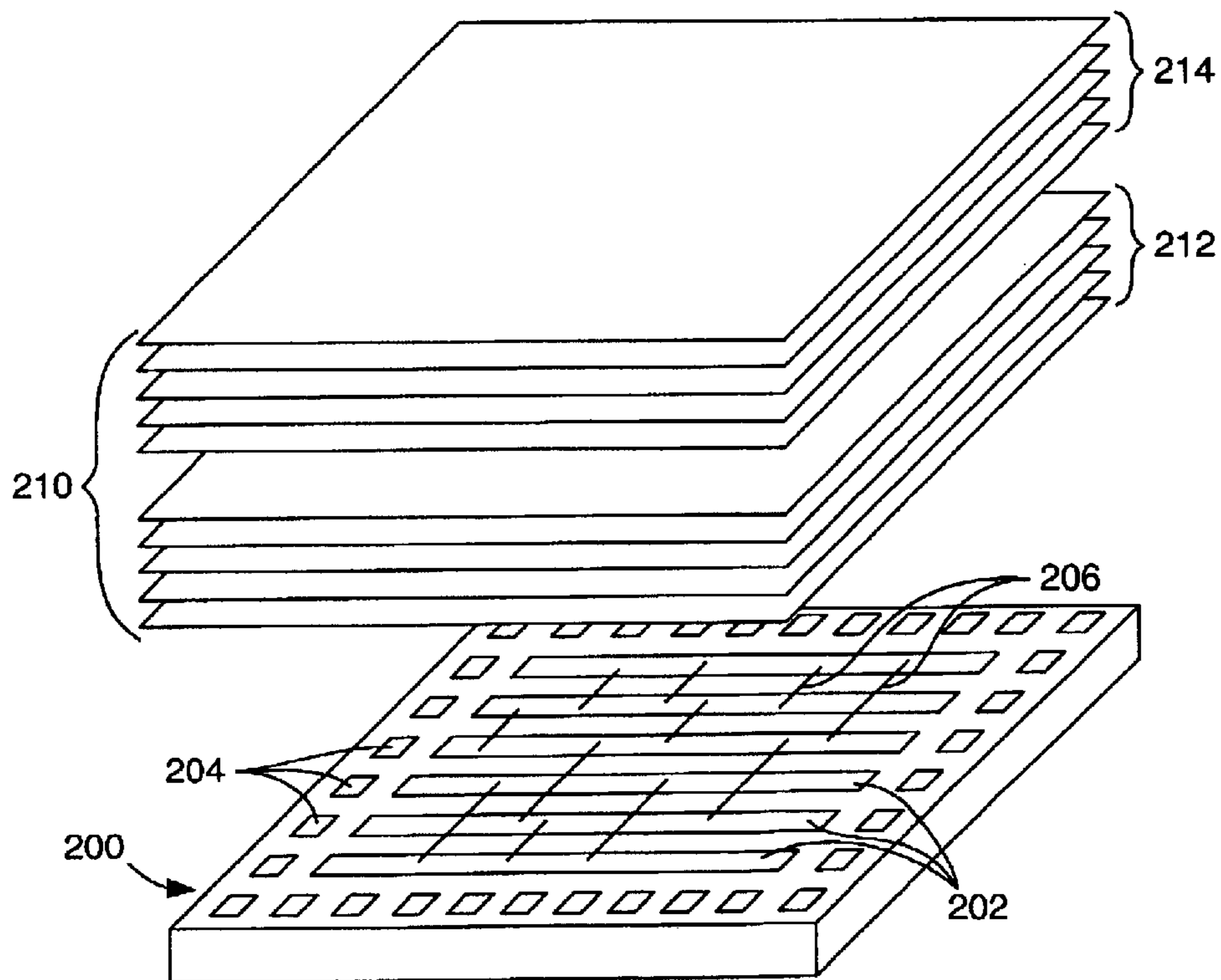
FIG. 2 (PRIOR ART)
