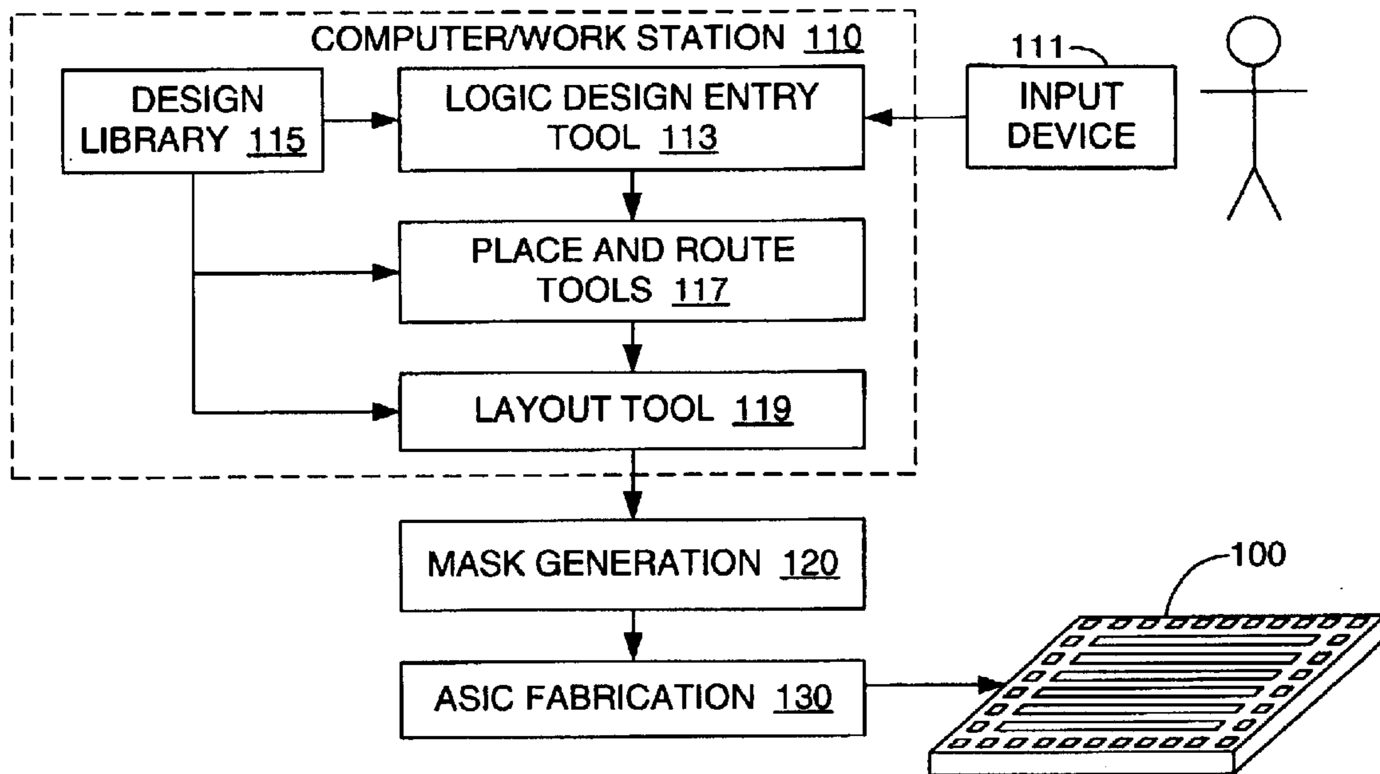
FIG. 1 (PRIOR ART)
