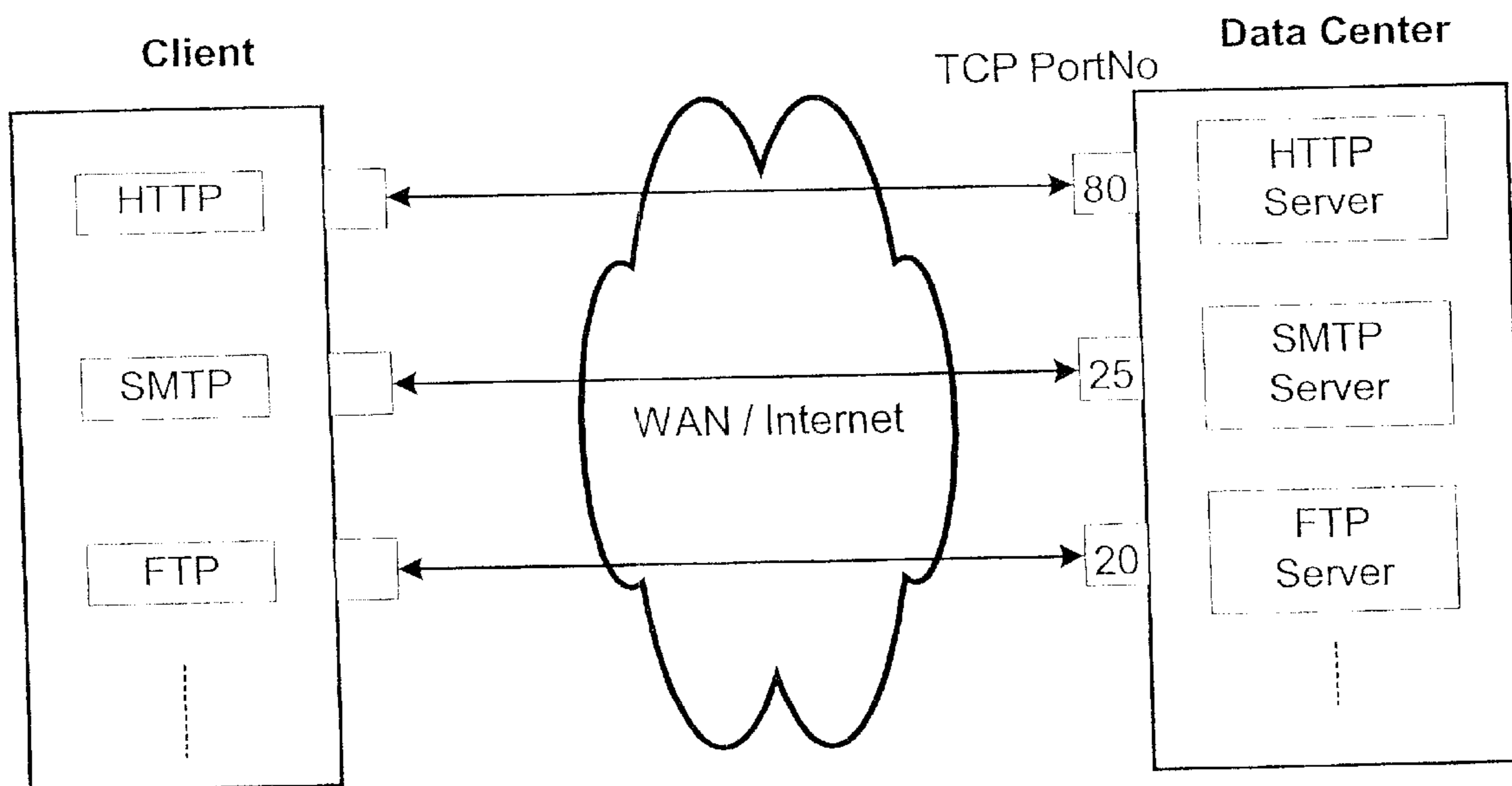
Well-Known TCP port (Softport) Connections
