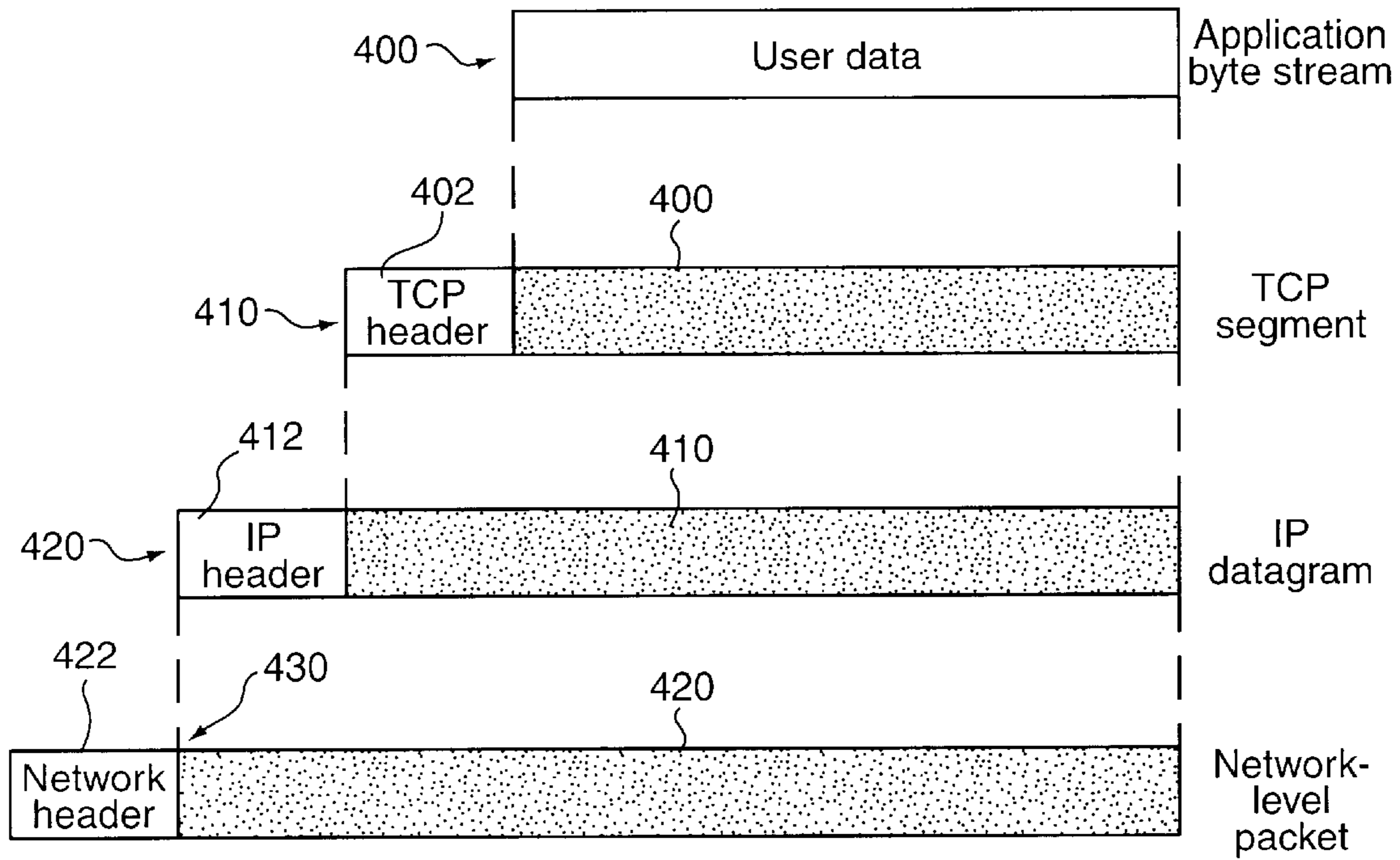
FIGURE 4 (PRIOR ART)
