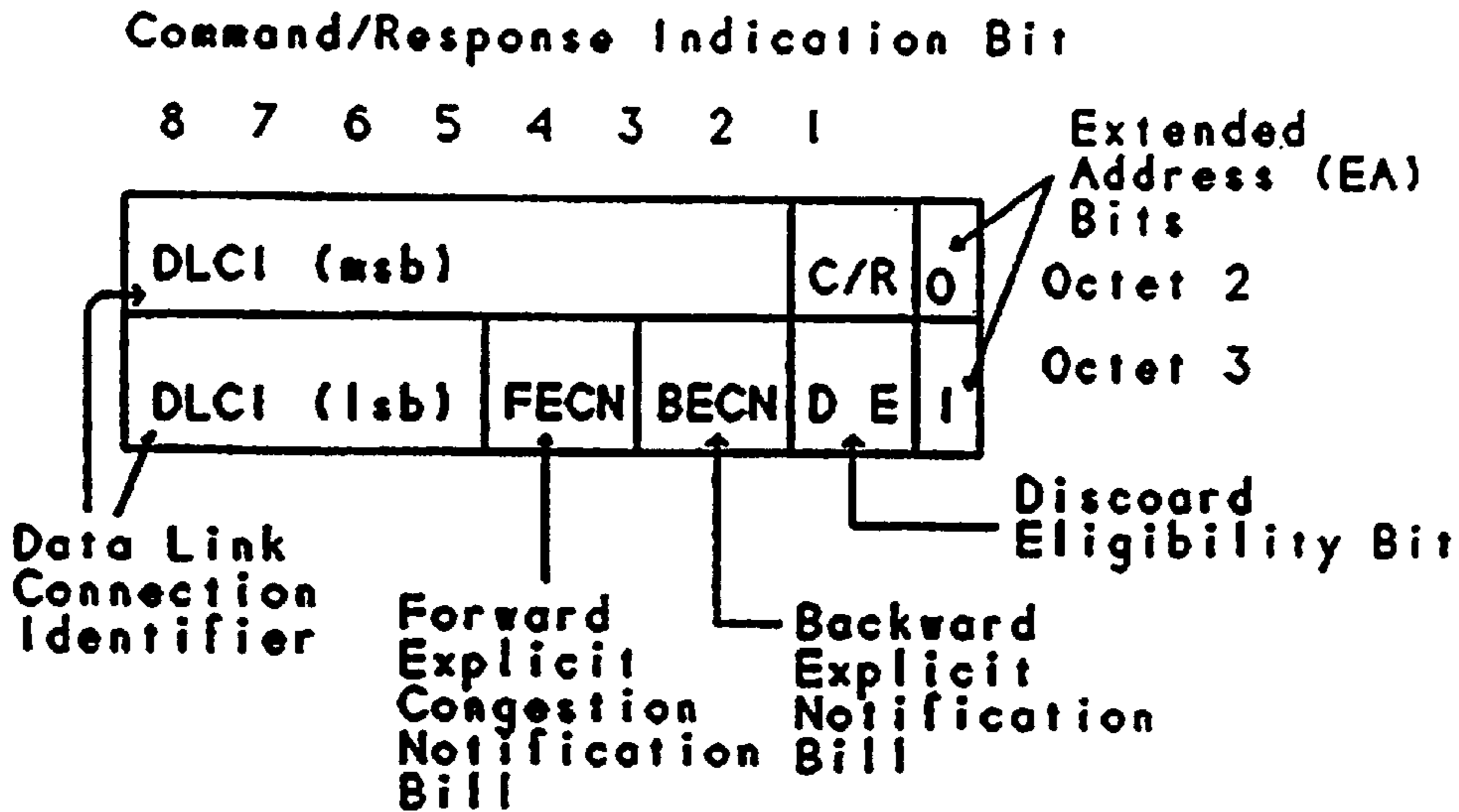
Address Field Format
