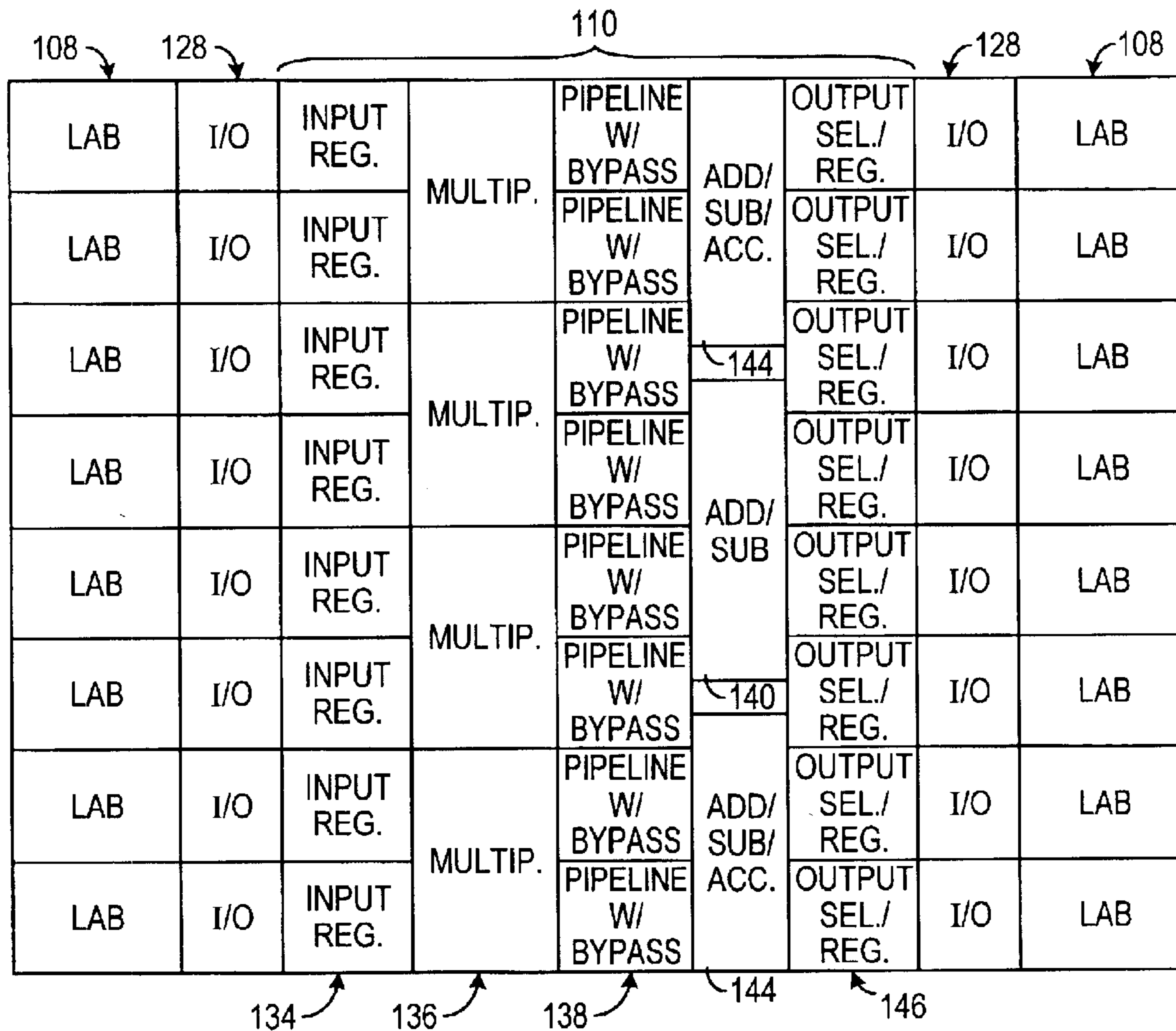
FLOOR PLAN
