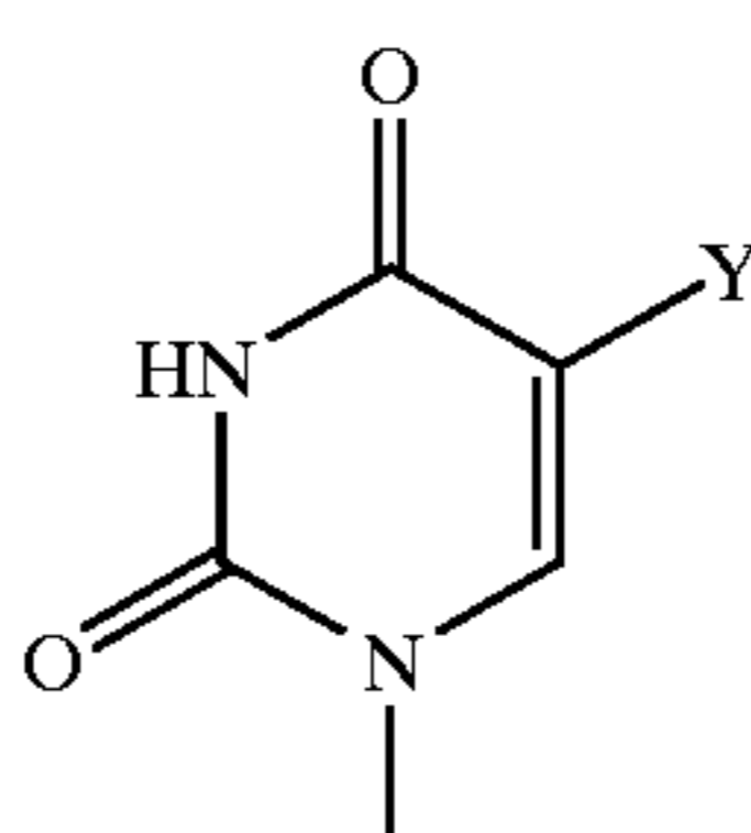
16, Y = Et, Pr, Bu, Pentyl (31)
