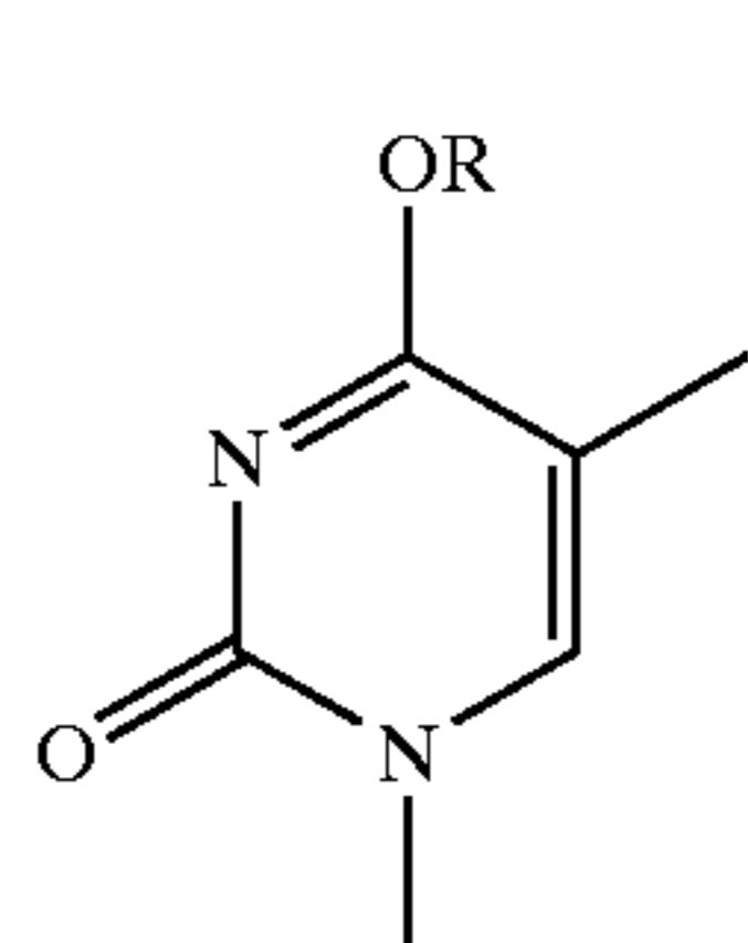
6a, R = Me; 6b, R = Et 6c, R = iPr, 6d, R = nBu (11-15)
