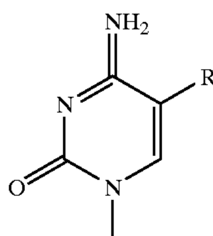
14a, R = Me (24,25) 14b, R = Et (30)
