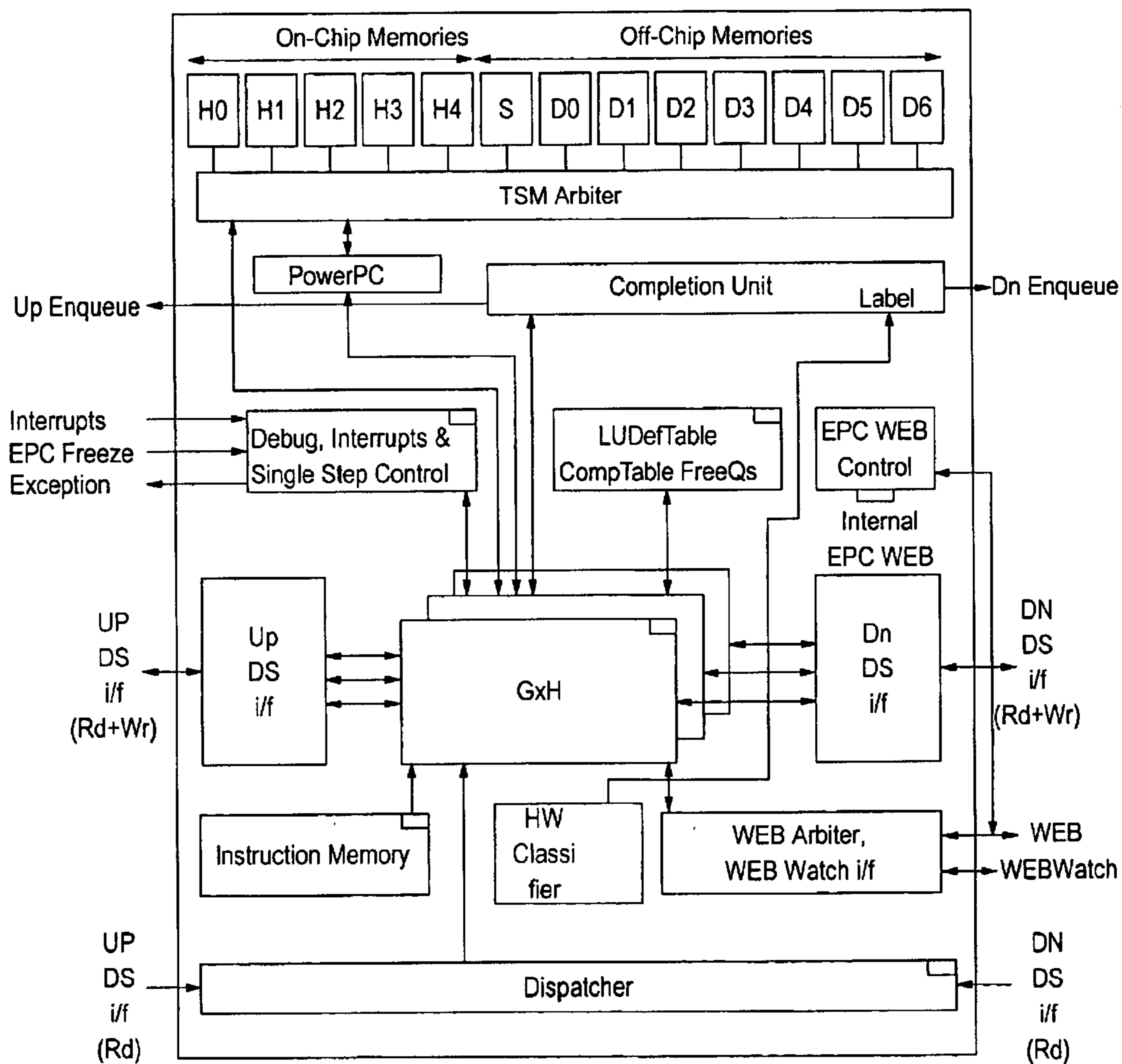
FIG. 12A BLOCK DIAGRAM OF THE EPC
