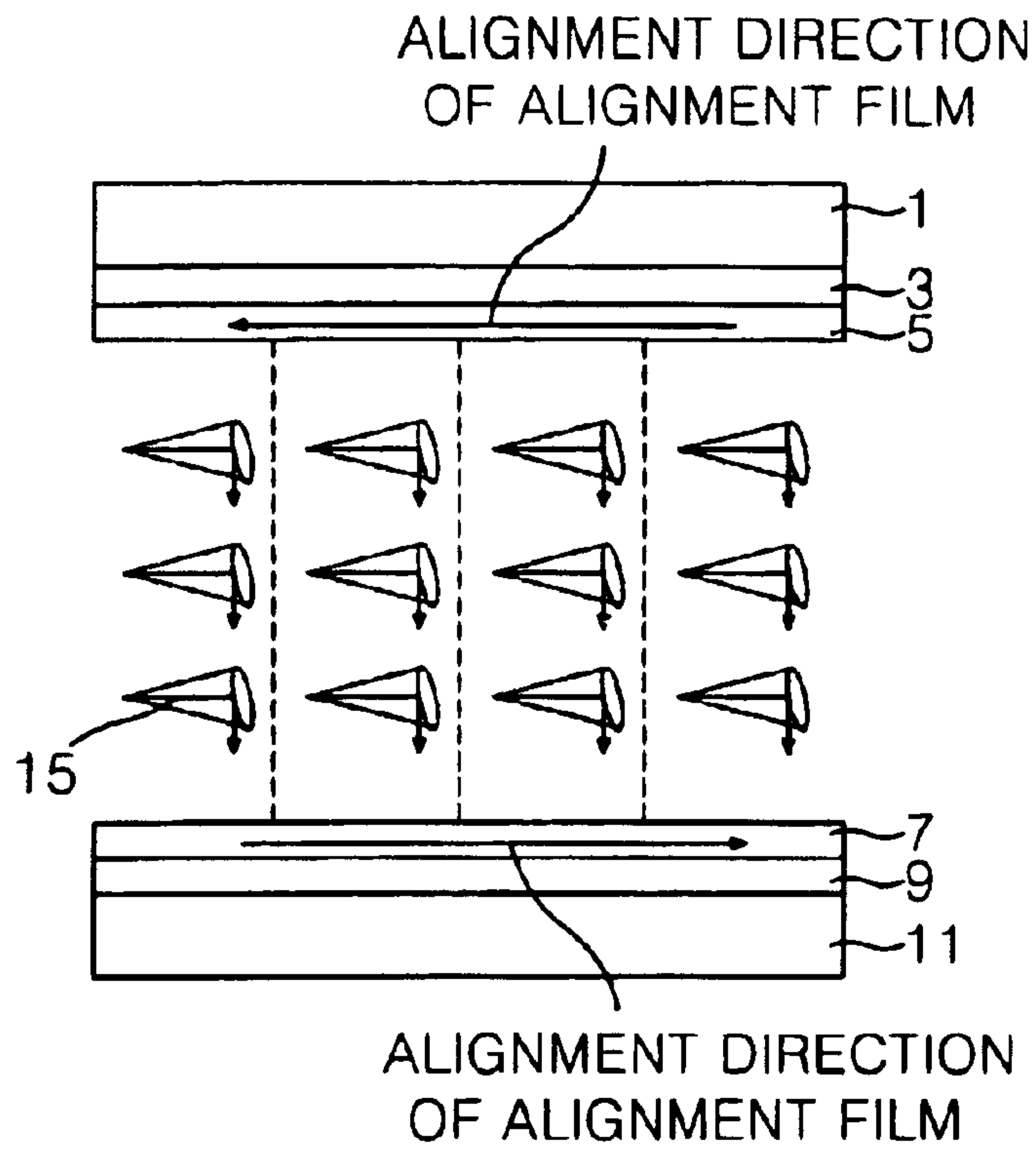
FIG. 3 CONVENTIONAL ART
