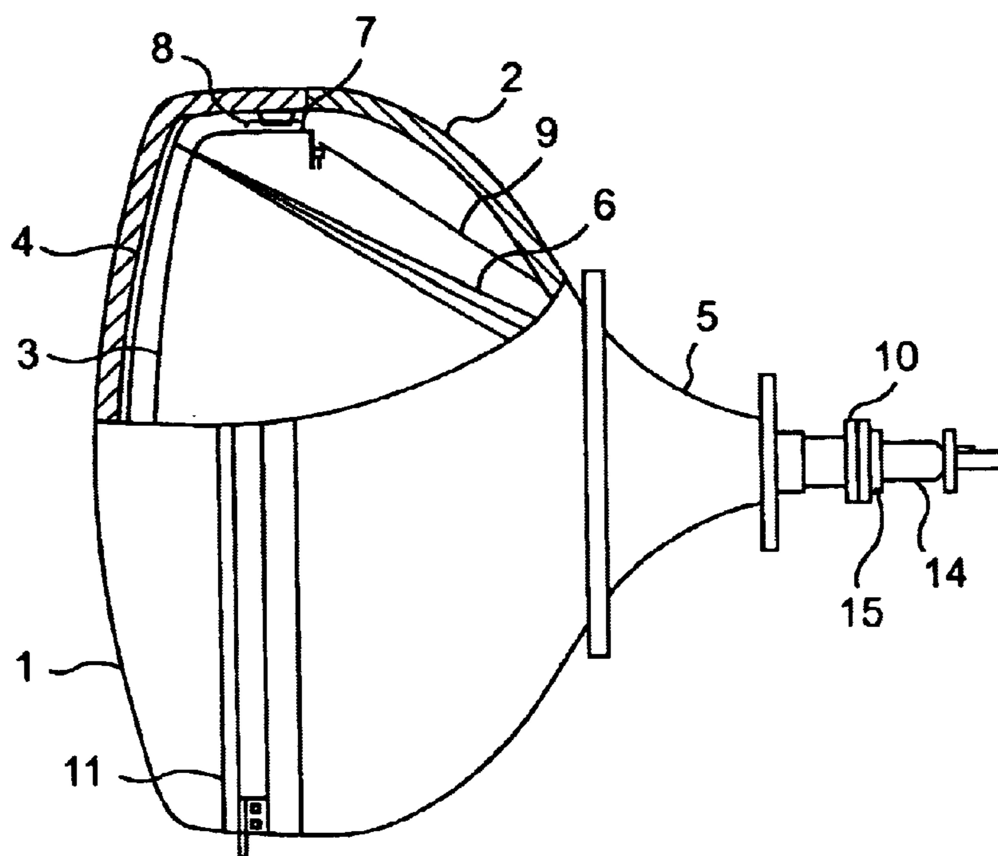
FIG. 1 PRIOR ART
