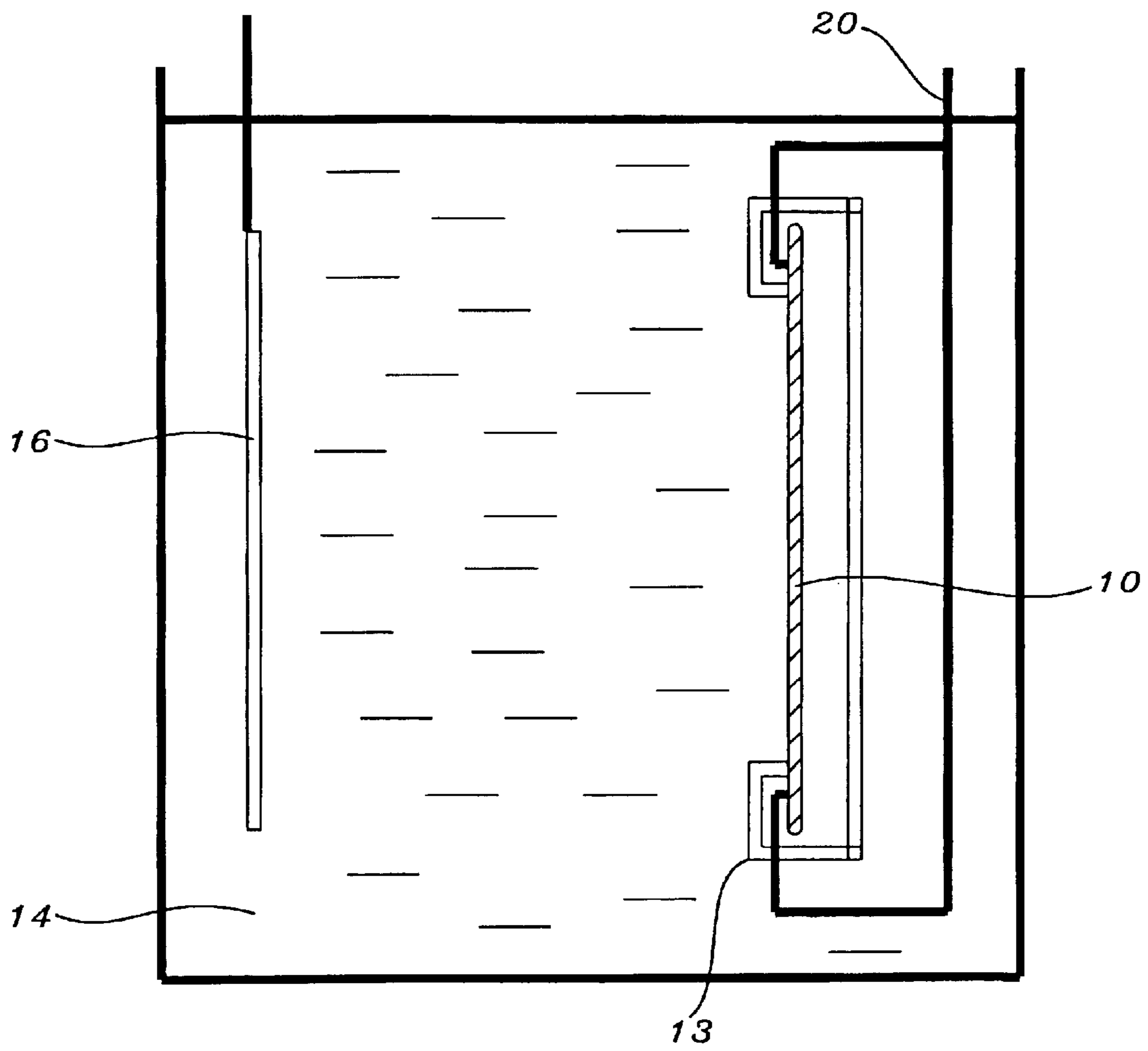
FIG. 3 - Prior Art
