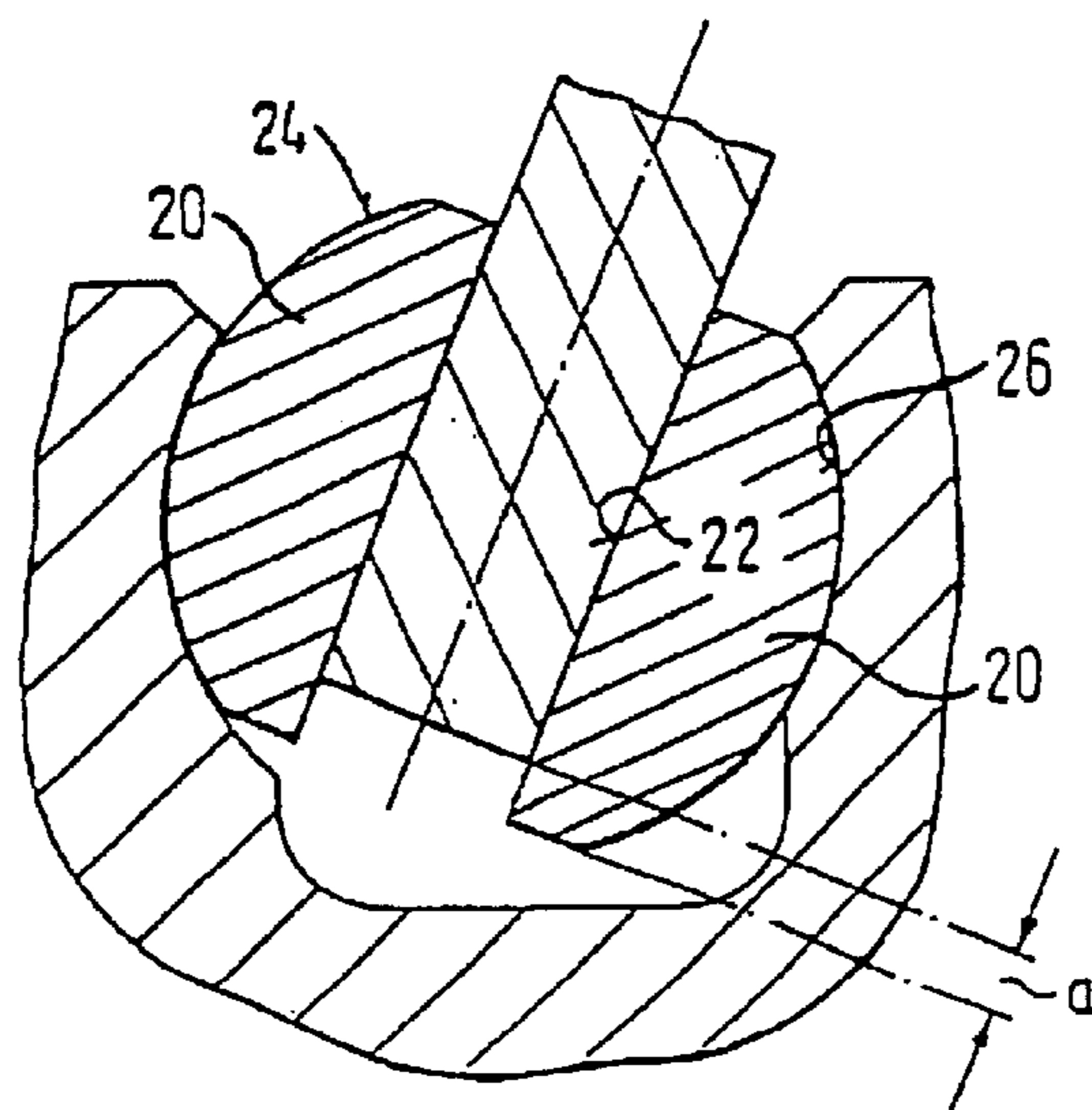
FIG. 2 (Prior Art)
