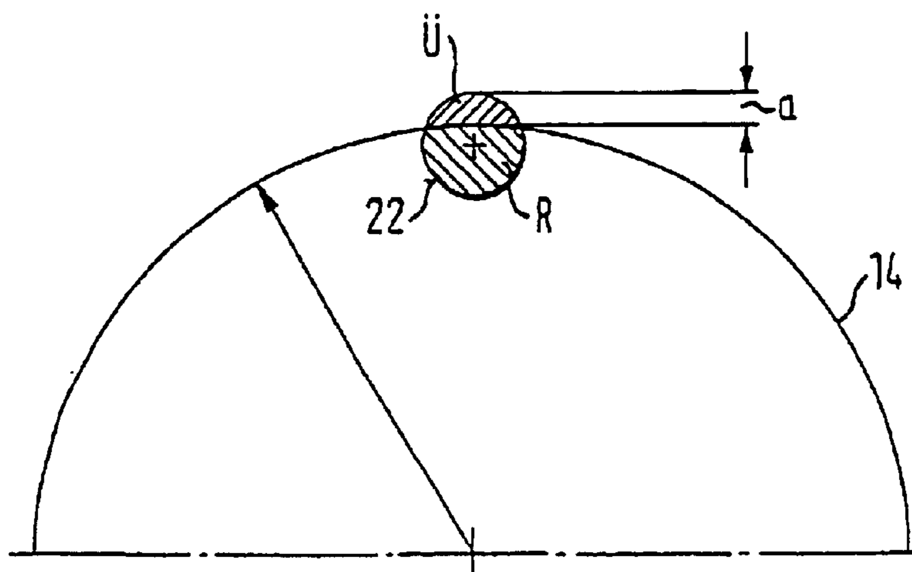
FIG. 5 (Prior Art)
