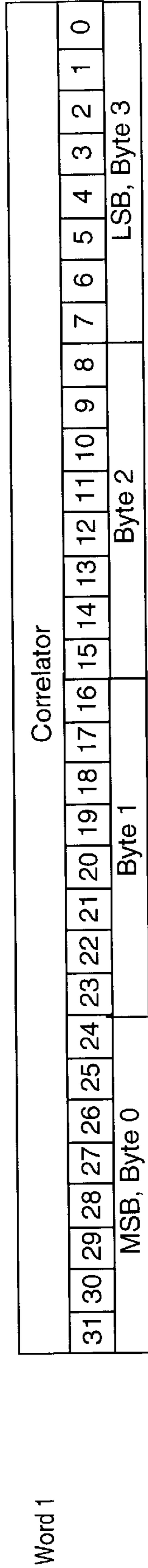
FIG. 7 Correlator
