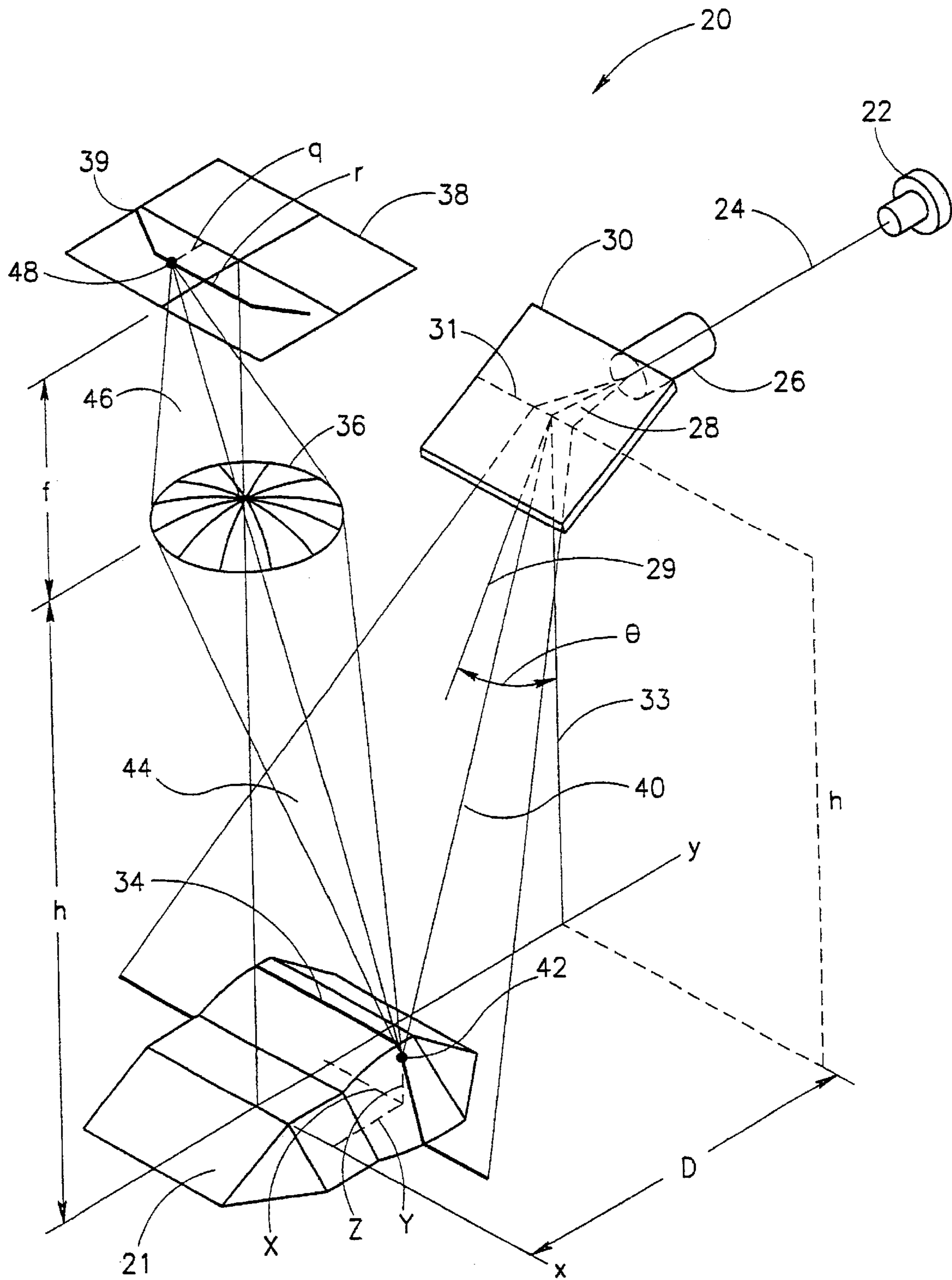
FIG. 1 PRIOR ART
